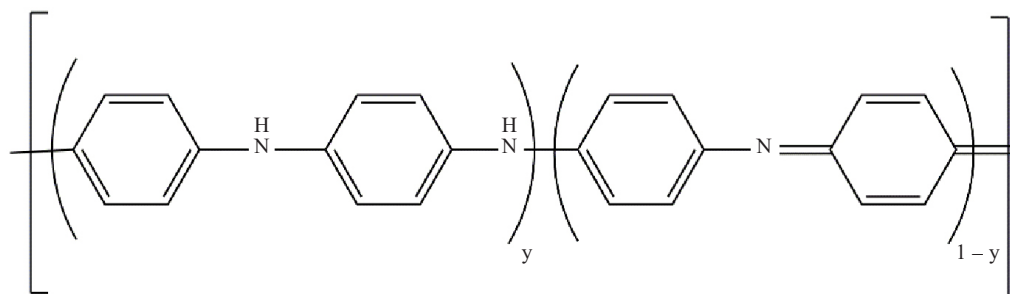
Figure 1. Chemical structure of PANI indicating different oxidation states: fully-reduced leuco-emeraldine (LE) state ( y = 1 ), semi-oxidized emeraldine base (EB) state ( y = 0.5 ) and fully-oxidized pernigraniline (PE) state ( y = 0 ).
