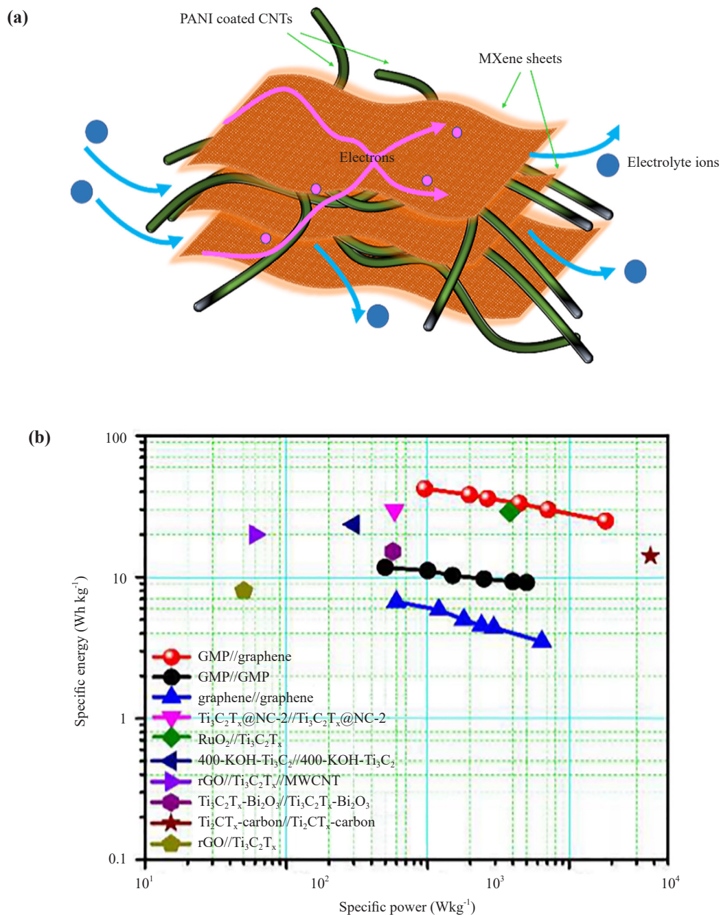
Figure 6. Schematic presentation of the operating charge transport and storage mechanism in MXene-CNT/PANI ternary nanocomposite (a). Ragone plot highlighting the improved electrochemical performances of the Graphene-Encapsulated MXene Ti 3 CT x @PANI (GMP) composite based asymmetric supercapacitor (GMP//graphene) relative to various other composites already reported in the literature (b). Reproduced on permission from ref. [100], copyright 2018, ACS publications
