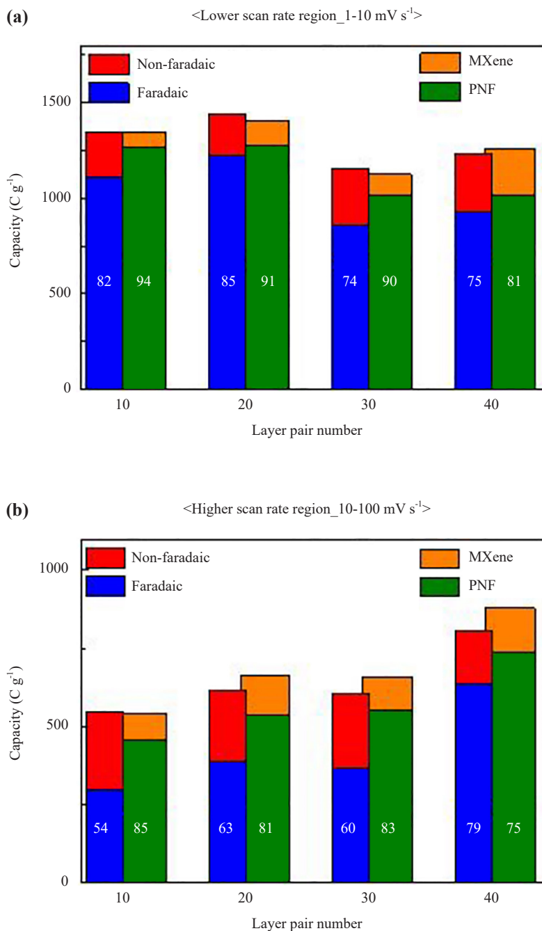
Figure 5. Relative contributions from non-Faradaic (red) and Faradaic (blue) processes bar from MXenes (orange) and PNFs (olive) as a function of the number of layer pair numbers (a) at the slower potential scan rate regime (1-10 mVs -1 ) and (b) at the higher potential scan rate regime (10-100 mVs -1 ). Reproduced on permission from ref. [96] ACS publications.
