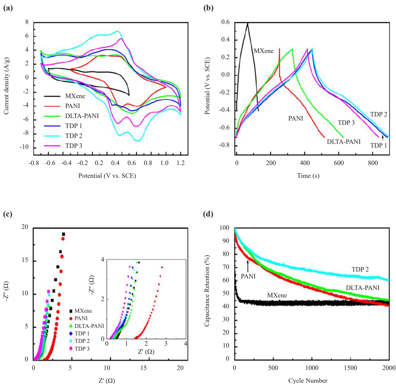
Figure 4. Comparative cyclic voltammograms of pristine-MXene, pure-PANI, DLTA-PANI and MXene-DLTA/PANI (TDPs) sample electrodes at a voltage sweep rate of 10 mVs -1 (a), Comparative galvanostatic charging/discharging profiles of pristine-MXene, pure-PANI, DLTA-PANI and MXene-DLTA/PANI (TDPs) electrodes at a current density of 1 Ag -1 (b), Nyquist plots of pristine-MXene, pure-PANI, DLTA-PANI and MXene-DLTA/PANI (TDPs) samples (c) and Comparative capacitance retention efficacy of pristine-MXene, pure-PANI, DLTA-PANI and optimized-MXene-DLTA/PANI (TDP2) sample electrode at a constant current density of 4 Ag -1 for 2000 cycles (d). Reproduced on permission form ref. [88], copyright 2020, ACS publications
