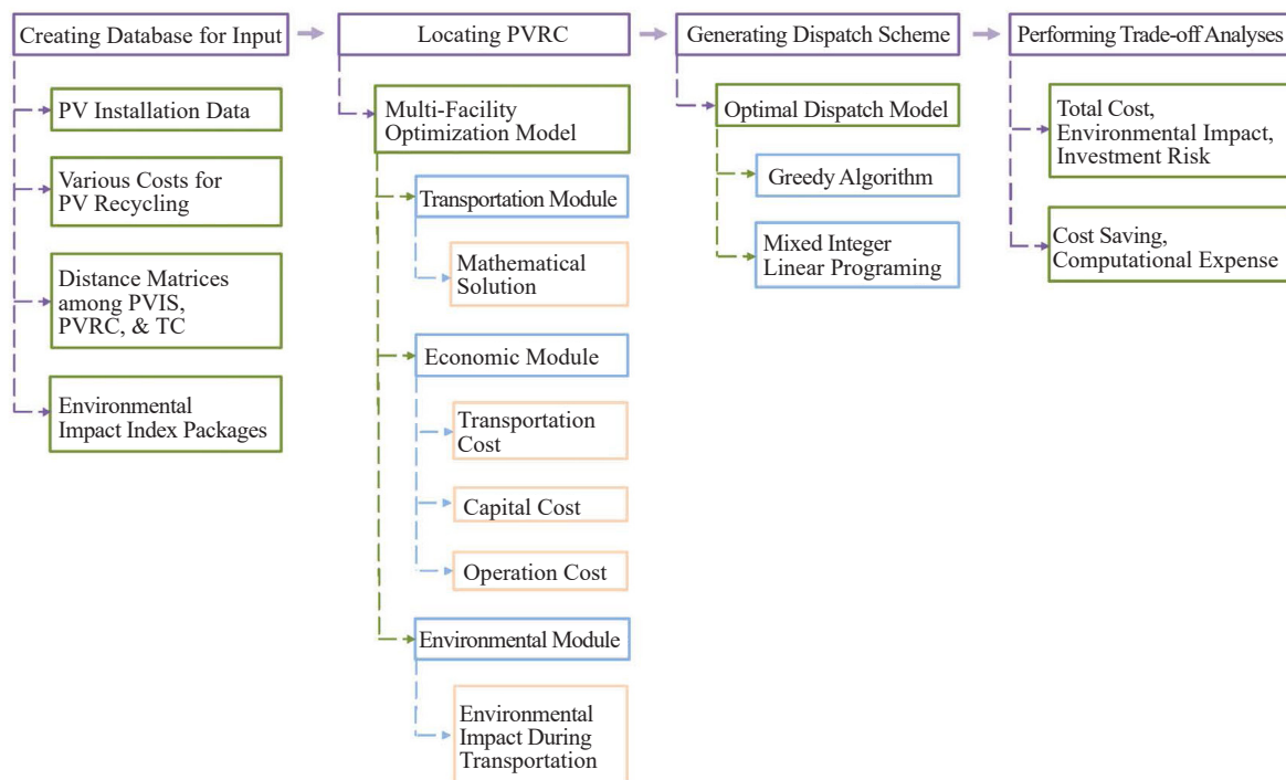
Figure 1. Structure of PV recycling network
