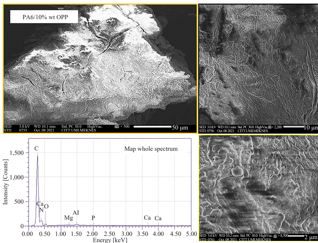
Figure 6. SEM image of the surface of a PA6/OPP pellet without contact with bacteria
