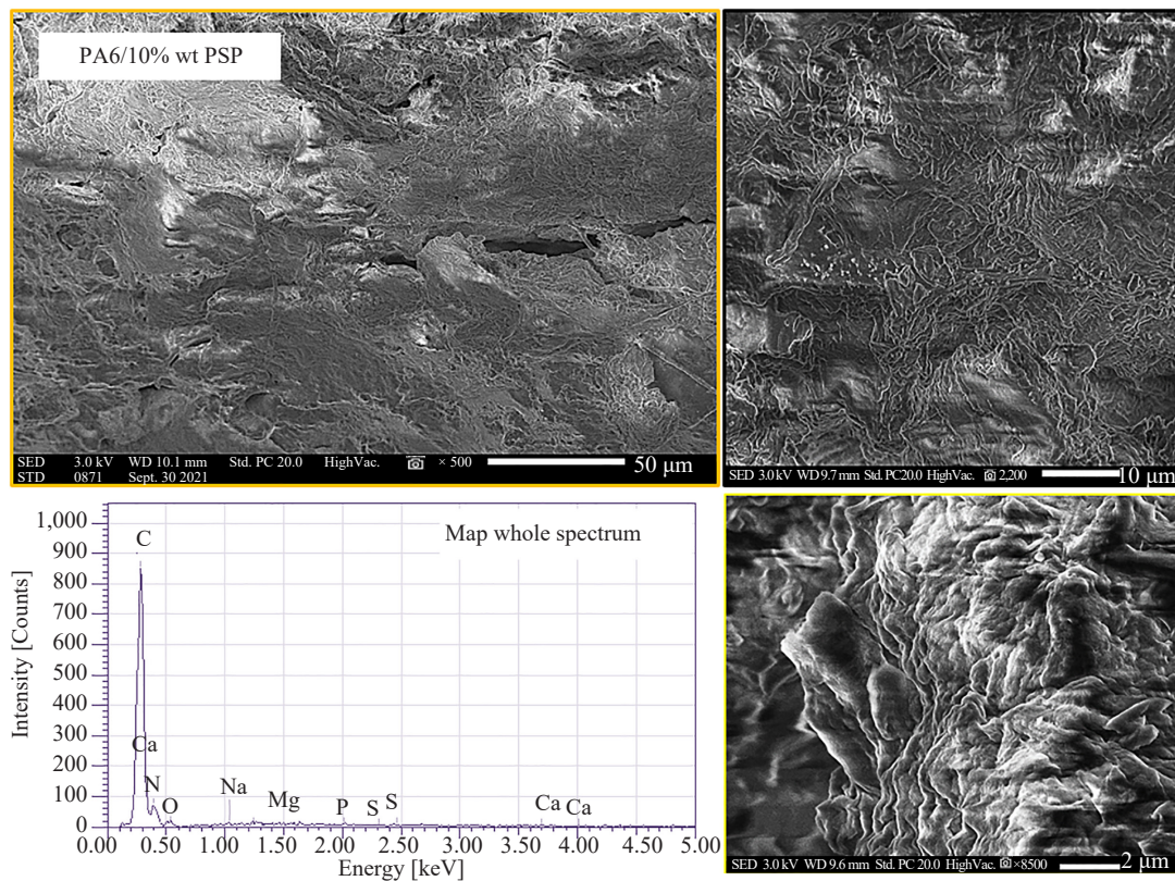
Figure 12. SEM image of PA6/PSP composite without contact with bacteria
