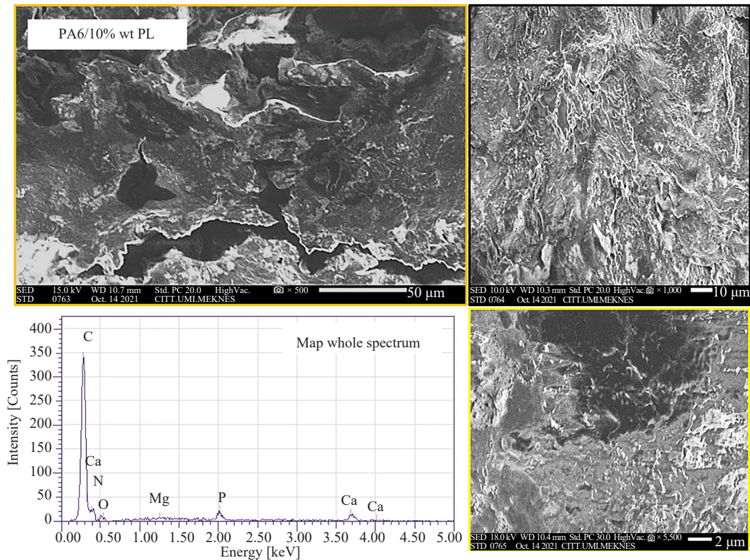
Figure 9. SEM-EDX of the surface of a PA6/PL without contact by bacteria
