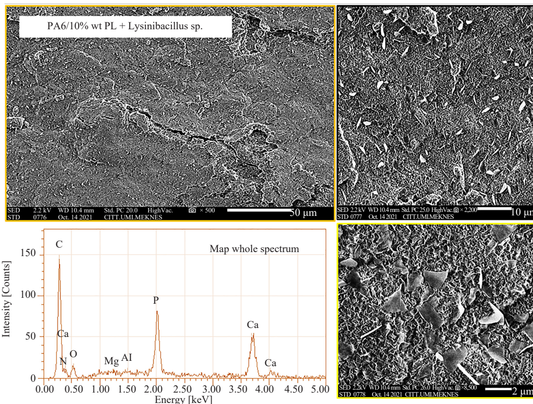
Figure 10. SEM-EDX of the surface of a PA6/PL in contact with Lysinibacillus sp.
