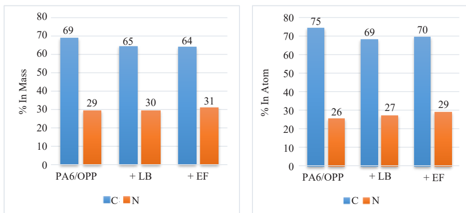
Figure 15. Evolution of the chemical composition by mass of the PA6/OPP composite without and in contact with bacteria: Lysinibacillus (LB) and Enterococcus faecalis (EF)
