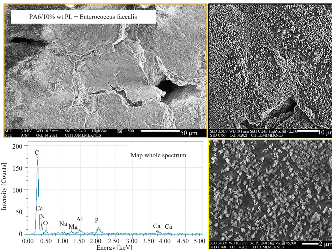
Figure 11. SEM-EDX of the surface of a PA6/PL in contact with Enterococcus faecalis
