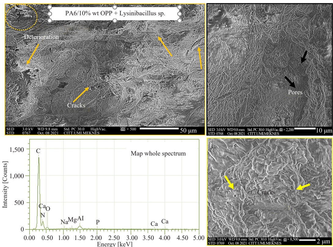
Figure 7. SEM-EDX of the surface of a PA6/OPP contact with Lysinibacillus sp.
