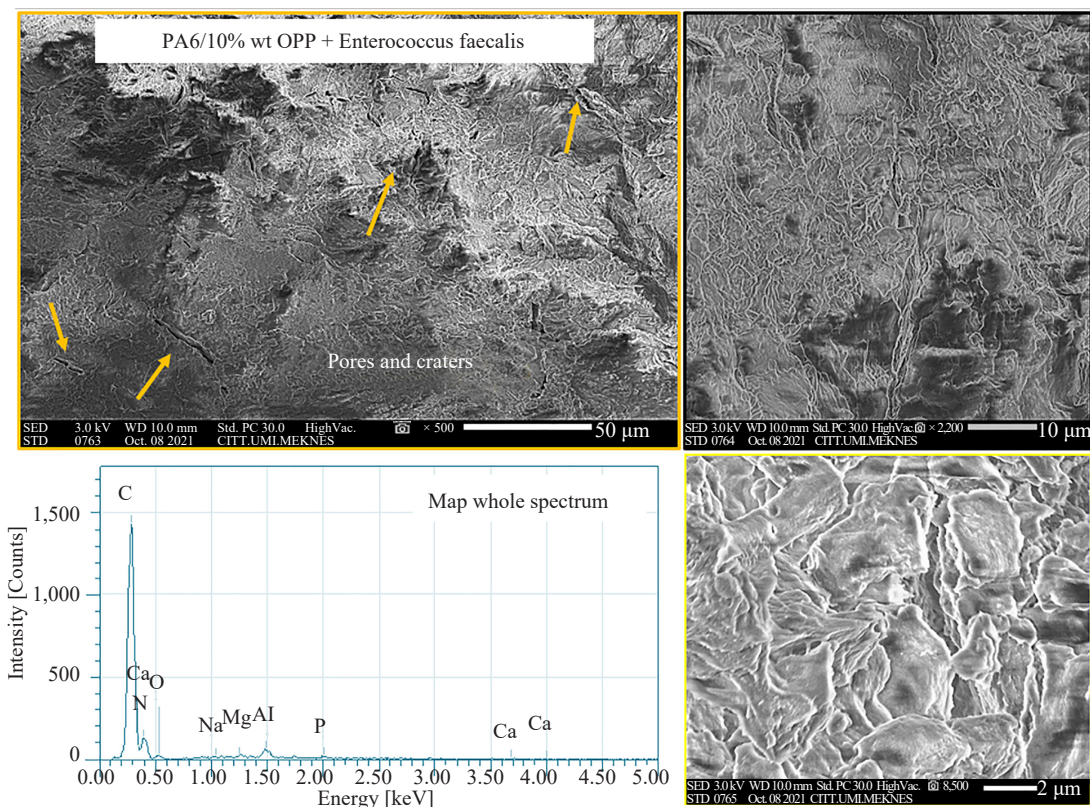
Figure 8. SEM image of the surface of a PA6/OPP in contact with Enterococcus faecalis
