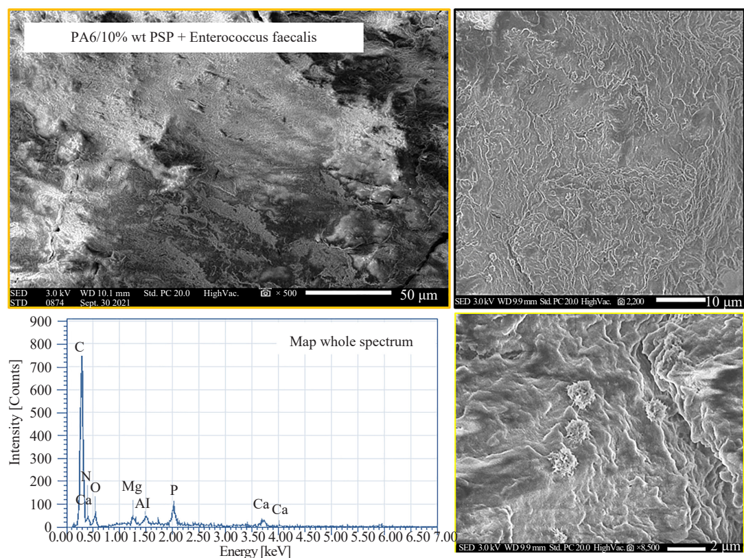
Figure 14. SEM image of the PA6/PSP composite in contact with Enterococcus faecalis bacteria
