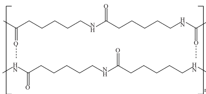
Figure 1. Hydrogen bonding between molecular chains of PA6
