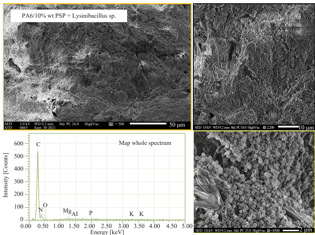
Figure 13. SEM image of the PA6/PSP composite in contact with Lysinibacillus sp.
