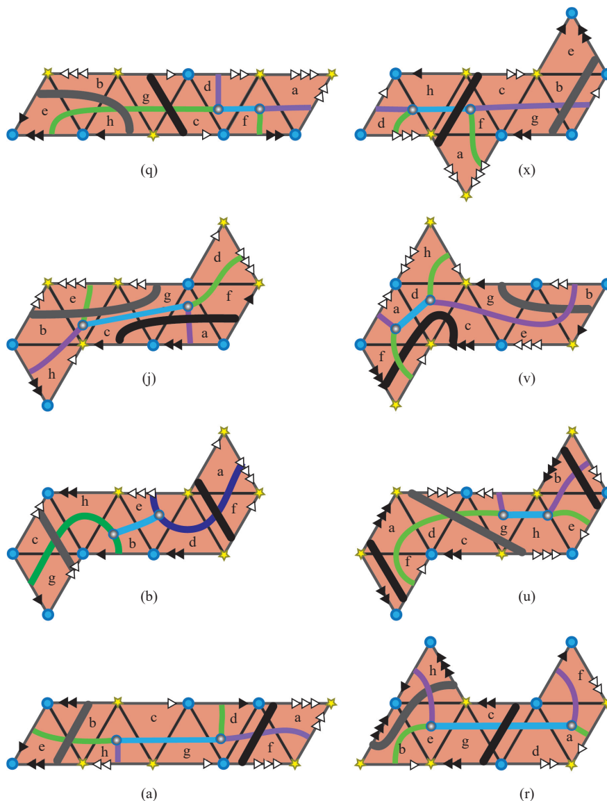
Figure 8. Theta graphs and attaching circles of the 2-handles embedded in the boundaries surfaces of the eight Fujii's manifolds
