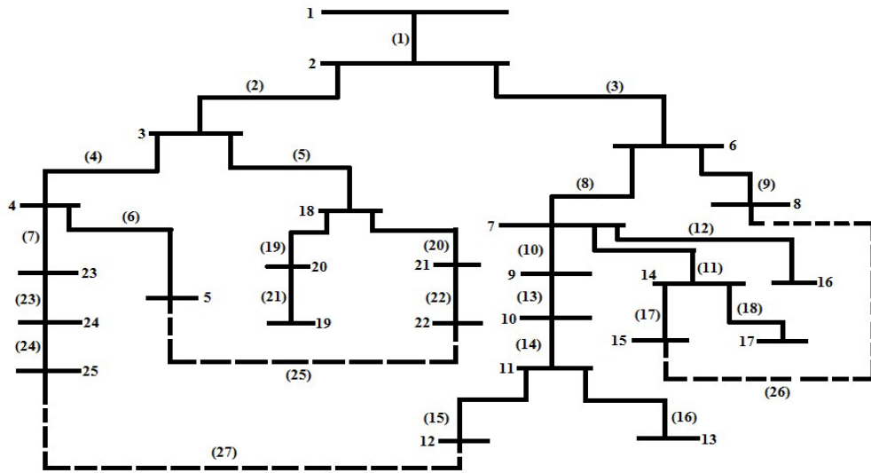
Figure 7: A 25-node Unbalanced Radial Distribution System.
