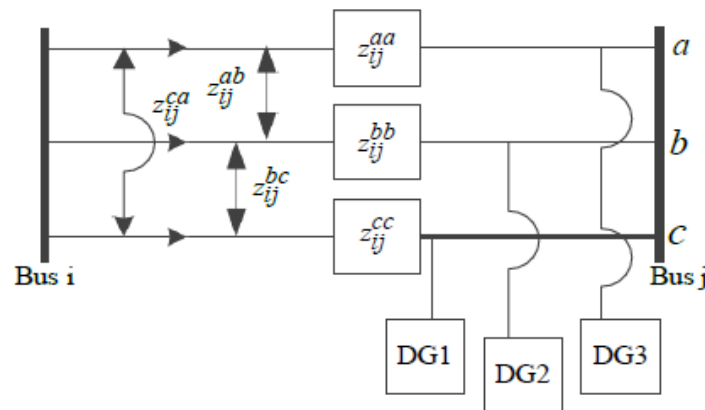
Figure 3: Connection diagram of DGs in a sample unbalanced distribution system.
