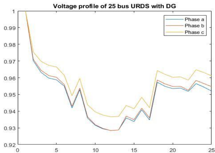
Figure 9: A 125-node URDS voltage profile with DG.
