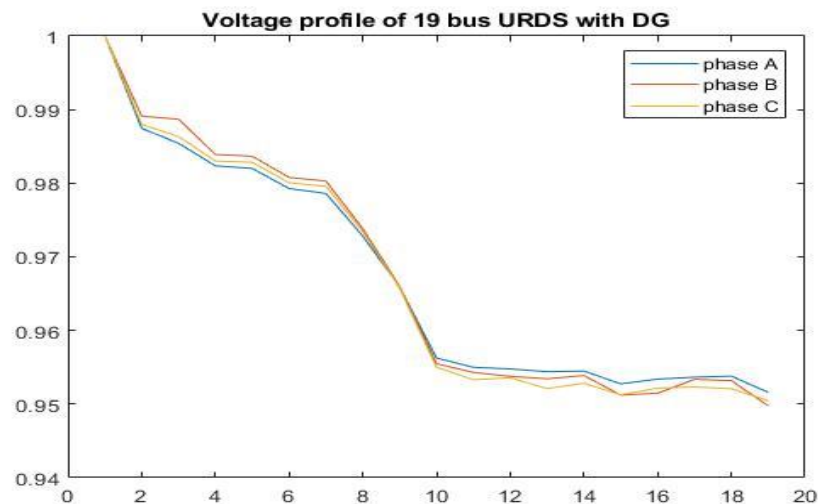
Figure 6: 19-node unbalanced radial distribution system voltage profile with DG
