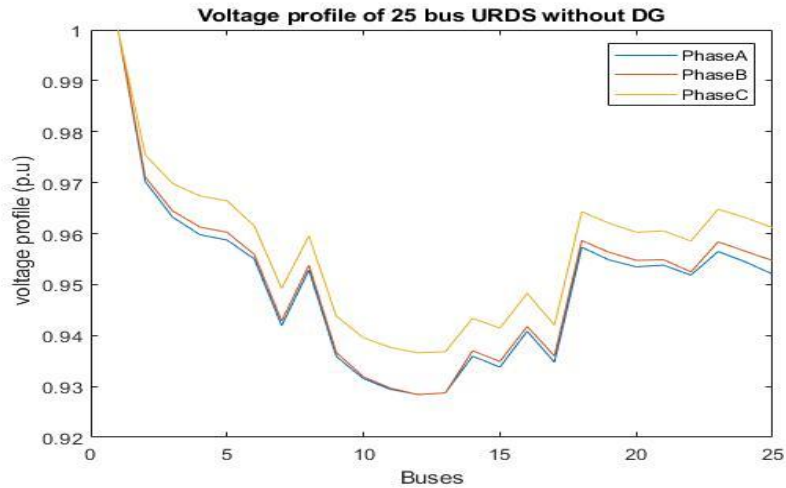
Figure 8: A 25-node unbalanced radial distribution system voltage profile without DG.
