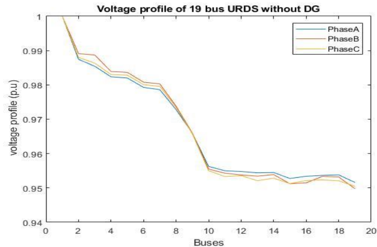
Figure 5: 19- node without DG
