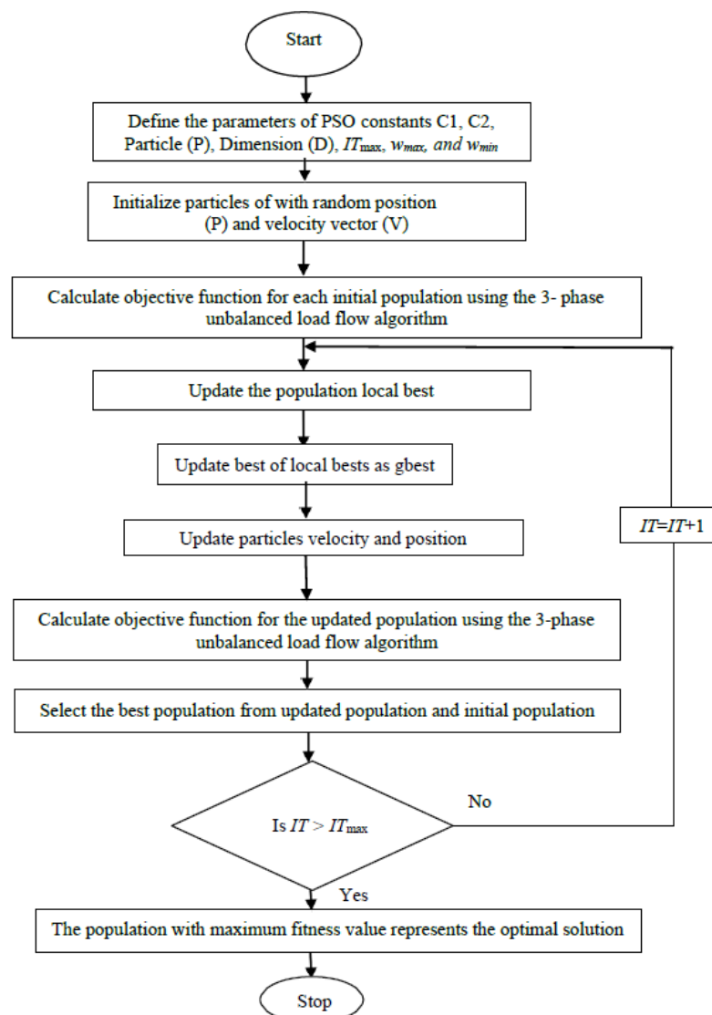
Figure 2: Flow chart of PSO algorithm
