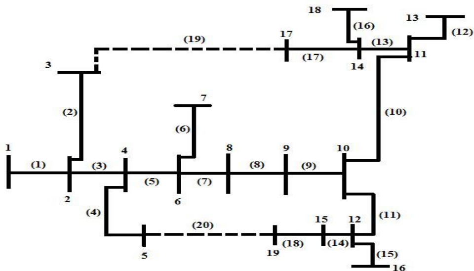
Figure 4: Diagrammatic representation of 19- bus Unbalanced Radial Distribution Network
