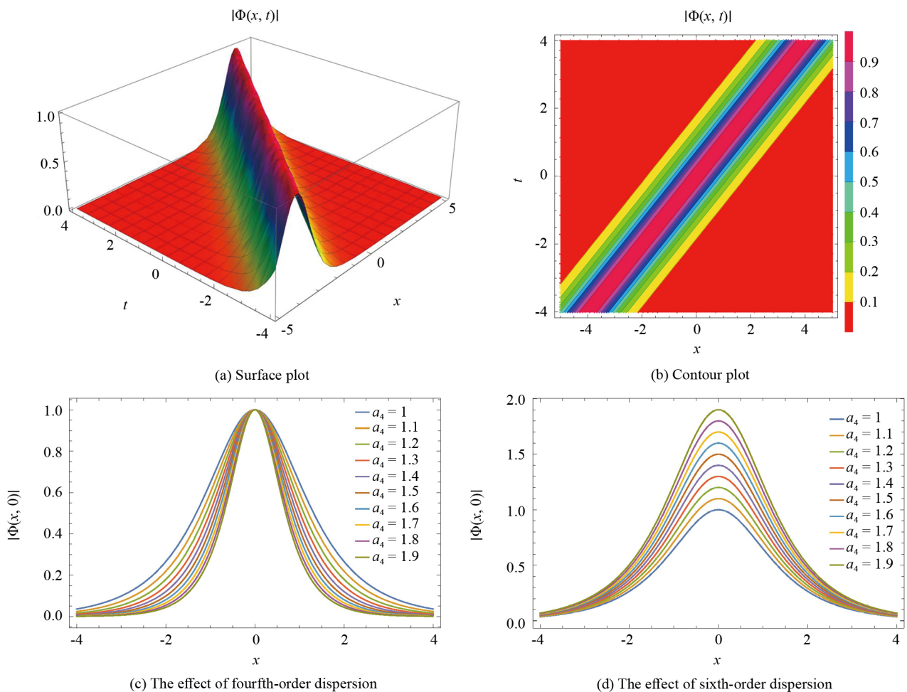
Figure 1. Profile of a bright soliton solution (39)
