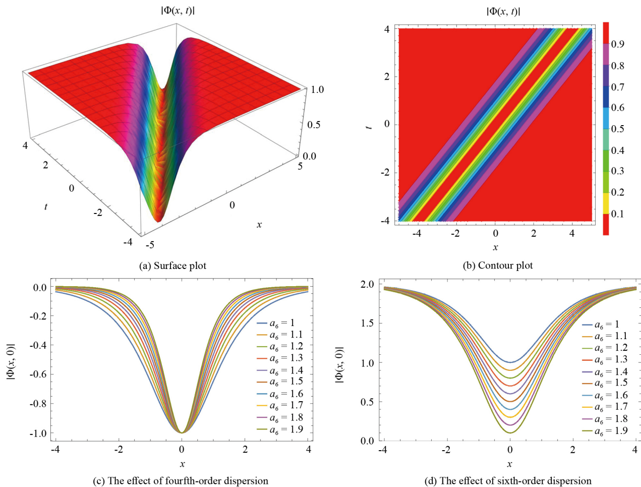
Figure 2. Profile of a bright soliton solution (66)
