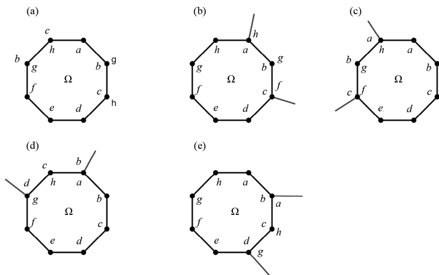
Figure 13. Region \Omega when g = b^{-1}, c = h^{-1}
