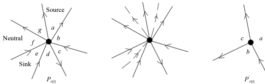
Figure 1. Pattern P_{r(t)} and its derivative P'_{r(t)}
