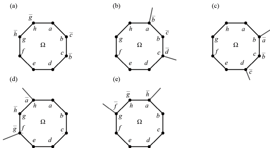
Figure 12. Region \Omega when b = c, g = h
