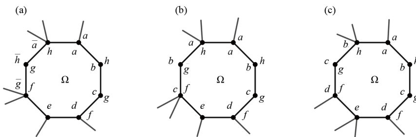
Figure 15. Region \Omega when d_{\Omega}(v_b) = d_{\Omega}(v_c) = d_{\Omega}(v_g) = 2
