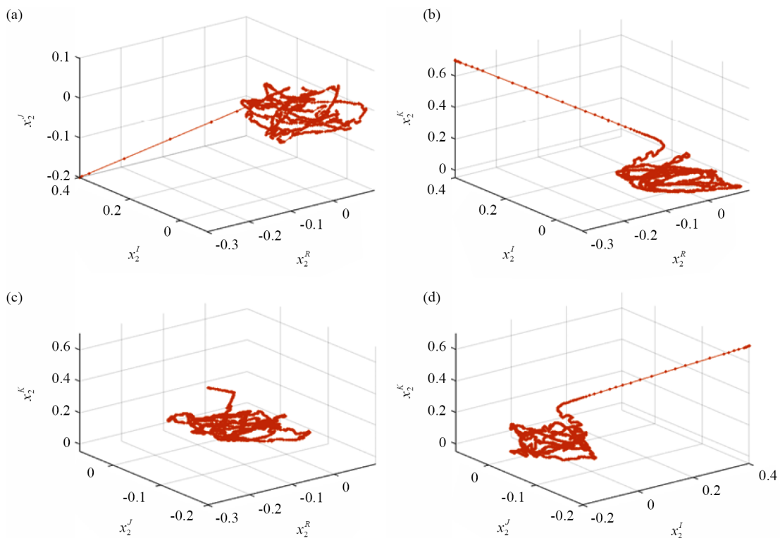
Figure 3. Stability of the system (1) in Example 5.1, x_2(t) = (x_2^R(t), x_2^I(t), x_2^J(t), x_2^K(t))^T
