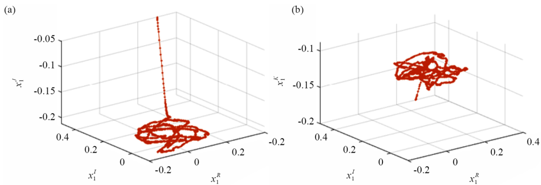
Figure 1. The state trajectories of the system (1) in Example 5.1, x_1(t) = (x_1^R(t), x_1^I(t), x_1^J(t), x_1^K(t))(t)^T , x_2(t) = (x_2^R(t), x_2^I(t), x_2^J(t), x_2^K(t))^T
