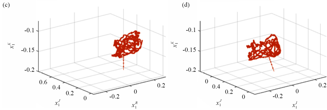
Figure 2. Stability of the system (1) in Example 5.1, x_1(t) = (x_1^R(t), x_1^I(t), x_1^J(t), x_1^K(t))^T
