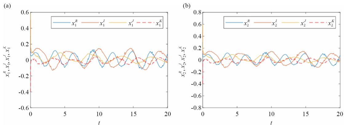
Figure 1. The state trajectories of the system (1) in Example 5.1, x_1(t) = (x_1^R(t), x_1^I(t), x_1^J(t), x_1^K(t))(t)^T , x_2(t) = (x_2^R(t), x_2^I(t), x_2^J(t), x_2^K(t))^T
