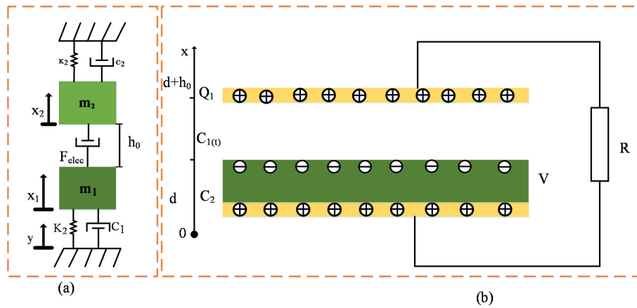
Figure 5. Electrostatic system
