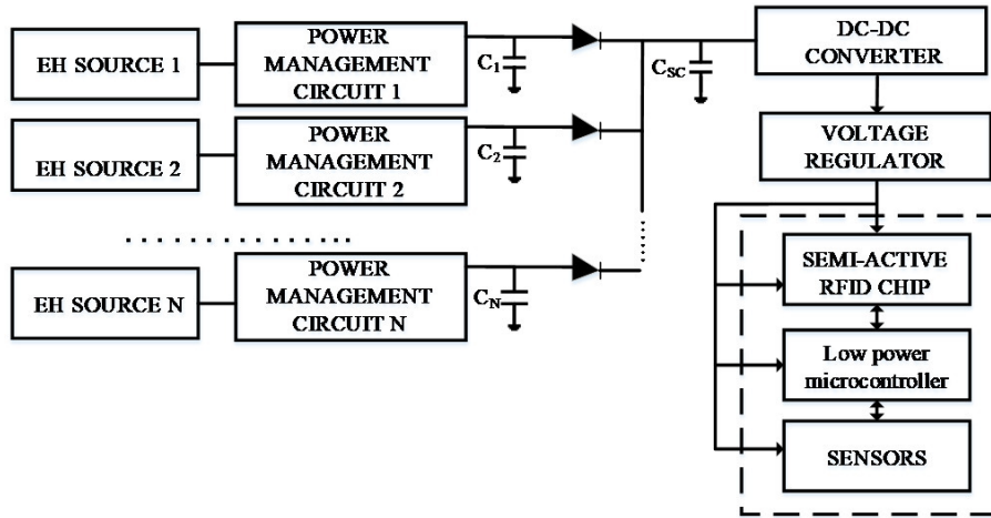
Figure 12. Hybrid energy harvesting system
