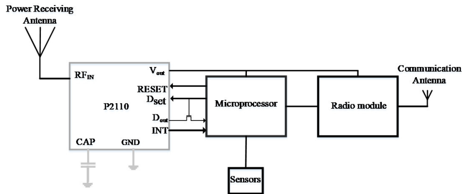
Figure 11. Radio frequency energy based harvesting system
