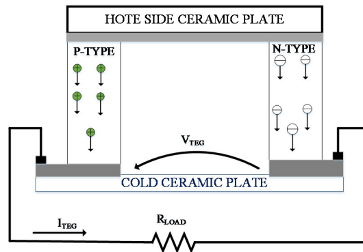
Figure 7. Thermocouple schematic
