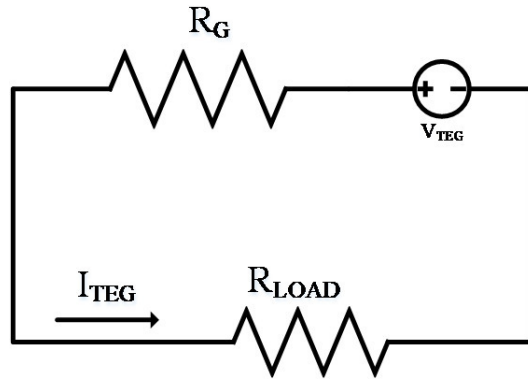
Figure 8. Equivalent electrical circuit of thermocouple schematic
