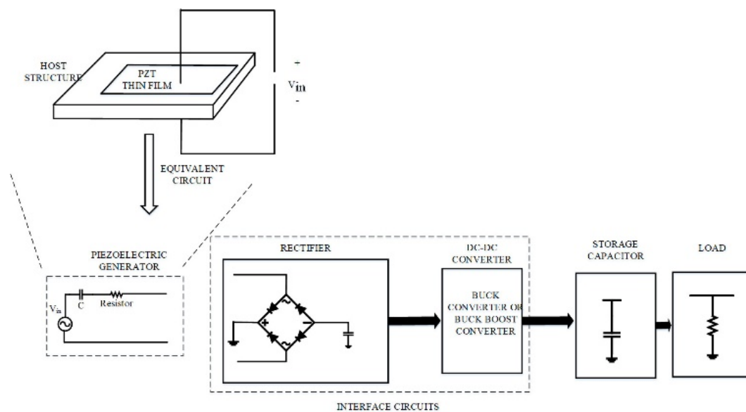
Figure 3. Basic block diagram of piezoelectric energy harvesting
