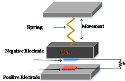
Figure 4. Electrostatic system
