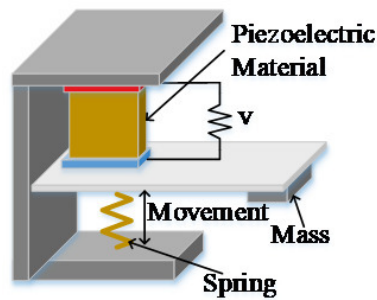
Figure 2. Piezoelectric system
