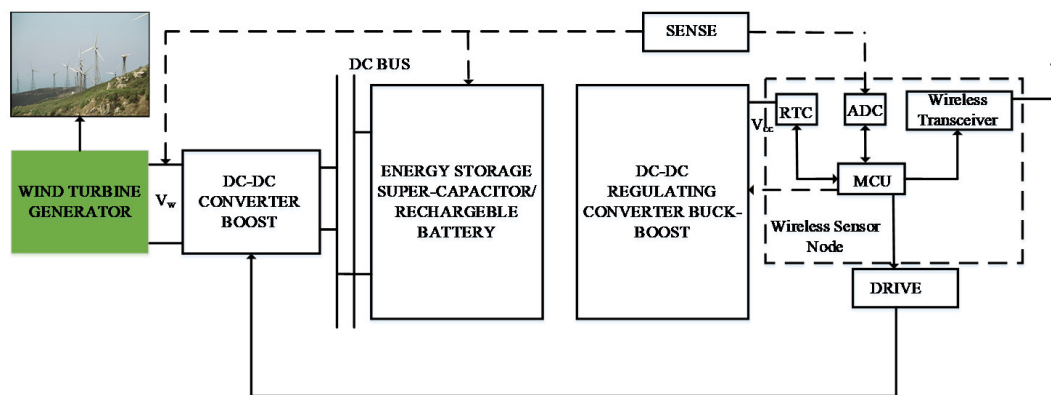
Figure 10. Wind energy based harvesting system
