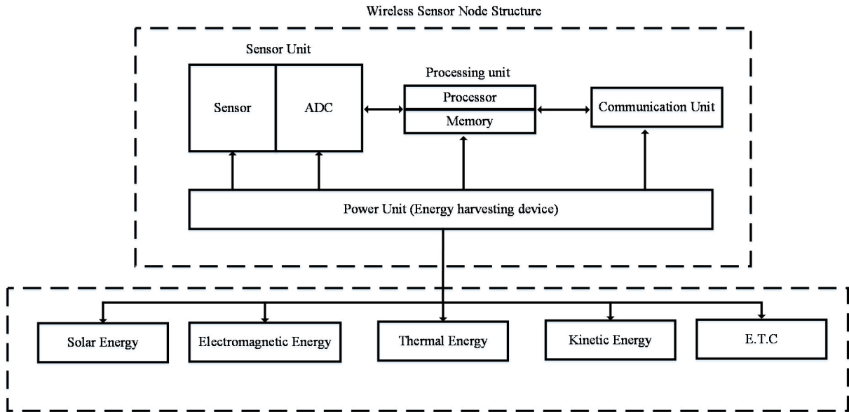
Figure 17. Hybrid energy harvesting for wireless sensor networks
