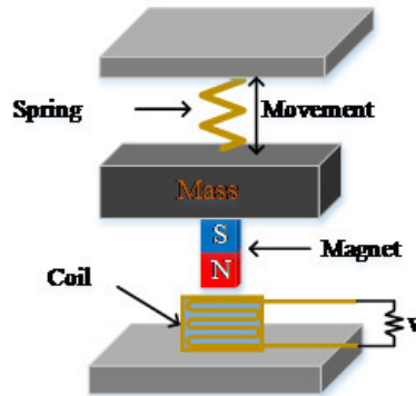
Figure 6. Electromagnetic induction system
