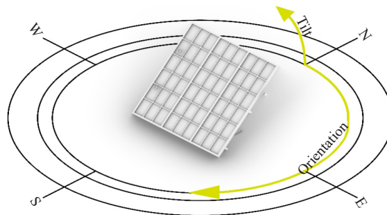
Figure 3. Tilt and orientation of solar modules illustrated
