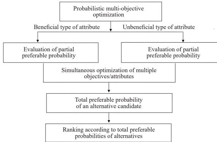
Figure 1. Evaluation procedure of the PMOO method
