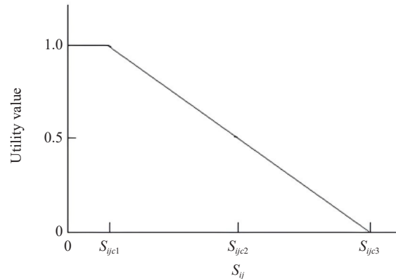
Figure 2. Illumination of “utility value” of water quality monitoring data S_{ij}
