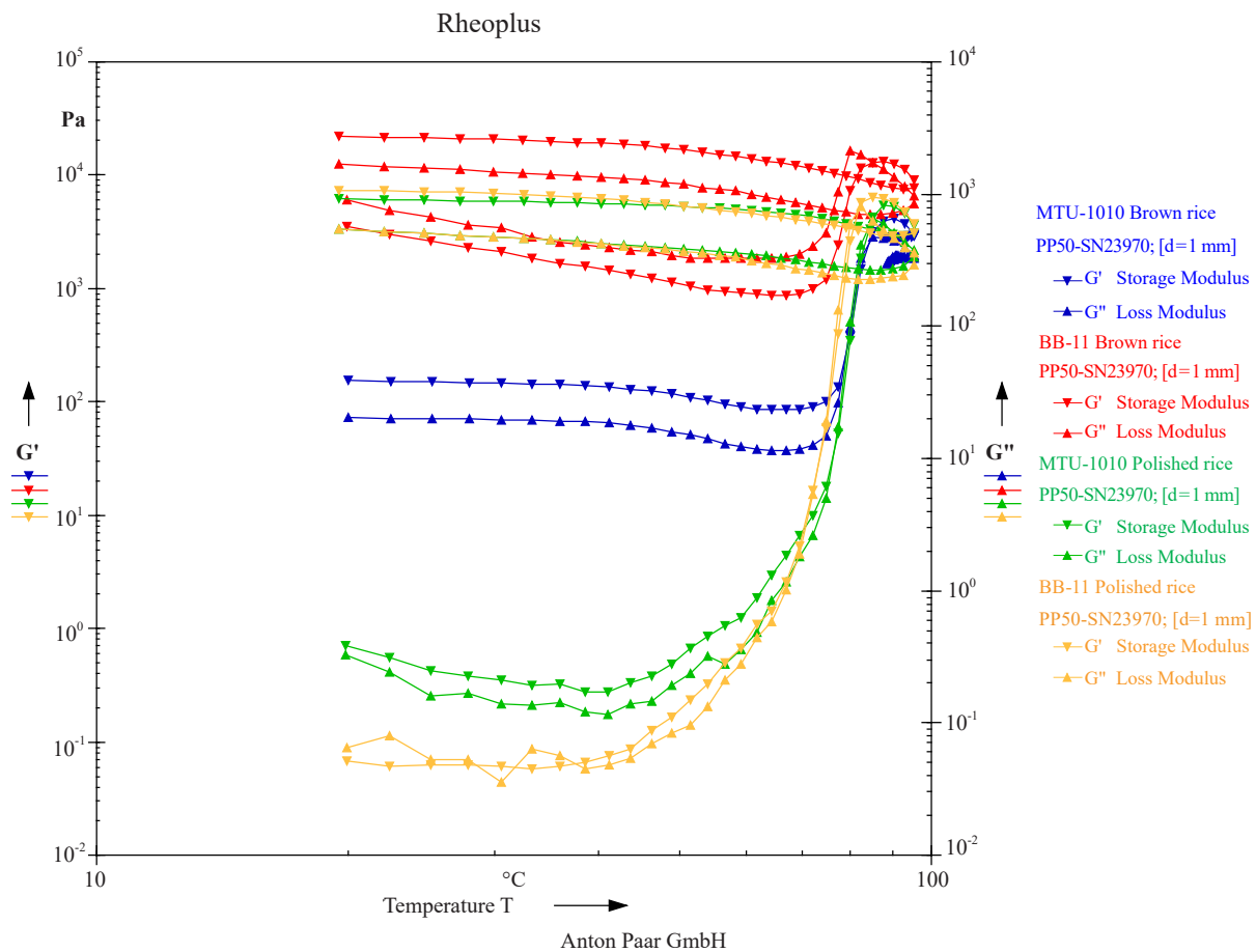
Figure 2. Rheogram showing storage and loss modulus of rice flour of paddy variety MTU-1010 and BB-11
