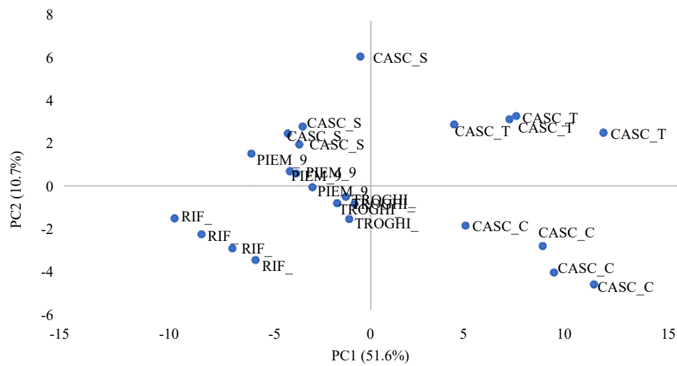
Figure 2. Plot of the first two axes of the PCA conducted on the VOCs of the different beers
