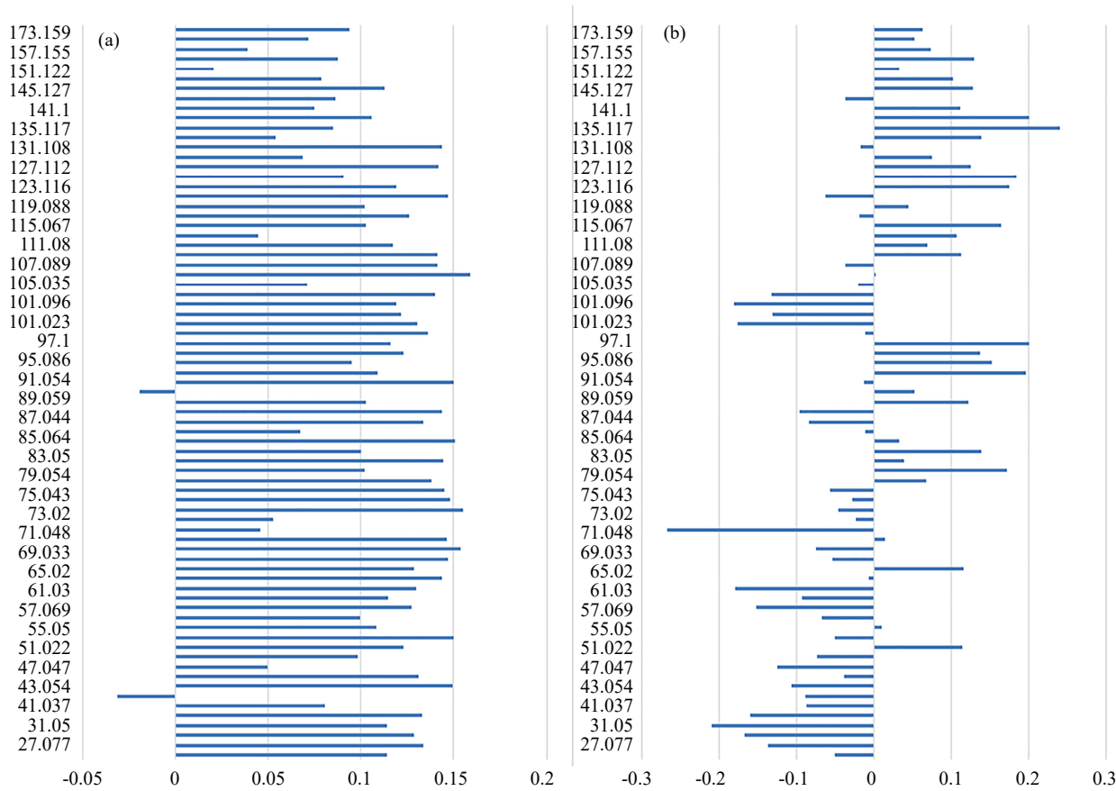
Figure 3. Loadings of the first two axes of the PCA conducted on the VOCs of the different beers. (a) = PC1; (b) = PC2
