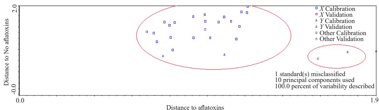
Figure 4. Discriminate analysis PCA
