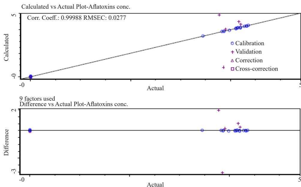
Figure 5. PLS regression statistics for 1,350-900 and 1,705-1,575cm -1 band areas. Correlation Coefficient (0.99988) calculated and displayed on plot, as well as the RMSEC (0.0277)
