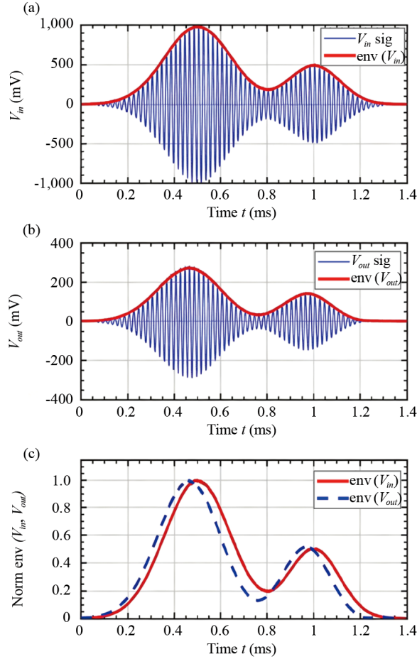
Figure 9. Time-domain analysis of BP-NGD Virtual PoC depicting plot of (a) v_{in, b} , (b) v_{out, b} and (c) \text{env}(v_{in, b}) vs \text{env}(v_{out, b}) in the range of [0, t_{\max}]
