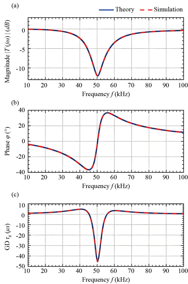
Figure 6. Comparison of theoretical and simulated responses of the proposed BP-NGD cell: VTF (a) magnitude, (b) phase and (c) GD
