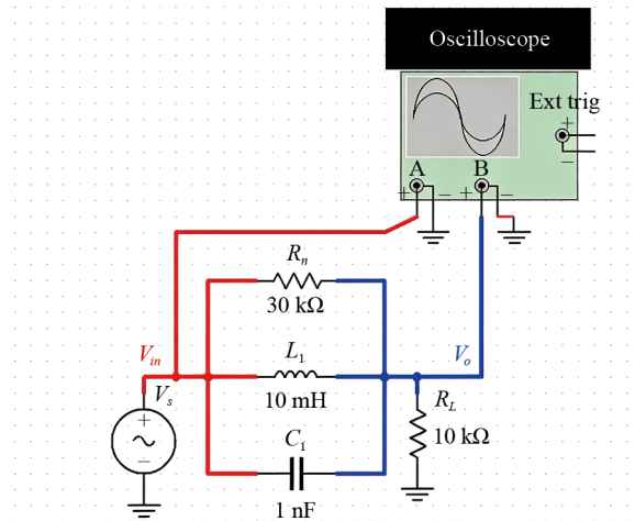
Figure 5. MULTISIM ® schematic diagram of BP-NGD circuit as Virtual POC
