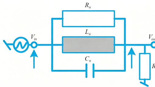
Figure 3. Passive parallel RLC BP-NGD circuit topology
