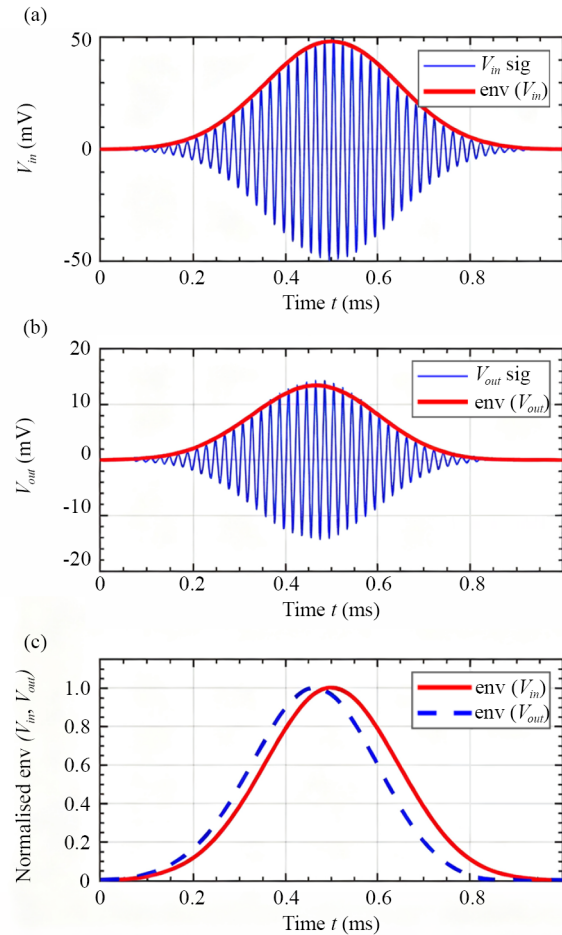
Figure 8. Time-domain analysis of BP-NGD Virtual PoC depicting plot of (a) v_{ina} , (b) v_{outa} and (c) \text{env}(v_{ina}) vs \text{env}(v_{outa}) in the range of [0, t_{\max}]
