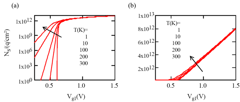
Figure 15. Variations with front gate voltage V_{g1} of the sheet carrier density N_s in log scale (a) and linear scale (b) for various temperatures as obtained in a FDSOI structure ( t_{ox1} = 2 nm, t_{ox2} = 20 nm, t_{si} = 10 nm, V_{g2} = 0 )
