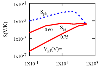
Figure 21. Variations with temperature T of the sheet electronic thermopower S_{es} for two front gate voltages V_{g1} (red solid lines) and of the phonon drag thermopower S_{ph} as given by Mahan model [28] of Equation (29) (blue dashed line) as obtained in a FDSOI structure ( t_{ox1} = 2 nm, t_{ox2} = 20 nm, t_{si} = 10 nm, V_{g2} = 0 )
