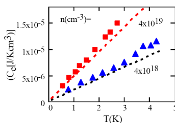
Figure 6. Experimental (symbols) and theoretical (dashed lines) variations of electronic heat capacitance C_e with temperature. Experimental data obtained from [20] on bulk silicon with various doping levels. Theoretical data from Equation (10) or (22)
