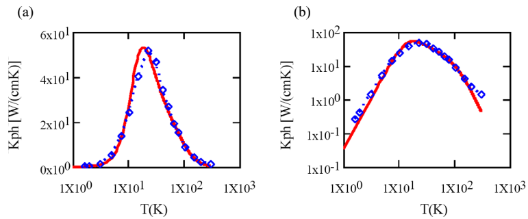
Figure 8. Variations of phonon heat conductivity K_{ph} with temperature T in linear scale (a) and log scale (b) as obtained from Equation (28) and experimental data of [23] for bulk silicon (Parameters: v_s = 9 \times 10^5 cm/s, \tau_{ph0} = 0.21 \mu s and T_0 = 14 K)
