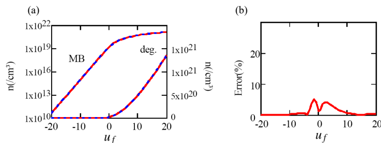
Figure 3. (a) Variations of carrier concentration n with reduced Fermi energy u_f in log scale and linear scale as obtained by exact Fermi-Dirac statistics (solid lines) and by analytical approximation of Equation (19) (dashed lines) and (b) Variations of corresponding error
