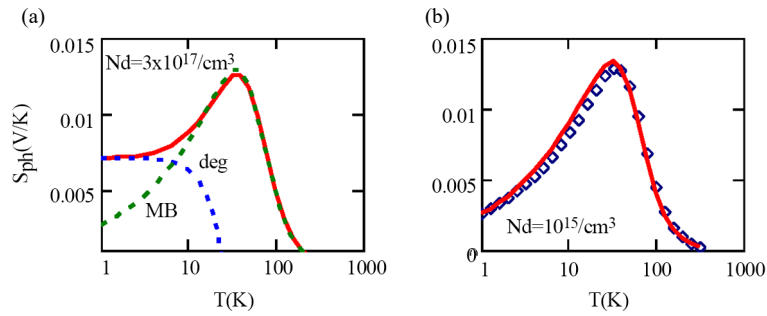
Figure 11. Variations of phonon drag thermopower S_{ph} with temperature T : (a) as obtained from Cantrell and Butcher model [27] of Equation (30) (red solid line) and from MB and degenerate asymptotic approximations (dashed lines) of Equations (33) and (34), and, (b) as obtained from Equation (30) (solid line) and extrapolated Mahan's data [28] (symbols) for low doped silicon (Parameters: v_s = 9 \times 10^5 cm/s, \tau_{ph0} = 18 ns and T_0 = 58 K)
