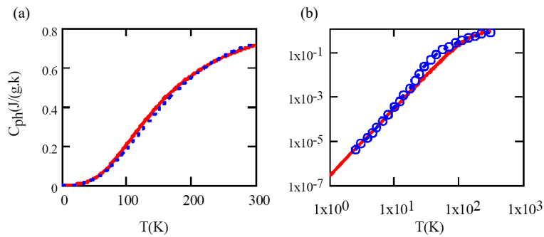
Figure 7. (a) Variations of phonon heat capacitance C_{ph} with temperature as obtained from exact Debye Equation (24) (solid line) and analytical approximation formula (26) (dashed line). (b) Experimental (symbols) and theoretical (solid line) variations of phonon heat capacitance C_{ph} with temperature as obtained from bulk silicon data of [21] and from Debye model of Equations (24) or (26)
