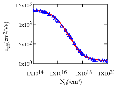
Figure 10. Variations of electron effective mobility \mu_{eff} with doping level N_d as obtained from modelling with Equations (1), (3), (31) and (32a) (red solid line) and from experiment (room temperature standard Si data [31])
