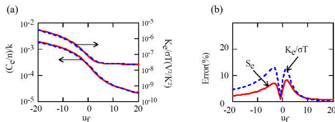
Figure 4. (a) Variations of electronic thermopower S_e and reduced electronic heat conductivity K_e/\sigma T with reduced Fermi energy u_f as obtained by exact Fermi-Dirac statistics (solid lines) and by analytical approximation of Equations (20) and (21) (dashed lines) and (b) Variations of corresponding error
