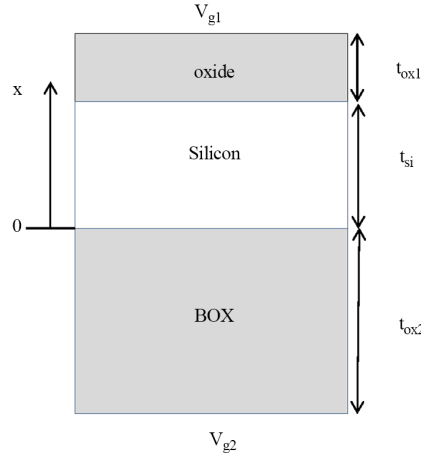
Figure 12. Schematic of FDSOI structure used for simulation ( t_{ox1} = 2 nm, t_{ox2} = 20 nm, t_{si} = 10 nm)
