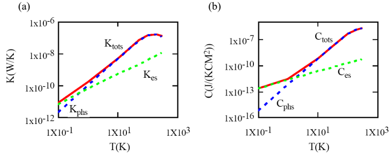
Figure 18. (a) Variations with temperature of whole sheet thermal conductivity K_{\text{tots}} (red solid line), sheet phonon thermal conductivity K_{\text{phs}} (blue dashed line) and sheet electronic thermal conductivity K_{\text{es}} (green dashed line). (b) Variations with temperature of whole thermal capacitance C_{\text{tots}} (red solid line), sheet phonon thermal capacitance C_{\text{phs}} (blue dashed line) and sheet electronic thermal capacitance C_{\text{es}} (green dashed line) as obtained in a FDSOI structure ( t_{\text{ox}1} = 2 nm, t_{\text{ox}2} = 20 nm, t_{\text{si}} = 10 nm, V_{g1} = 1.5 V, V_{g2} = 0 )
