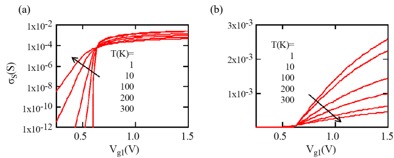
Figure 16. Variations with front gate voltage V_{g1} of the sheet electrical conductivity \sigma_s in log scale (a) and linear scale (b) for various temperatures as obtained in a FDSOI structure ( t_{ox1} = 2 nm, t_{ox2} = 20 nm, t_{si} = 10 nm, V_{g2} = 0 )
