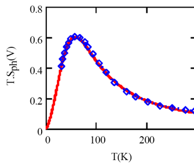
Figure 9. Variations of temperature-phonon drag thermopower product T \cdot S_{ph} with temperature T as obtained from model of Equation (29) and from modelling data of [28] for bulk silicon (Parameters: v_s = 9 \times 10^5 cm/s, \tau_{ph0} = 25 ns and T_0 = 58 K, Si doping level 10^{15}/\text{cm}^3 )
