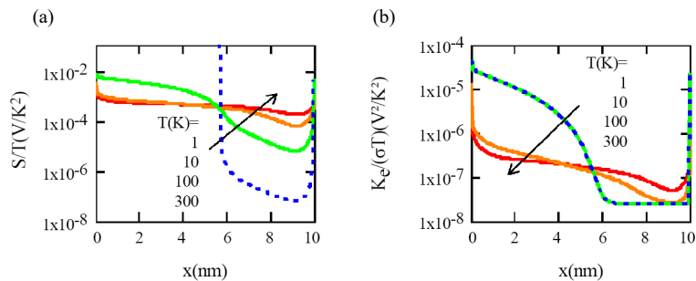
Figure 14. Spatial variations of the electronic thermopower S_e(x) (a) and of the reduced electronic heat conductivity K_e/(\sigma T)(x) (b) for various temperatures as obtained in a FDSOI structure biased in strong inversion ( t_{ox1} = 2 nm, t_{ox2} = 20 nm, t_{si} = 10 nm, V_{g1} = 1.5 V, V_{g2} = 0 )
