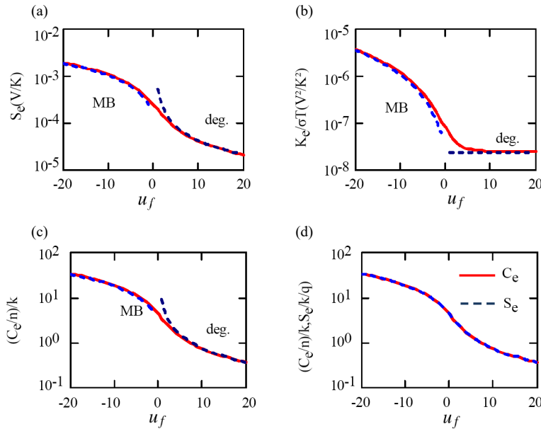
Figure 2. Variations of electronic thermopower S_e (a) and reduced electronic heat conductivity K_e/(\sigma \cdot T) (b) and reduced electronic heat capacitance C_e/N (c) and 3S_e/(2k/q) (d) with reduced Fermi energy u_f as obtained from Fermi-Dirac statistics expressions (8)–(10), as well as from Maxwell-Boltzmann (12)–(14) and degenerate (16)–(18) asymptotic approximations ( T = 300 K)
