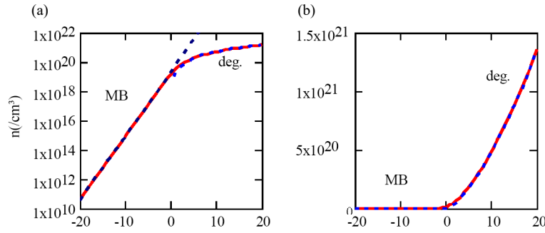
Figure 1. Variations of carrier concentration n with reduced Fermi energy u_f in log scale (a) and linear scale (b) as obtained by Fermi-Dirac statistics (solid line), Maxwell-Boltzmann (MB) and degenerate metallic (deg.) approximations (dashed lines) ( T = 300 K)
