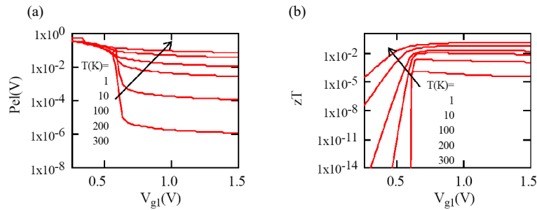
Figure 20. Variations with front gate voltage V_{g1} of the Peltier coefficient Pel and thermoelectric figure of merit factor zT for various temperatures as obtained in a FDSOI structure ( t_{ox1} = 2 nm, t_{ox2} = 20 nm, t_{si} = 10 nm, V_{g1} = 1.5 V, V_{g2} = 0 )
