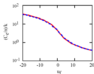
Figure 5. Variations of reduced electronic heat capacitance C_e/n with reduced Fermi energy u_f as obtained by exact Fermi-Dirac statistics (solid lines) and by analytical approximation of Equation (22) (dashed lines)
