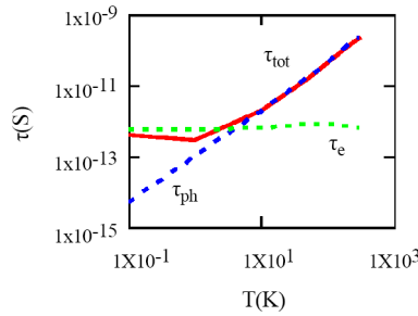
Figure 19. Variations with temperature of the total thermal response time \tau_{\text{tot}} (red solid line), thermal phonon response time \tau_{\text{ph}} (blue dashed line) and electronic response time \tau_e (green dashed line) as obtained in a FDSOI structure ( t_{\text{ox}1} = 2 nm, t_{\text{ox}2} = 20 nm, t_{\text{si}} = 10 nm, L = 100 nm, V_{g1} = 1.5 V, V_{g2} = 0 )
