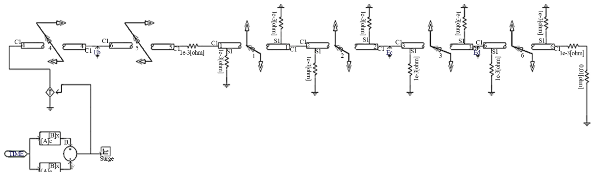
Figure 4. A four-layer co-axial cable Model representing a Gas Insulated Substation in PSCAD
