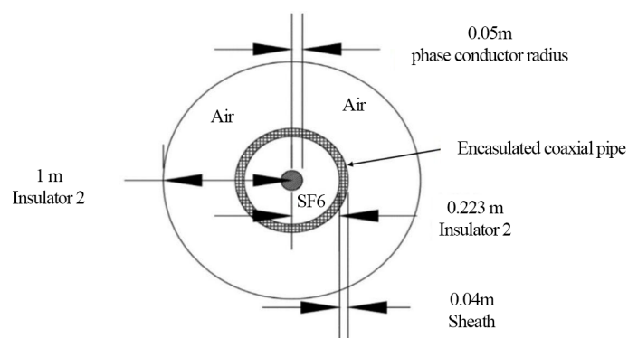
Figure 3. A four-layer co-axial cable Model representing one conductor of the phase conductors shown in Figure 1
