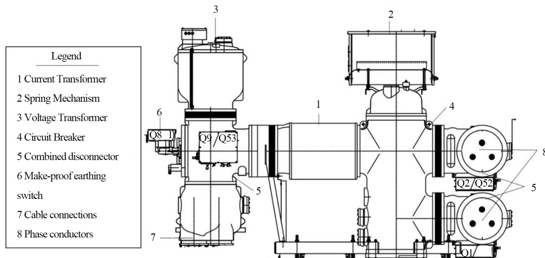
Figure 1. Physical model of a 110 KV substation
