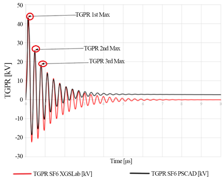
Figure 6. TGPR waveforms at 1.5 m away from point A (Refer to Figure 2) along the GIS length
