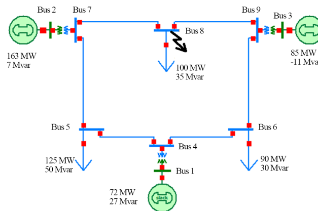
Figure 5. IEEE 9-bus system
