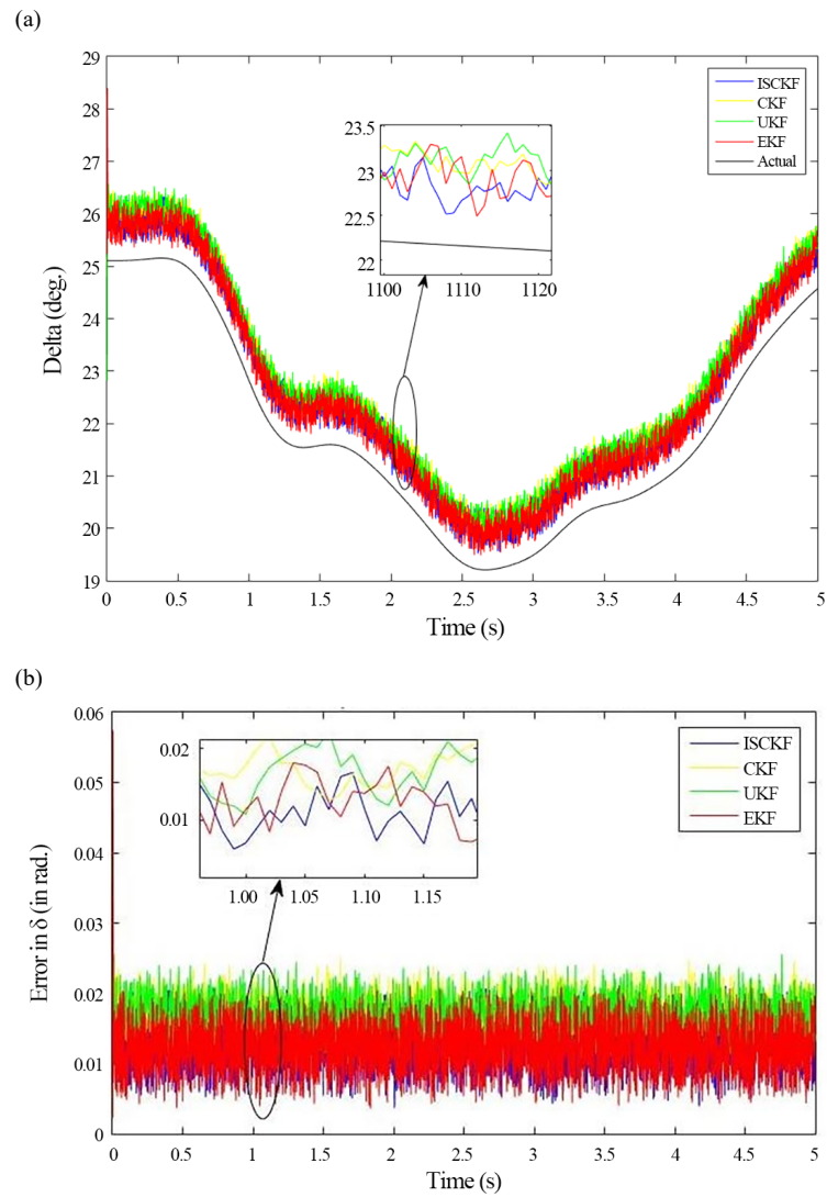
Figure 8. The rotor angle and error plots at generator bus-6 in 19-gen 42-bus test system, (a) Rotor angle plots, (b) Error in rotor angle
