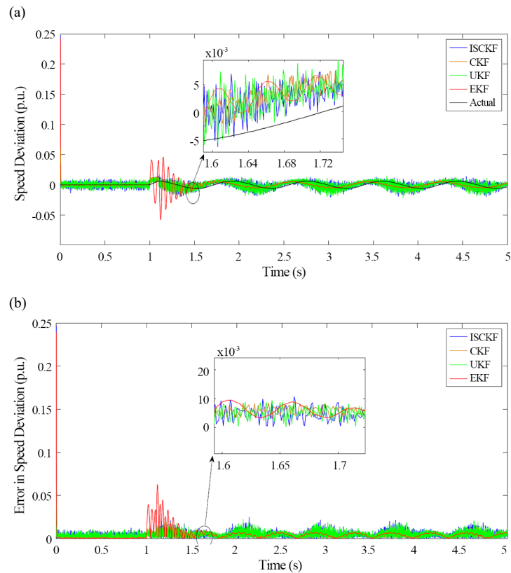
Figure 4. The estimated speed deviation and error plots for SMIB, (a) Speed deviation plots, (b) Error in speed deviation
