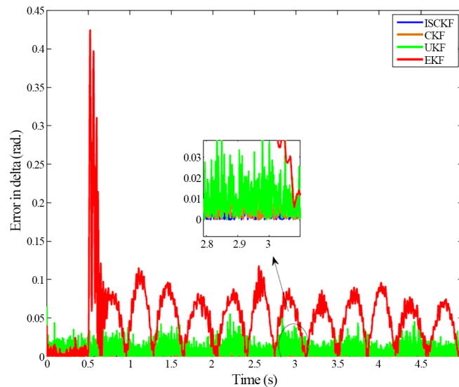
Figure 6. The estimated rotor angle and absolute error plots at generator bus-2 for IEEE 9-bus system, (a) Rotor angle plots, (b) Error in rotor angle
