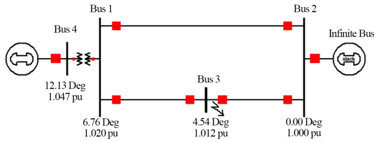
Figure 2. SMIB system
