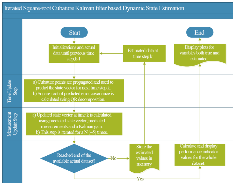
Figure 1. The flowchart for the general flow of logic in dynamic state estimation using Iterated square-root Kalman filter
