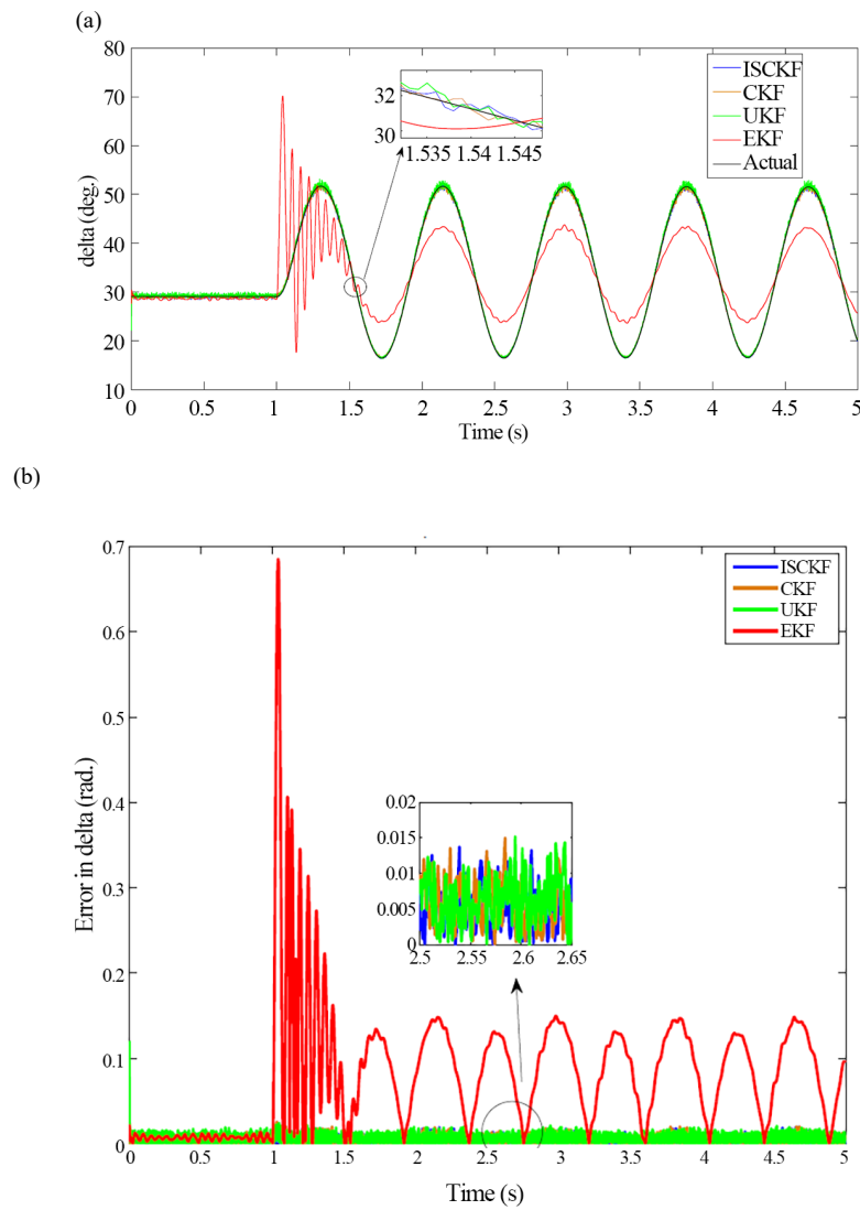
Figure 3. The estimated rotor angle and error plots at main generator bus for SMIB, (a) Rotor angle plots, (b) Error in rotor angle
