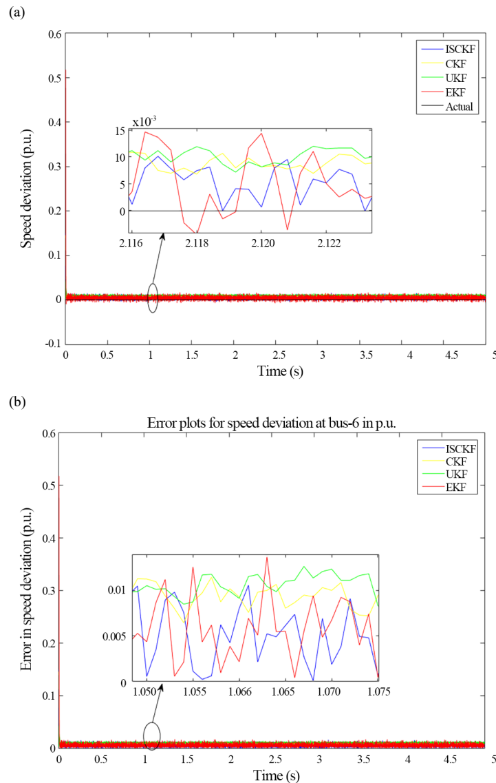
Figure 9. The estimated speed deviation and error plots at generator bus-6 in 19-gen 42-bus test system, (a) Speed deviation plots, (b) Error in speed deviation
