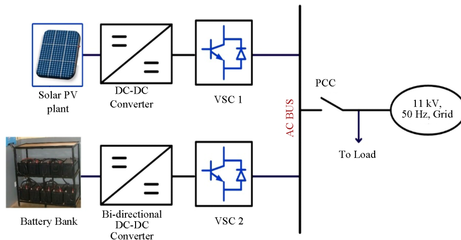
Figure 6. The battery station is linked to the grid to regulating PV output
