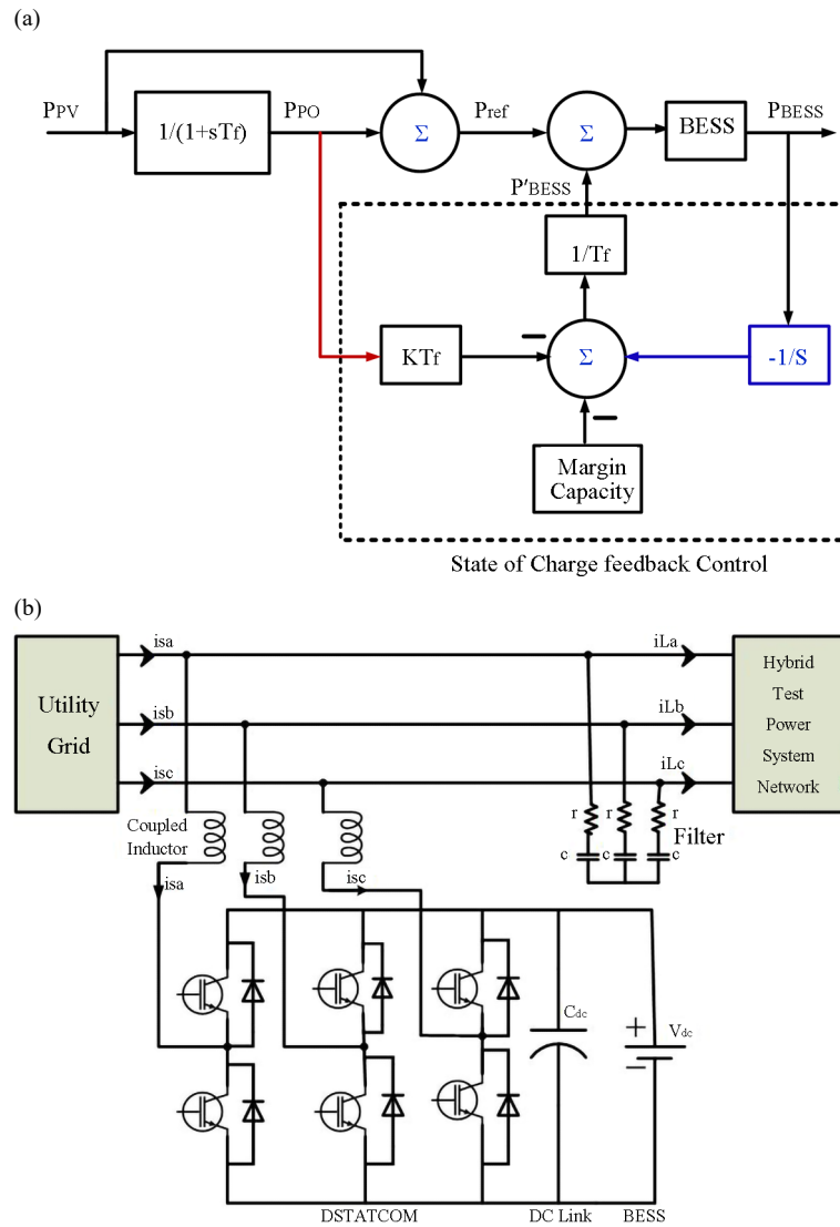
Figure 9. Control strategy for battery storage system supported by DSTATCOM for mitigating power variability (a) SOC-feedback controller (b) Power exchange by BESS
