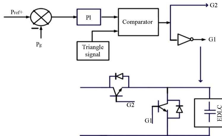
Figure 7. Buck-boost converter control
