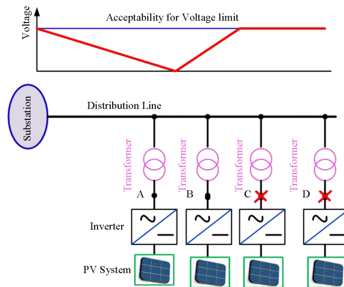
Figure 3. Issue of voltage rise at distribution network
