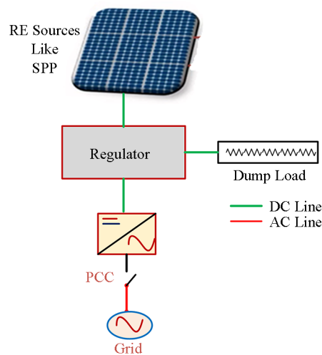
Figure 8. Grid-connected solar renewable energy source with DC dump load
