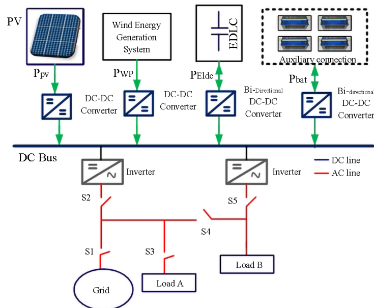
Figure 5. Structure of PV, EDLC, WEGS dispersed system
