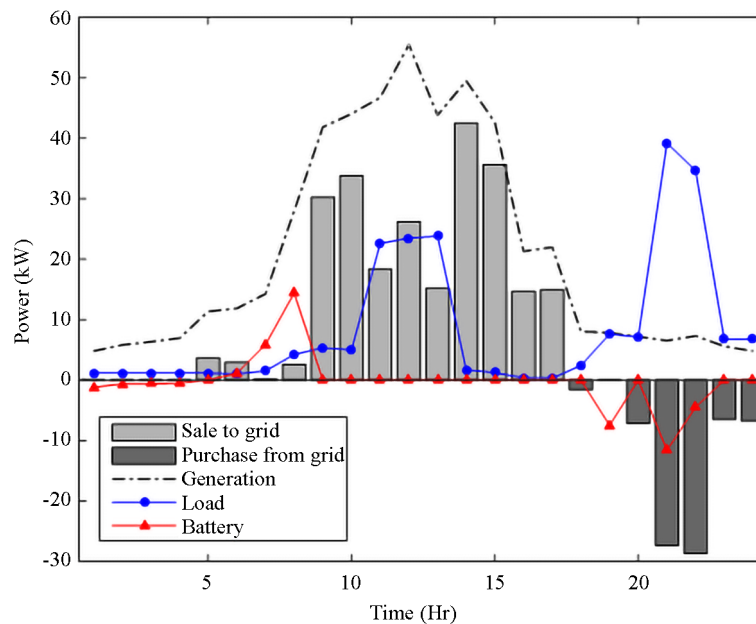
Figure 3. The optimization procedure results
