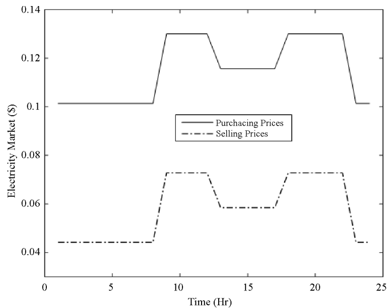
Figure 2. The electricity market values
