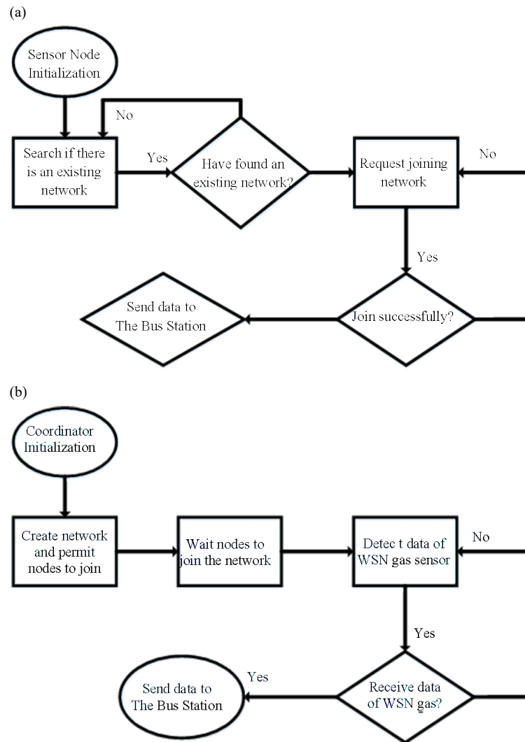
Figure 11. (a) Flow chart of the router software design, (b) Flow chart of the coordinator software design
