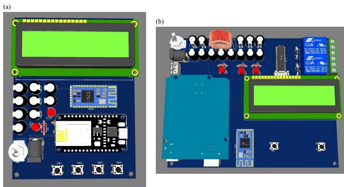
Figure 8. PCBs captured from easyeda version, (a) Zigbee coordinator and (b) Zigbee router
