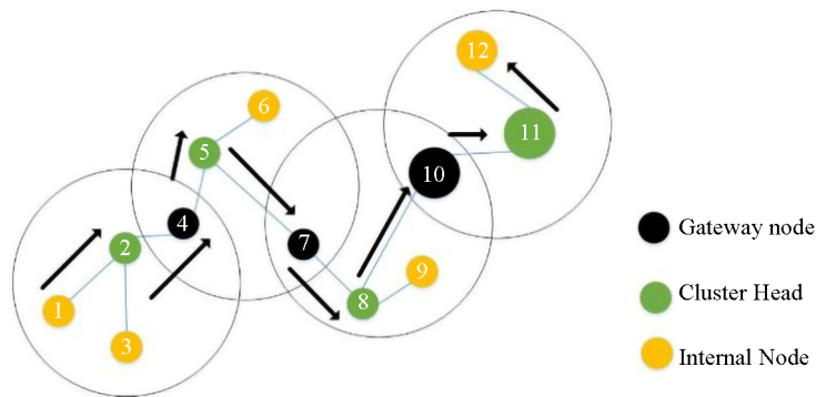
Figure 3. Cluster-head gateway switch routing protocol
