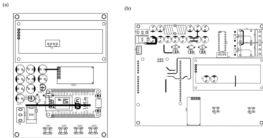
Figure 7. PCBs in PDF version. From left to right, there is (a) Zigbee coordinator and (b) Zigbee router
