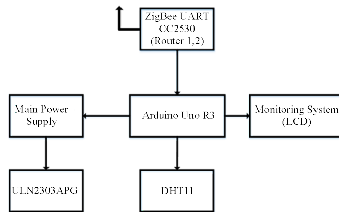
Figure 10. ZigBee router system with a DHT11 sensor
