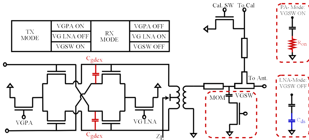
Figure 13. PA-LNA based on unbalanced neutralized bi-directional technique [11]
