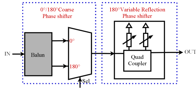
Figure 10. A 94-GHz phase shifter employing a cascaded active-passive phaseshift method, with a variable phase shift of 360^\circ with a 5-bit phase resolution [18]
