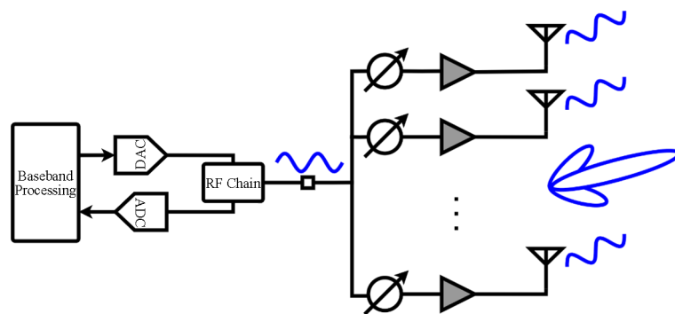
Figure 3. Analog beamforming [6]
