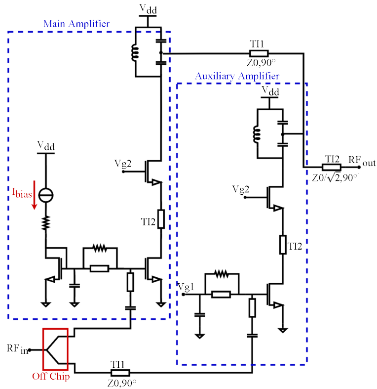
Figure 14. Schematic diagram of Doherty Amplifier utilizing a main amplifier and an auxiliary amplifier [22]
