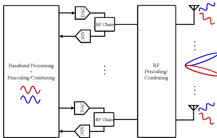
Figure 5. Hybrid beamforming [6]
