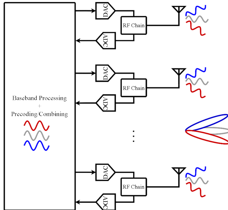
Figure 2. Digital architecture [6]
