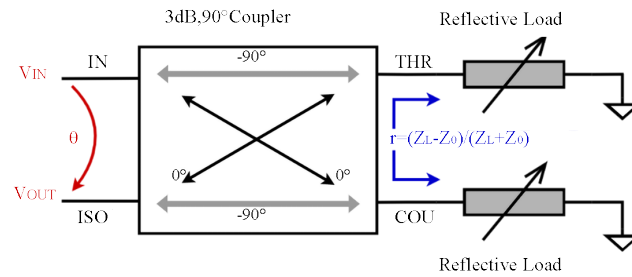
Figure 8. Reflective-Type Phase Shifter (RTPS) composed of 3 dB coupler and reflective loads [16]
