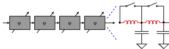
Figure 7. Switched-LC Phase Shifter circuit consisting of an LC network and a set of switches that can connect or disconnect the LC network to the input and output of the circuit [14, 16]
