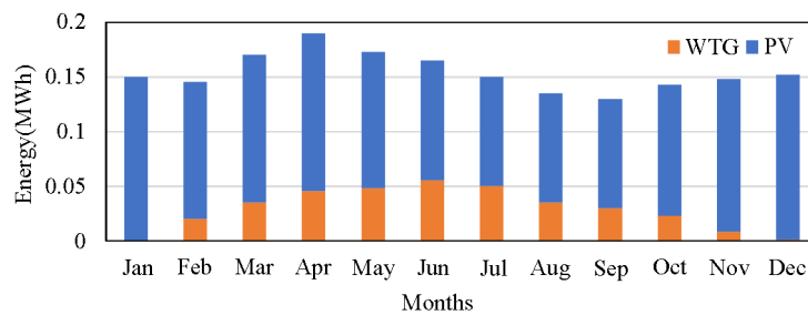
Figure 9. Simulated monthly electrical energy production from the system
