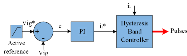
Figure 3. Controller for IG side converter
