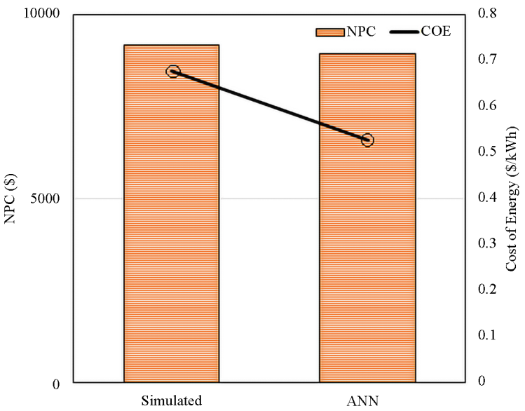
Figure 12. Comparison of NPC and COE from the simulated and optimized system data
