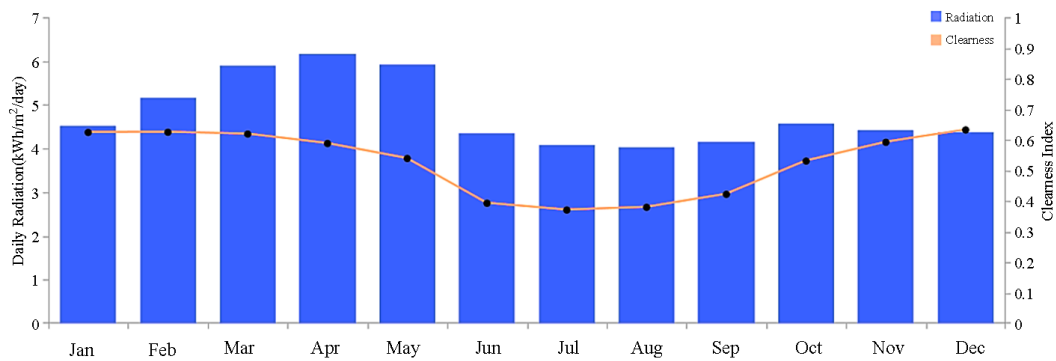
Figure 5. Solar resource data
