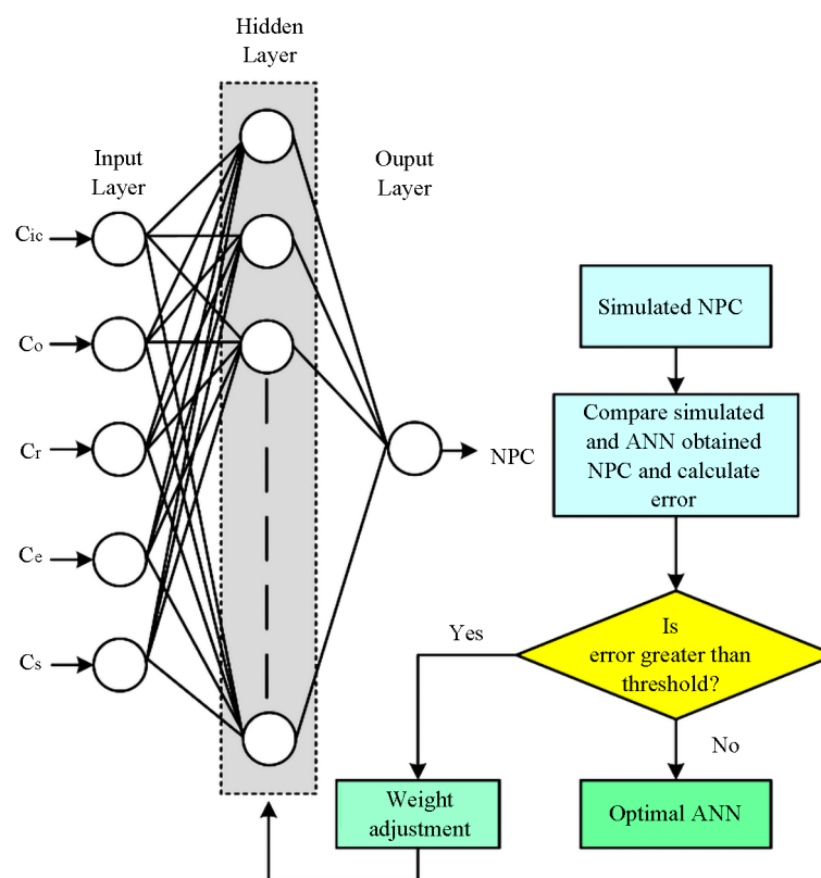
Figure 7. Proposed ANN structure
