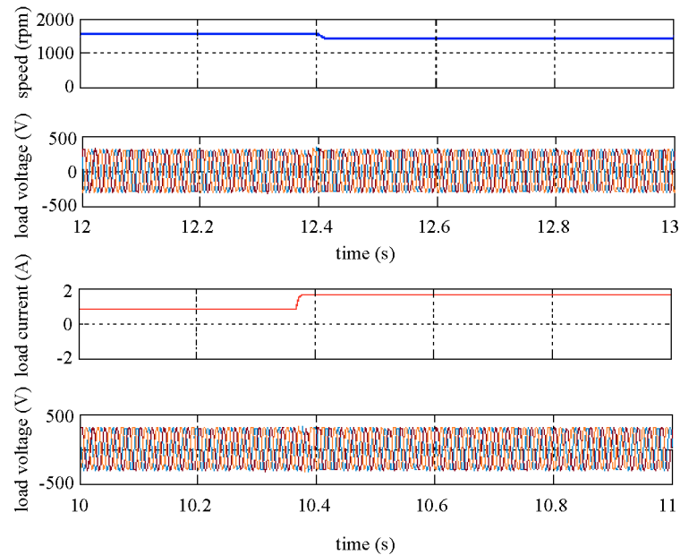
Figure 14. Variation of load voltage with change in speed and load current
