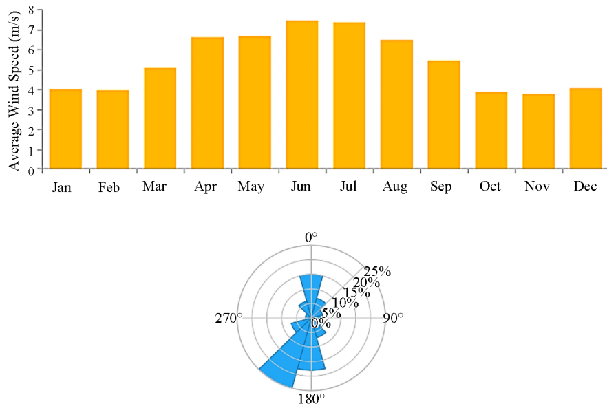
Figure 4. Wind resource profile of the place under consideration for installation along with the wind frequency rose
