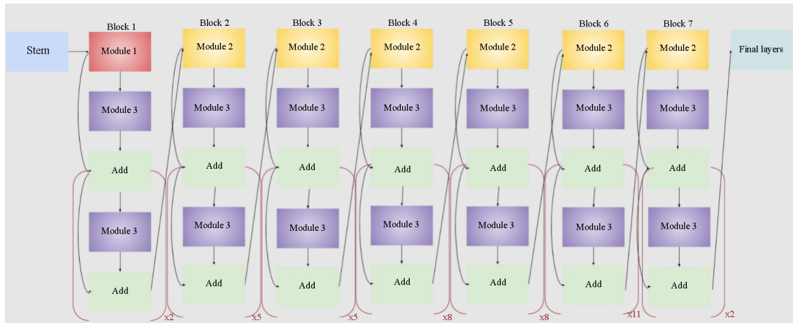
Figure 4. EfficientNet-B7 architecture
