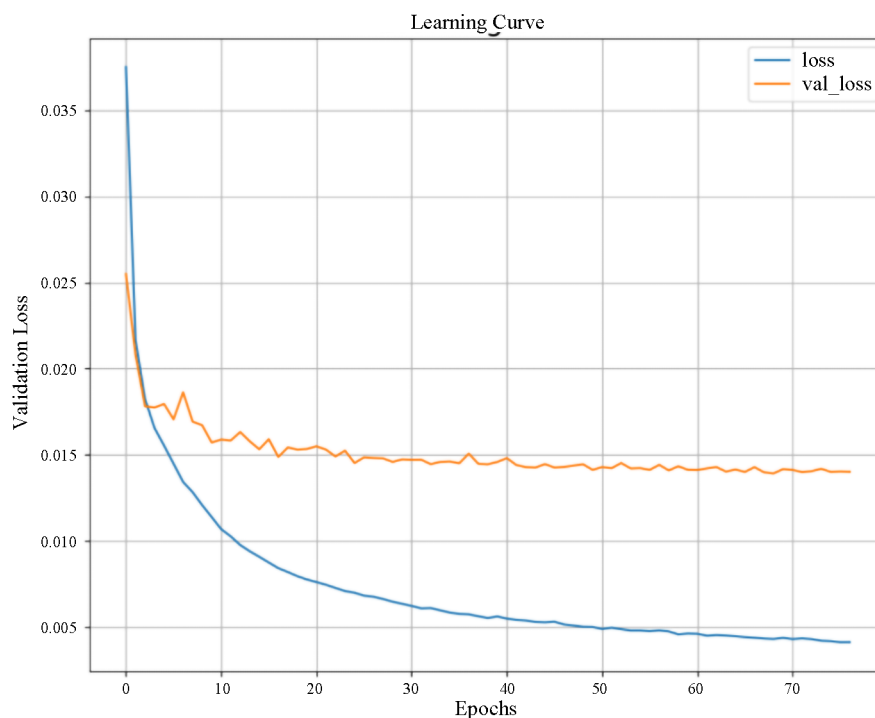
Figure 10. Loss learning curve of EfficientNet-B7
