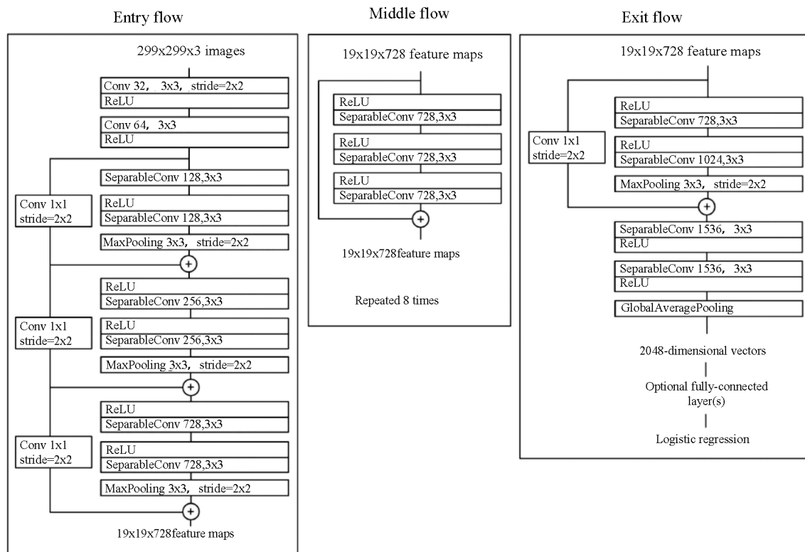
Figure 6. Xception architecture
