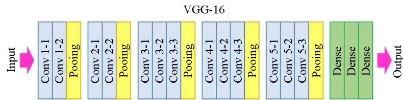
Figure 2. VGG-16 architecture
