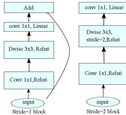
Figure 3. MobileNet-V2 architecture
