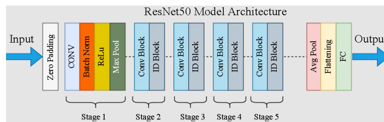
Figure 5. ResNet-50 architecture
