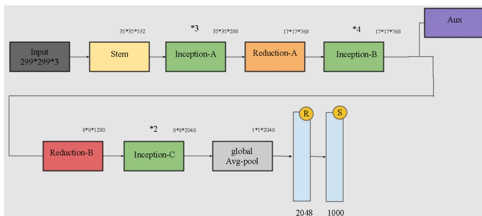
Figure 7. Inception architecture
