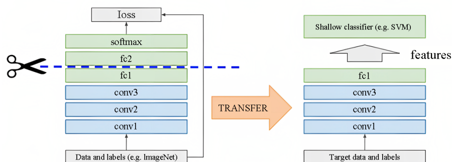
Figure 1. Transfer learning with pre-trained model as feature extractor
