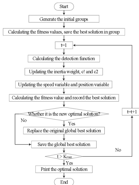
Figure 3. Flow chart for the enhanced PSO
