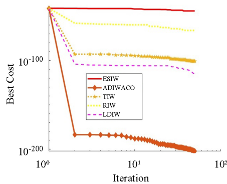
Figure 11. Optimization performance for the rotated hyper-ellipsoid function
