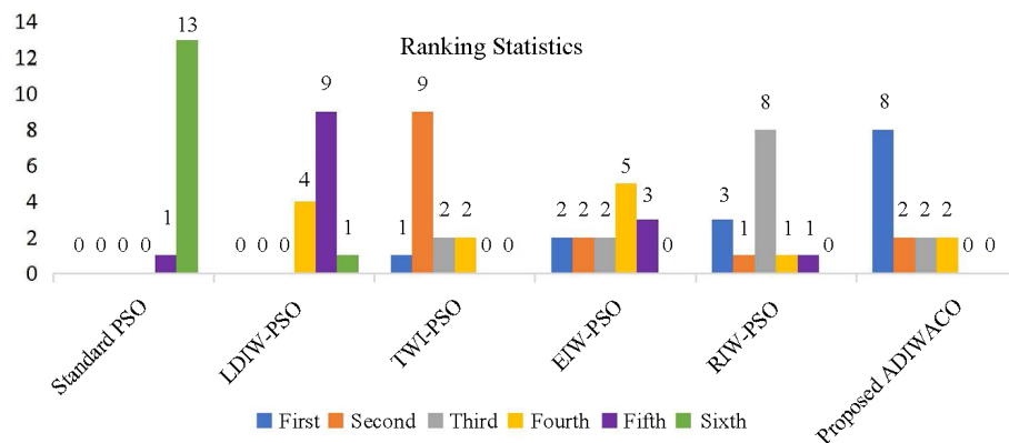
Figure 12. Ranking statistics of experimental results
