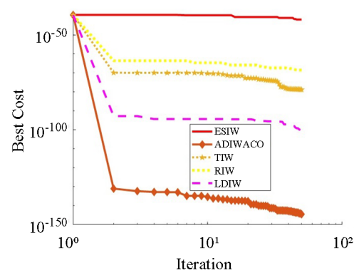
Figure 8. Optimization performance for the matyas function
