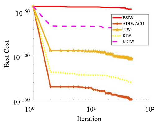
Figure 6. Optimization performance for the sphere function
