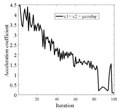
Figure 2. Behaviour of acceleration coefficient function
