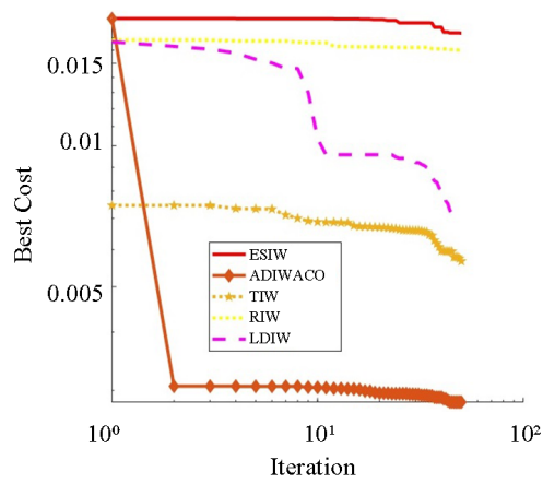
Figure 7. Optimization performance for the coville function
