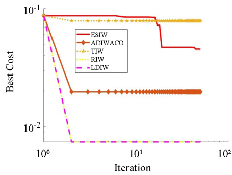
Figure 10. Optimization performance for the griewank function
