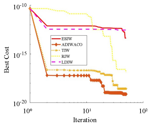
Figure 9. Optimization performance for the rosenbrock function
