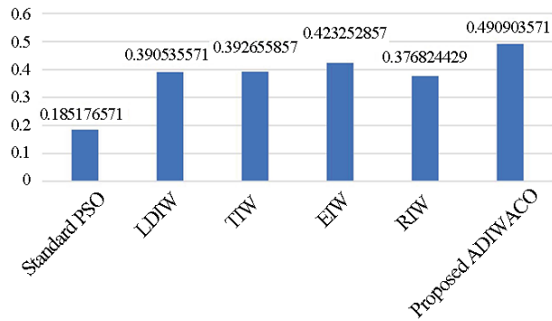
Figure 4. Average runtime of algorithms in seconds
