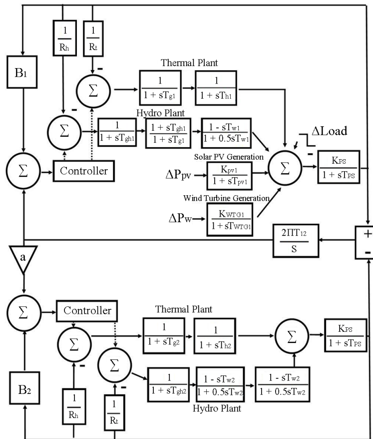
Figure 1. Block diagram of test system
