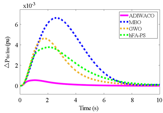
Figure 15. Scenario 4 change in tie line power
