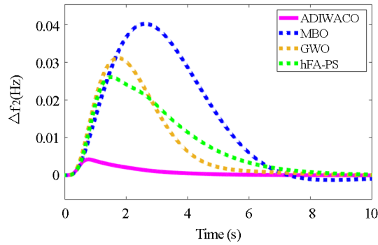
Figure 11. Scenario 3 area 2 change in frequency
