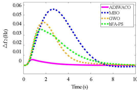
Figure 17. Scenario 5 change in area 2 frequency
