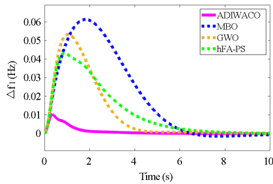
Figure 16. Scenario 5 change in area 1 frequency
