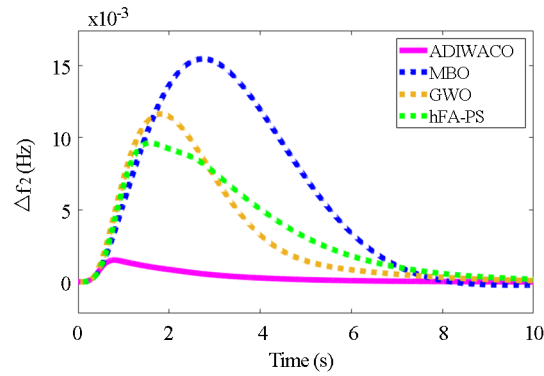
Figure 14. Scenario 4 change in area 2 frequency
