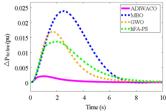
Figure 18. Scenario 5 change in tie line power
