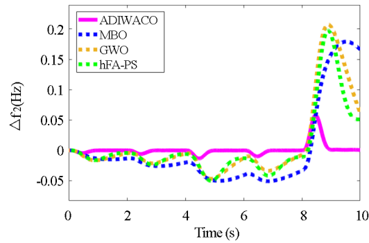
Figure 8. Scenario 2 area 2 change in frequency
