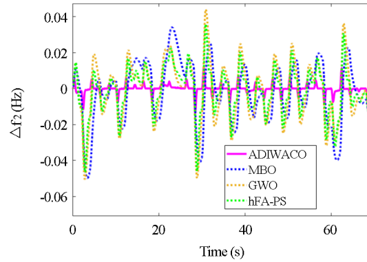
Figure 21. Scenario 6 change in area 1
