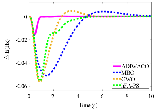
Figure 4. Scenario 1 area 2 change in frequency
