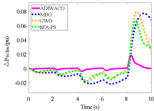
Figure 9. Scenario 2 change in tie line power
