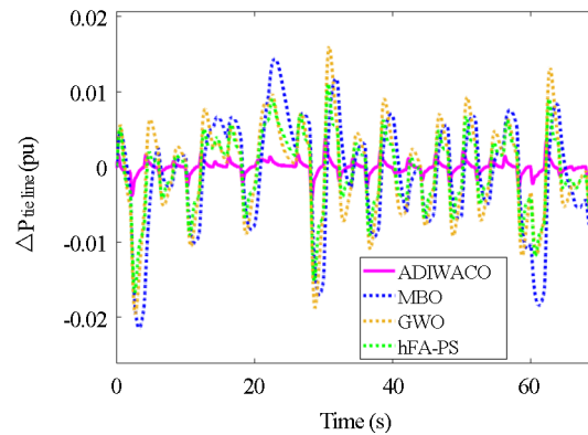
Figure 22. Scenario 6 change in tie line power
