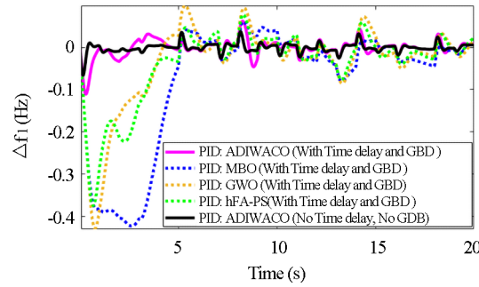
Figure 23. Scenario 7 change in area 1 frequency
