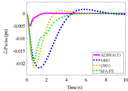
Figure 5. Scenario 1 tie line power deviation
