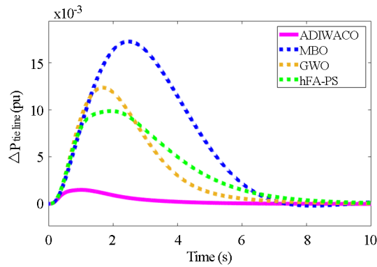
Figure 12. Scenario 3 change in tie line power
