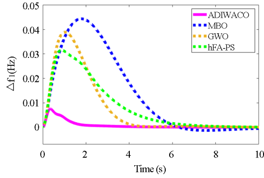
Figure 10. Scenario 3 area 1 change in frequency
