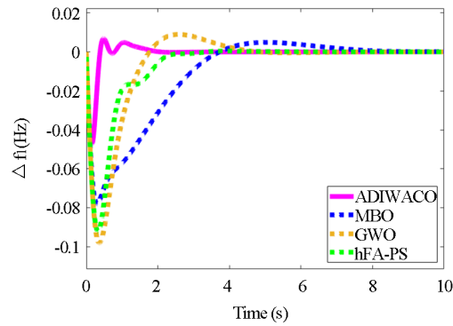
Figure 3. Scenario 1 area 1 change in frequency
