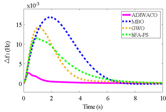
Figure 13. Scenario 4 change in area 1 frequency
