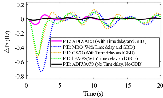
Figure 24. Scenario 7 change in area 2 frequency
