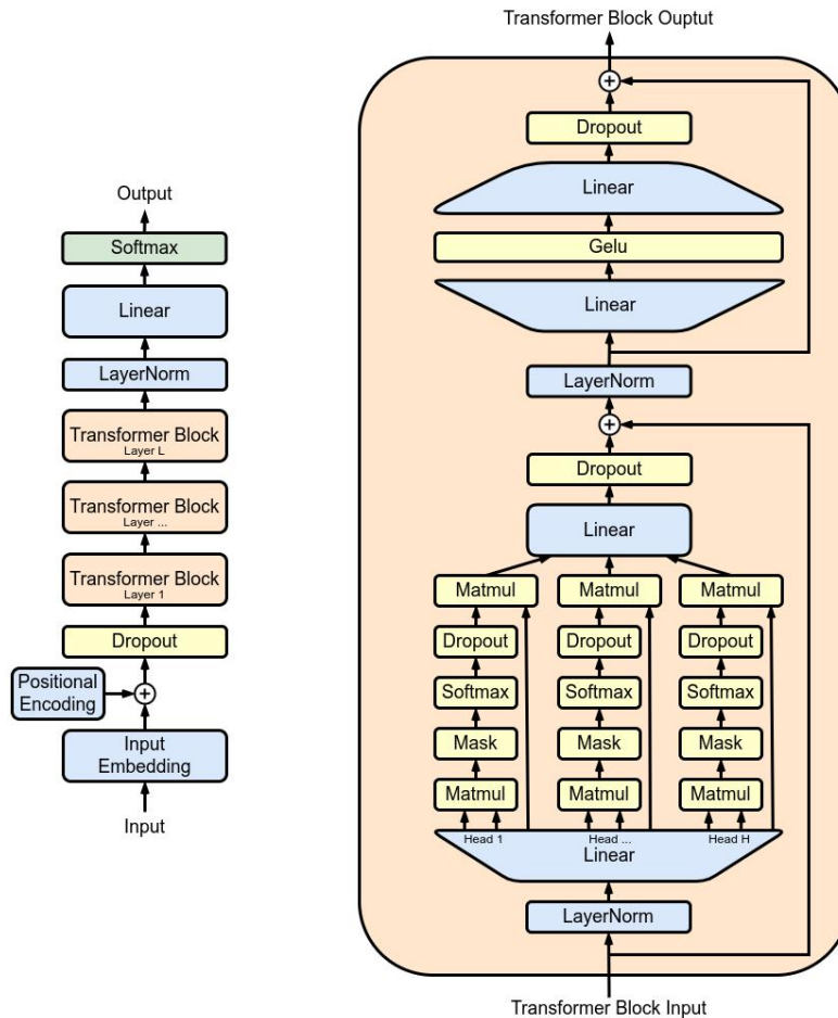
Figure 5. GPT's transformer model-based architecture [56]
