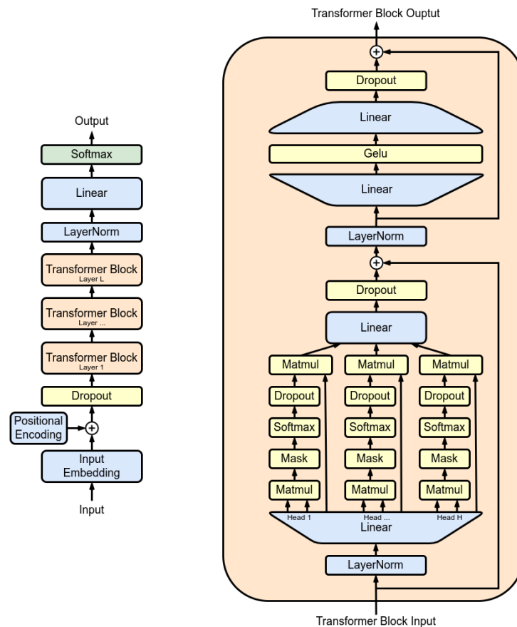
Figure 5. GPT's transformer model-based architecture [56]
