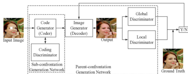
Figure 3. Recovery of a damaged image using GANs [40]
