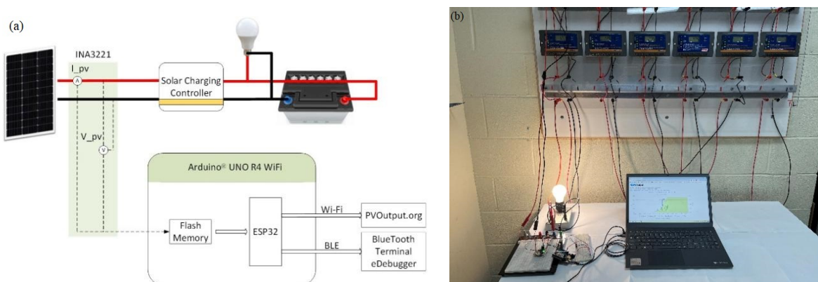
Figure 2. (a) The designed SCADA system block diagram. (b) Experimental setup
