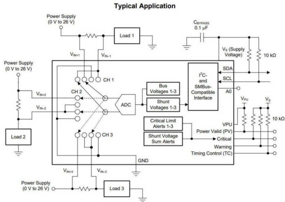
Figure 1. INA3221 schematic diagram
