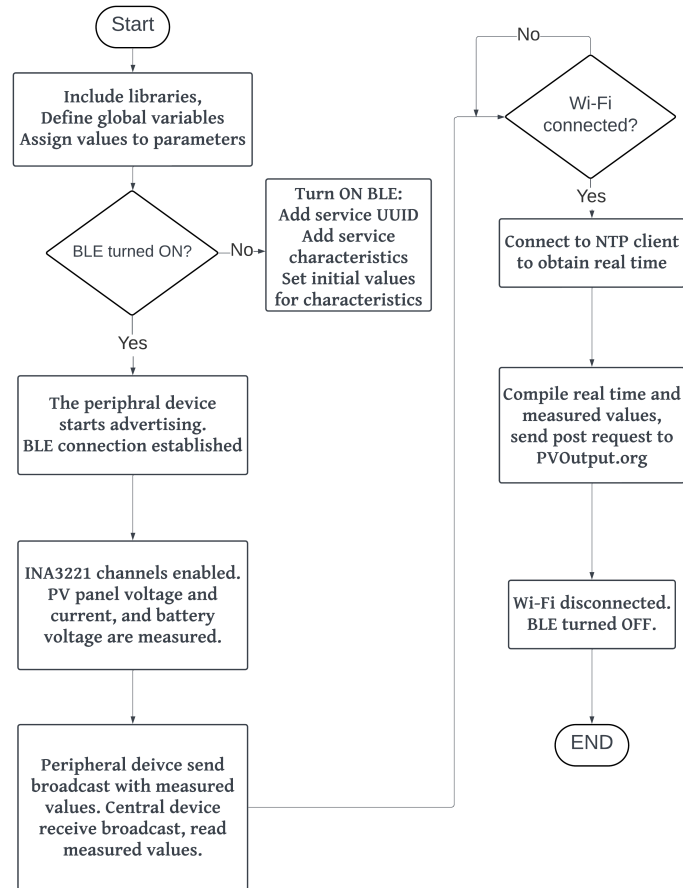
Figure 3. The SCADA system program flowchart
