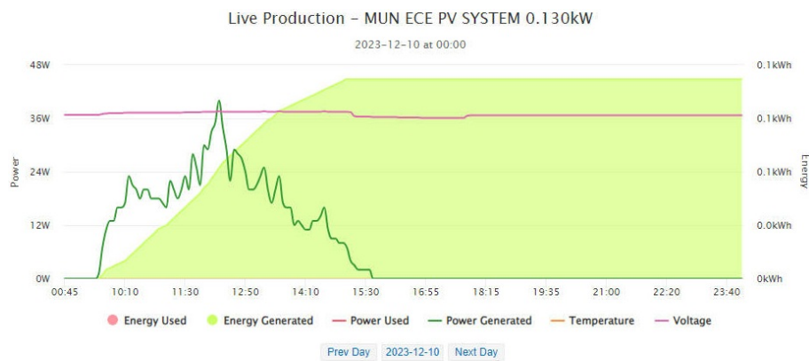
Figure 5. PV panel output power on 10 December 2023, recorded in PVOutput.org
