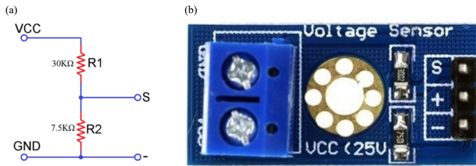
Figure 6. Voltage sensor (0-25 V). (a) Schematic diagram. (b) Sensor picture
