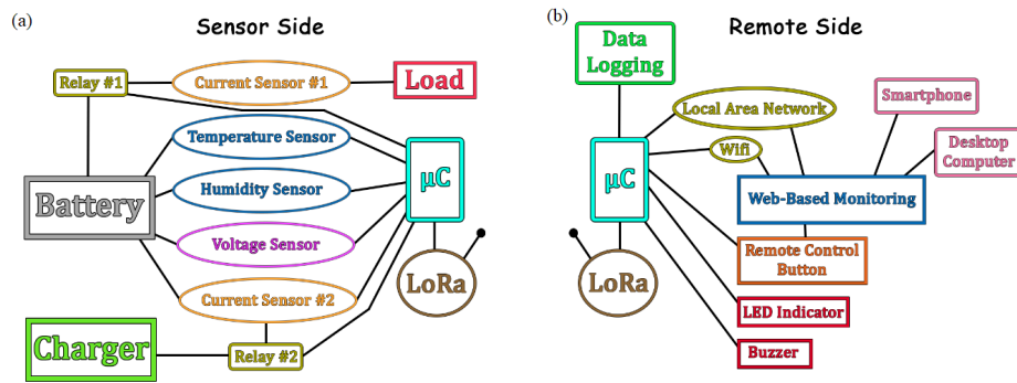
Figure 3. Block diagram of the battery monitoring system. (a) Sensor side. (b) Remote side
