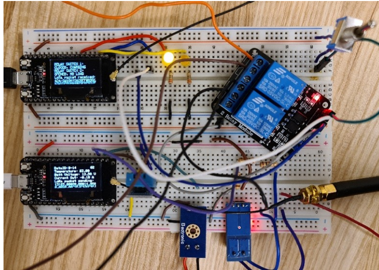
Figure 12. Sensor side of the battery monitoring system
