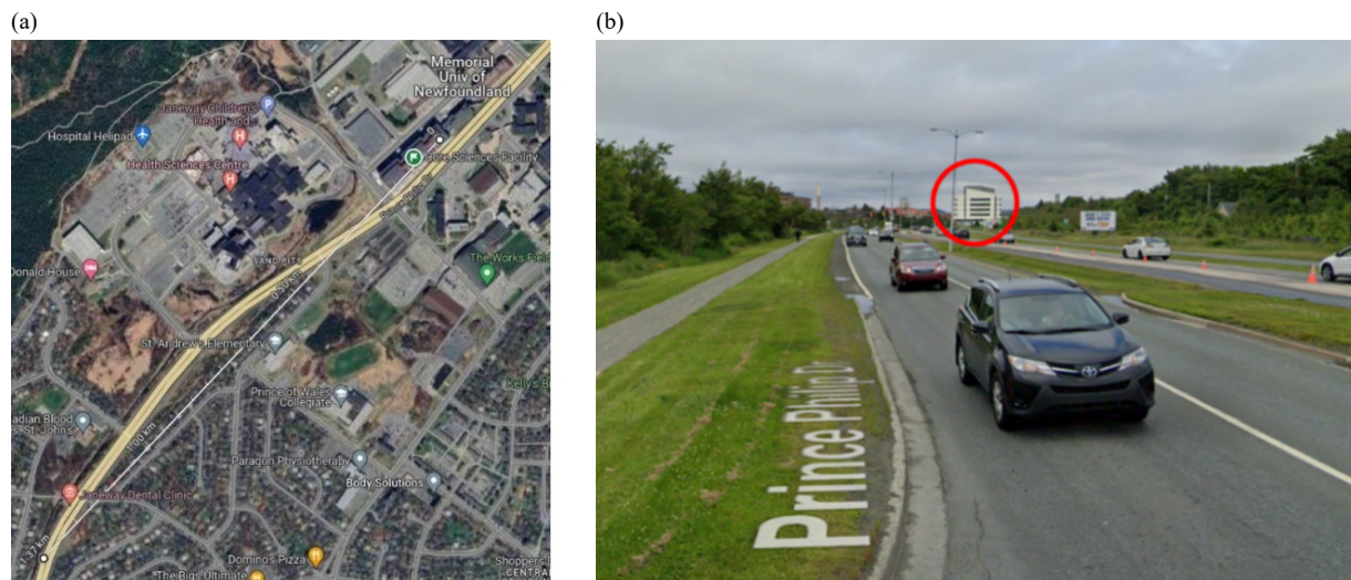
Figure 21. Range test site on a low dense space. (a) Map. (b) In-person view of the building at the distance
