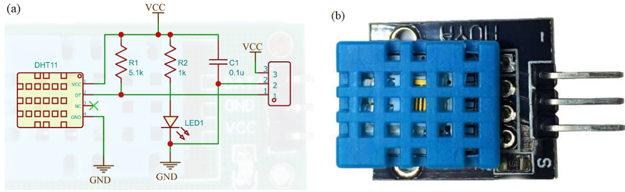
Figure 5. DHT11 temperature and humidity sensor. (a) Schematic diagram. (b) Sensor picture
