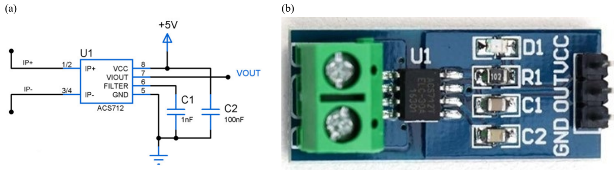
Figure 7. ACS712-20A current sensor. (a) Schematic diagram. (b) Sensor picture
