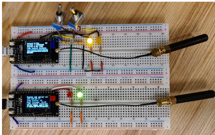
Figure 13. Remote side of the battery monitoring system
