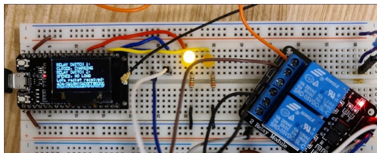
Figure 20. Sensor side relay switch CLOSED for charging/load
