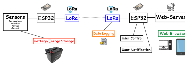
Figure 1. Graphical abstract of the proposed battery monitoring and control system
