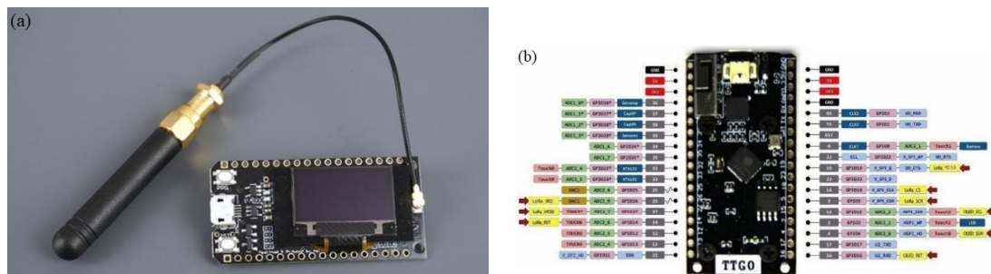
Figure 4. TTGO LoRa32 SX1276 OLED ESP32 board. (a) Board picture. (b) Board Pin-out
