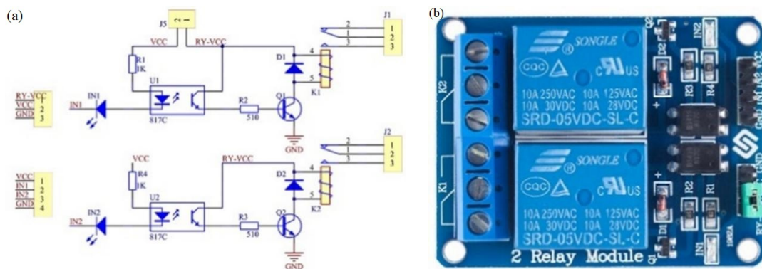
Figure 8. 2-Channel 5V relay module. (a) Schematic diagram. (b) Sensor picture
