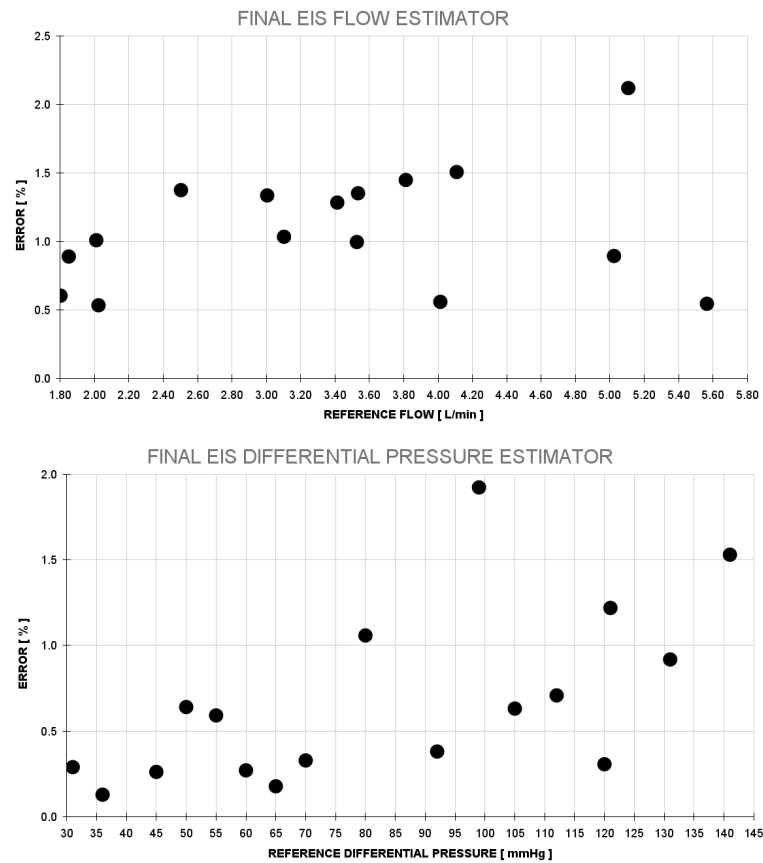
Figure 6. Graph depicting the error relationship between measured data and the reference value for IES with the last version of the flow and differential pressure estimator
