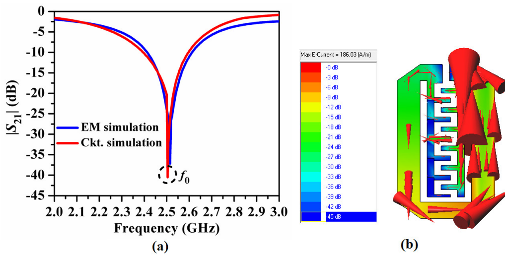
Figure 5. (a) Comparison of the EM and circuit simulated |S_{21}| (dB) of the unit CCDFHL cell, (b) surface current vectors distribution plot for a CCDFHL cell at f_0 = 2.5 GHz.
