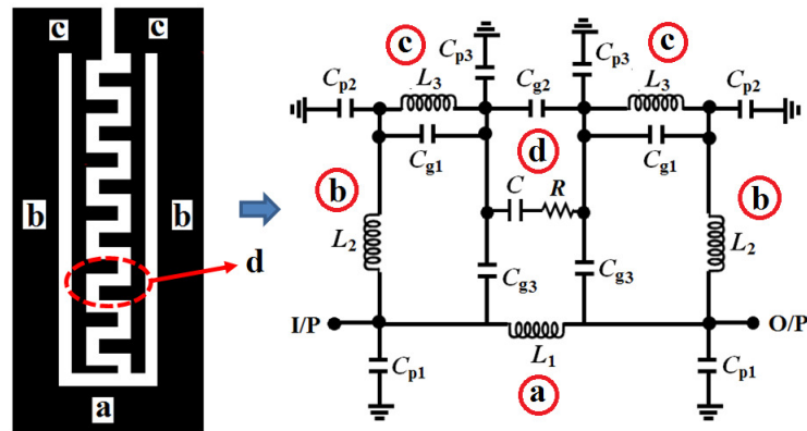
Figure 4. Equivalent circuit diagram of the unit CCDFHL cell in lumped elements.
