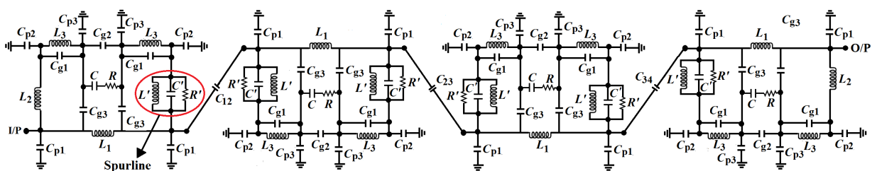
Figure 25. Equivalent circuit of the fourth-order CCDFHL cells based bandpass filter with meander spurline in lumped elements.
