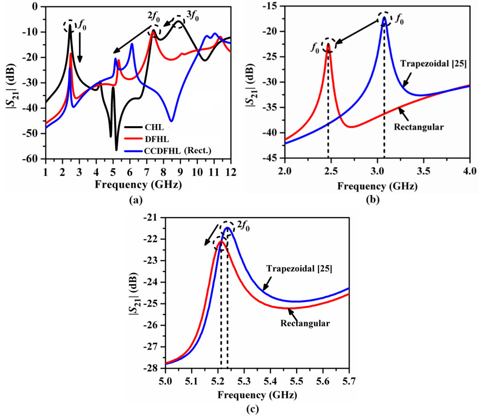
Figure 2. (a) Comparison of |S_{21}| (dB) of the rectangular shaped CCDFHL cell with the CHL and DFHL cells, (b) comparison of |S_{21}| (dB) for the center frequency ( f_0 ), and (c) the second harmonic frequency ( 2f_0 ) between the proposed rectangular shaped and trapezoidal shaped CCDFHL cells [25].
