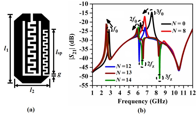
Figure 16. CCDFHL unit cell with meander spurline: (a) schematic diagram, (b) broad band resonant properties of |S_{21}| (dB).
