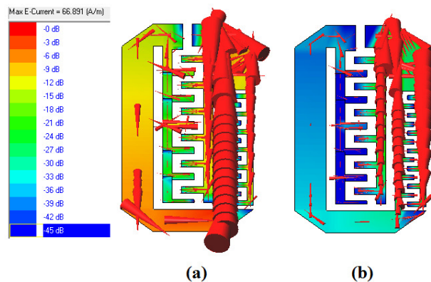
Figure 18. Surface currents for the unit CCDFHL cell with meander spurline at (a) f_0 = 2.23 GHz, (b) 2f_z = 5.38 GHz.
