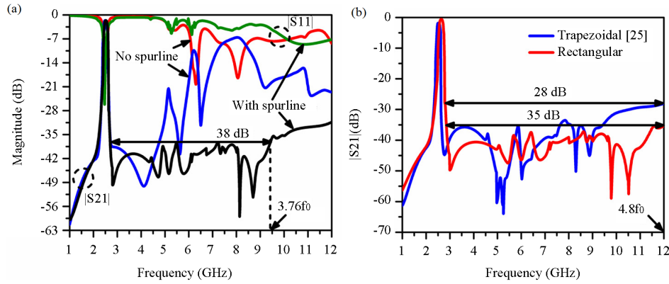
Figure 24. (a) Comparison of S -parameters curves for the fourth-order bandpass filters based on CCDFHL cells for the cases without and with spurline, (b) comparison of |S_{21}| (dB) curves for the fourth-order bandpass filters based on trapezoidal [25] and rectangular CCDFHL cells with spurline
