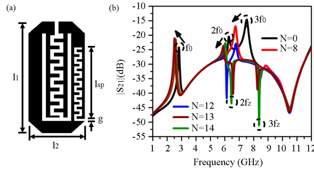
Figure 16. CCDFHL unit cell with meander spurline: (a) schematic diagram, (b) broad band resonant properties of |S_{21}| (dB)
