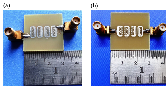
Figure 28. Fourth-order bandpass filter prototypes that were fabricated using CCDFHL cells—(a) without a spurline and (b) with one
