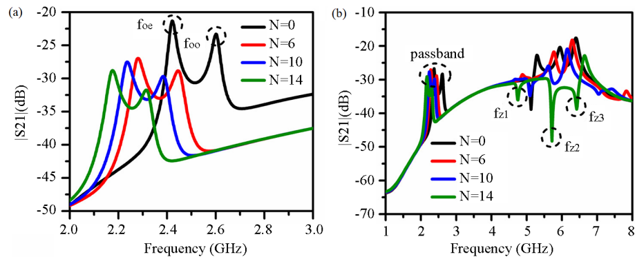
Figure 20. (a) Variation of even- and odd-mode resonant frequencies, (b) comparison of wideband resonant frequency curves for a pair of CCDFHL cells with different values of N
