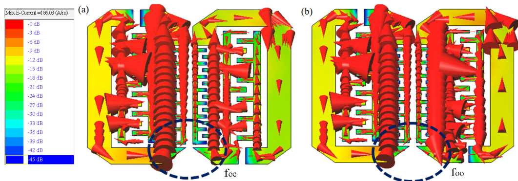
Figure 21. Surface currents for a pair of CCDFHL cells with N = 14 at (a) f_{oe} = 2.17 GHz, (b) f_{oo} = 2.32 GHz
