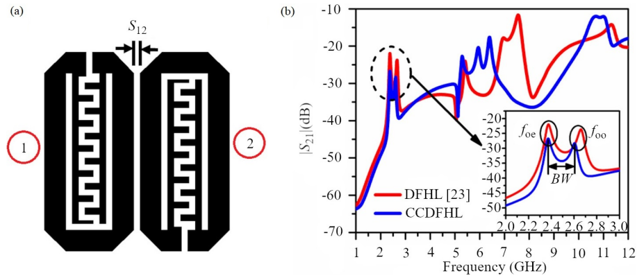
Figure 6. (a) Structure of a pair of CCDFHL cells, (b) comparison of |S_{21}| (dB) between a pair of DFHL cells [23] and CCDFHL cells (passband response is shown in the inset figure)
