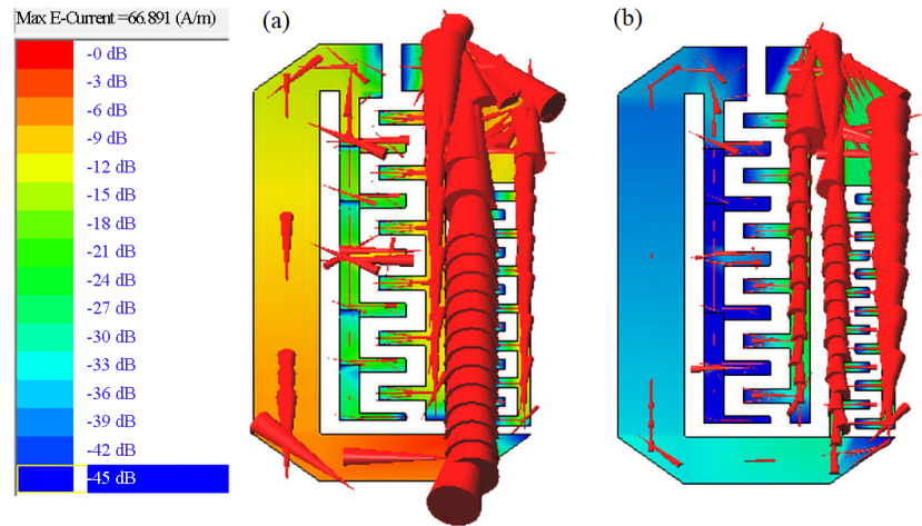
Figure 18. Surface currents for the unit CCDFHL cell with meander spurline at (a) f_0 = 2.23 GHz, (b) 2f_z = 5.38 GHz
