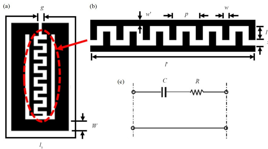
Figure 3. (a) Layout of the unit CCDFHL cell, (b) structure of an interdigital capacitor (IDC), and (c) ideal equivalent circuit diagram of the IDC in lumped elements
