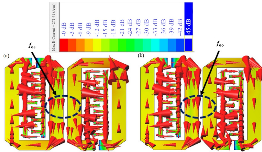
Figure 7. Surface currents of the CCDFHL cells at (a) f_{oe} = 2.38 GHz, and (b) f_{oo} = 2.61 GHz
