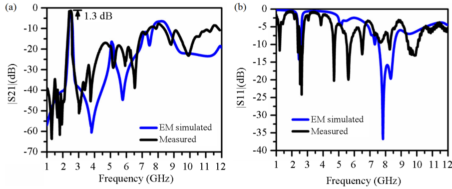
Figure 29. Comparison of the EM simulated and measured S -parameters curves for the fourth-order CCDFHL filter without spurline: (a) |S_{21}| (dB), and (b) |S_{11}| (dB)
