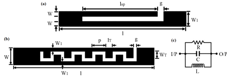
Figure 14. (a) Layout of a quarter-wavelength line with a conventional spurline meander spurline, (b) layout of a quarter-wavelength line with a meander spurline, (c) equivalent circuit diagram
