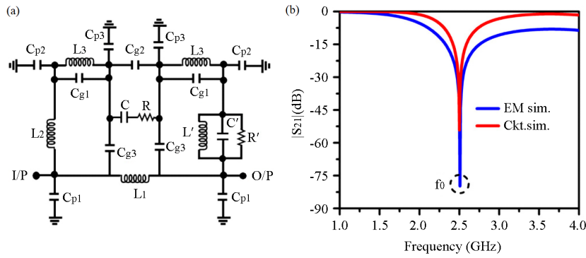
Figure 17. (a) Equivalent circuit schematic for the unit CCDFHL cell featuring a meander spurline; (b) comparison between the curves for |S_{21}| (dB) generated by circuit simulation and EM
