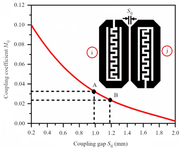
Figure 8. Change in the coupling coefficient M in relation to the coupling gap S (mm) for two CCDFHL cells
