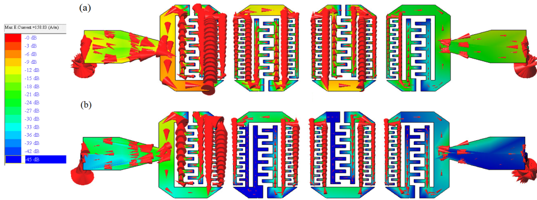
Figure 31. Surface currents for the fourth-order bandpass filter with spurline based CCDFHL cells (a) f_0 = 2.5 GHz, (b) 2f_0 = 5.0 GHz
