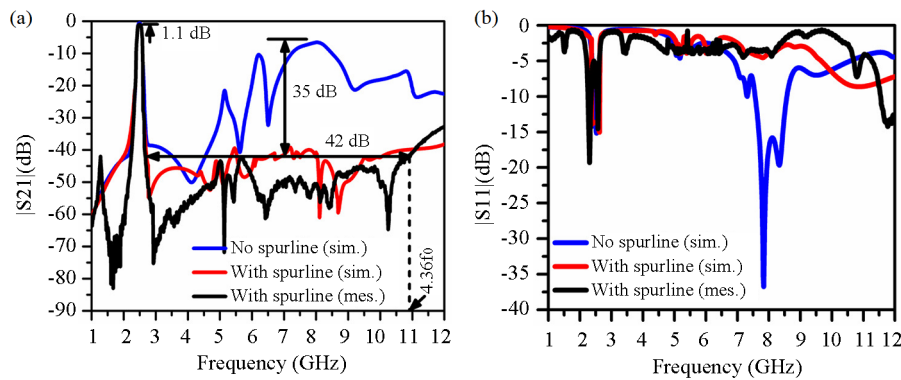
Figure 30. Comparison of the EM simulated and measured S -parameters curves for the fourth-order CCDFHL filter for the cases with and without spurline: (a) |S_{21}| (dB), and (b) |S_{11}| (dB)
