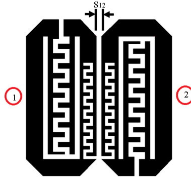
Figure 19. Structure of a pair of CCDFHL cells with meander spurline
