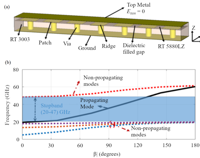
Figure 4. PGW row of unit cell: (a) 3-D view; (b) Dispersion diagram
