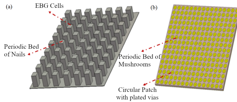
Figure 2. EBG 2-D structures: (a) Metallic bed of nails; (b) Periodic mushroom cells on PCB substrate
