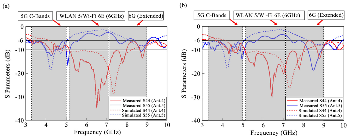
Figure 7. Antenna measured and simulated in 3–10 GHz S-parameter (a) B4 type, (b) B2 type
