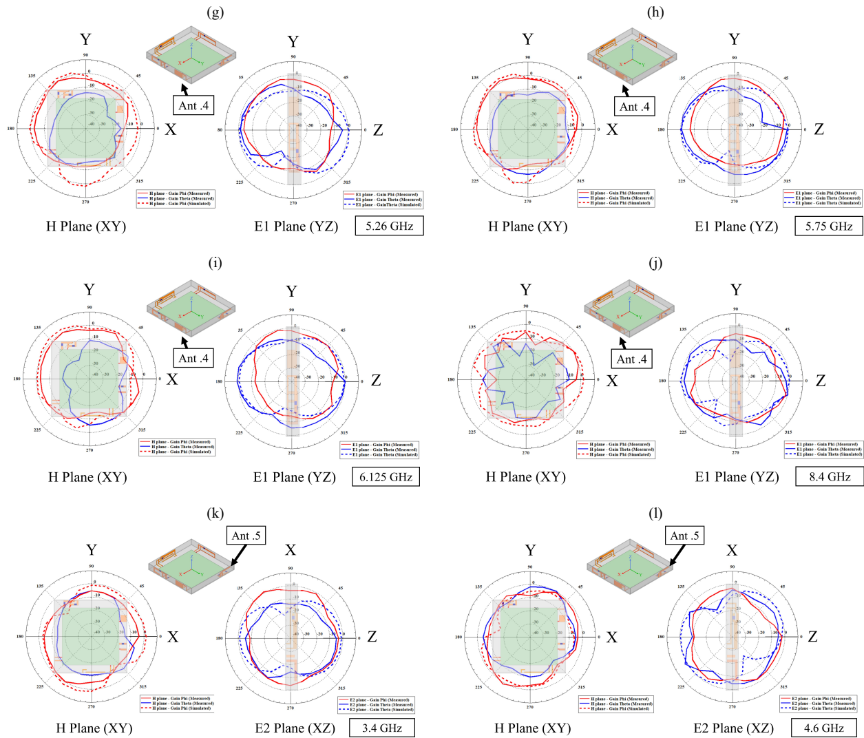
Figure 11. Measured and simulated 2D radiation patterns of antenna (continued)—(g) Ant. 4 testing at 5.26 GHz (resonating by Port 4/B4 type), (h) Ant. 4 testing at 5.75 GHz (resonating by Port 4/B4 type), (i) Ant. 4 testing at 6.125 GHz (resonating by Port 4/B4 type), (j) Ant. 4 testing at 8.4 GHz (resonating by Port 4/B4 type), (k) Ant. 5 testing at 3.4 GHz (resonating by Port 5/B4 type), (l) Ant. 5 testing at 4.6 GHz (resonating by Port 5/B4 type)
