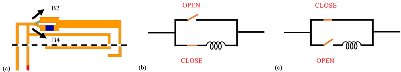
Figure 4. Ant. 2 with different switch types of antenna design and circuit diagrams (a) The antenna element place a switch on the main path, (b) B4 type (B4 Uplink band), (c) B2 type (B2 Bands)
