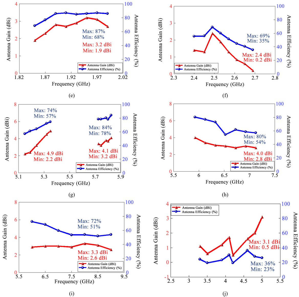
Figure 10. Measured gain and efficiency of antenna (continued)—(e) Ant. 2 testing in 1.85–1.99 GHz (Resonating by Port 2/B2 type), (f) Ant. 3 testing in 2.4–2.69 GHz (Resonating by Port 3/B4 type), (g) Ant. 4 testing in 5.15–5.825 GHz (Resonating by Port 4/B4 type), (h) Ant. 4 testing in 5.925–7.125 GHz (Resonating by Port 4/B4 type), (i) Ant. 4 testing in 6–9 GHz (Resonating by Port 4/B4 type), (j) Ant. 5 testing in 3.3–5 GHz (Resonating by Port 5/B4 type)
