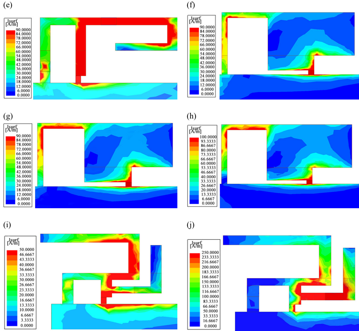
Figure 5. Simulated surface current distribution (continued)—(e) resonating at 2.53 GHz (Port 3/B4 type), (f) resonating at 5.48 GHz (Port 4/B4 type), (g) resonating at 6.52 GHz (Port 4/B4 type), (h) resonating at 8 GHz (Port 4/B4 type), (i) resonating at 3.75 GHz (Port 5/B4 type), (j) resonating at 4.7 GHz (Port 5/B4 type)
