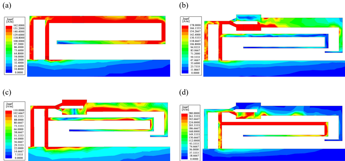
Figure 5. Simulated surface current distribution of antenna elements (a) resonating at 1.575 GHz (Port 1/B4 type), (b) resonating at 1.73 GHz (Port 2/B4 type), (c) resonating at 1.92 GHz (Port 2/B2 type), (d) resonating at 2.13 GHz (Port 2/B4 type)
