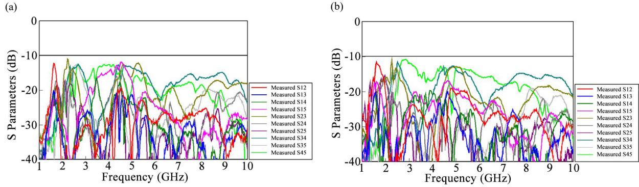
Figure 8. Antenna measured in 1–10 GHz isolation S-parameters (a) B4 type, (b) B2 type
