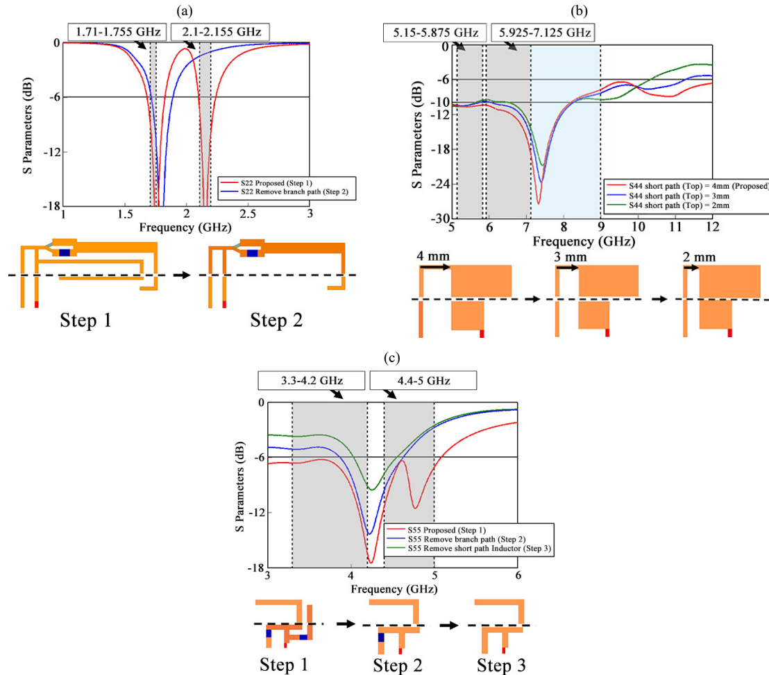
Figure 9. Step-wise design of antenna elements (a) Ant. 2 Step-wise chart (B4 type), (b) Ant. 4 Step-wise chart, (c) Ant. 5 Step-wise chart
