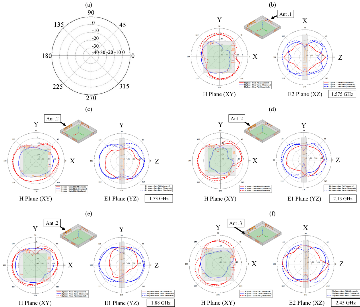
Figure 11. Measured and simulated 2D radiation patterns of antenna (a) angle and Scale of 2D radiation fields, (b) Ant. 1 testing at 1.575 GHz (resonating by Port 1/B4 type), (c) Ant. 2 testing at 1.73 GHz (resonating by Port 2/B4 type), (d) Ant. 2 testing at 2.13 GHz (resonating by Port 2/B4 type), (e) Ant. 2 testing at 1.88 GHz (resonating by Port 2/B2 type), (f) Ant. 3 testing at 2.45 GHz (resonating by Port 3/B4 type)
