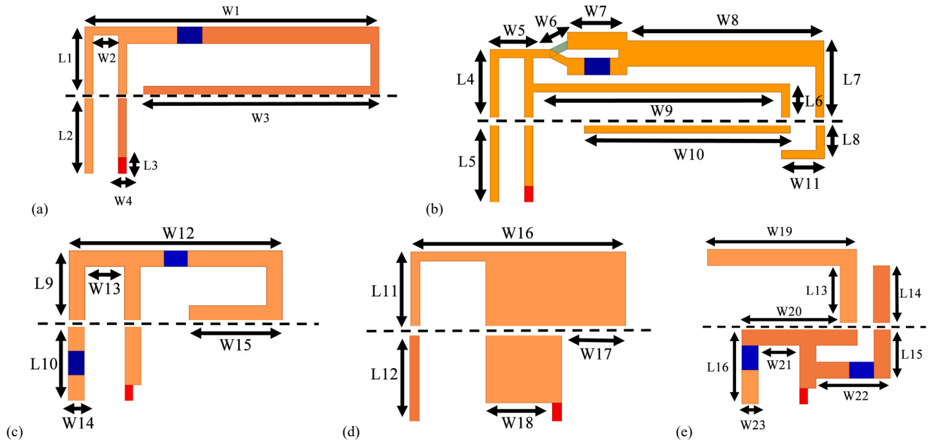
Figure 3. Details of antenna structure (a) Ant. 1, using to resonate GPS band, (b) Ant. 2, using to resonate B2 and B4 bands, (c) Ant. 3, using to resonate n41 and WLAN 2.4 bands, (d) Ant. 4, using to resonate WLAN 5, Wi-Fi 6E (6 GHz) and 6G mid-high extended bands, (e) Ant. 5, using to resonate 5G C-bands
