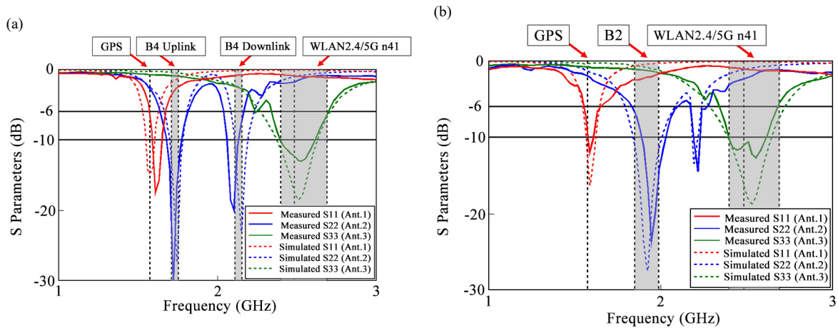
Figure 6. Antenna measured and simulated in 1–3 GHz S-Parameter (a) B4 type, (b) B2 type
