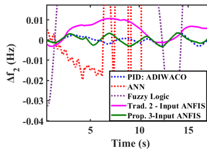
Figure 32. Scenario 3 Area 2 frequency response
