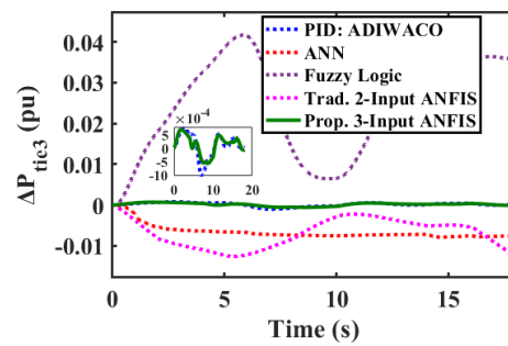
Figure 29. Scenario 2 \Delta P_{(tie\ 3)}
