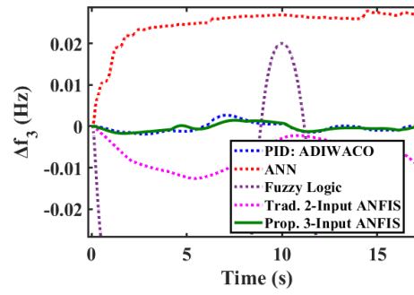
Figure 26. Scenario 2 Area 3 frequency response
