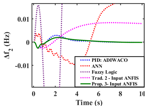
Figure 18. Scenario 1 Area 2 frequency response
