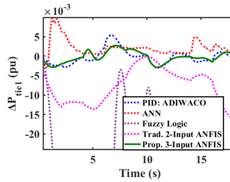
Figure 27. Scenario 2 \Delta P_{(tie\ 1)}
