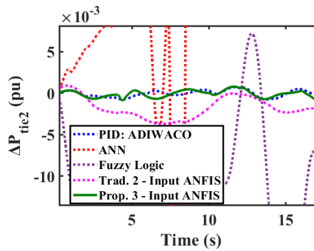
Figure 35. Scenario 3 \Delta P_{(tie\ 2)}
