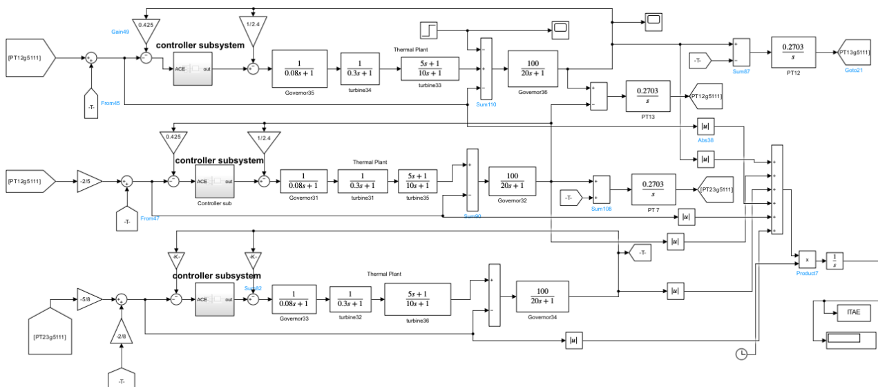
Figure 15. Simulation model of the test system
