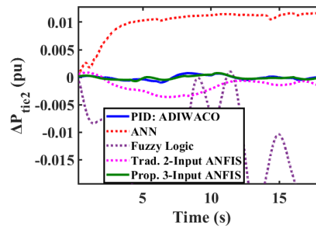
Figure 28. Scenario 2 \Delta P_{(tie\ 2)}
