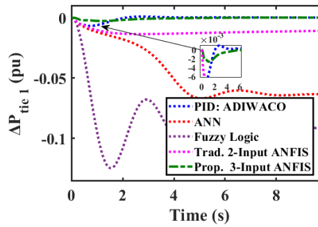
Figure 20. Scenario 1 \Delta P_{(tie\ 1)}
