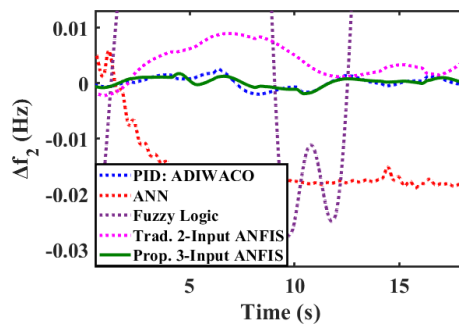
Figure 25. Scenario 2 Area 2 frequency response
