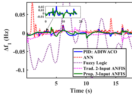
Figure 24. Scenario 2 Area 1 frequency response
