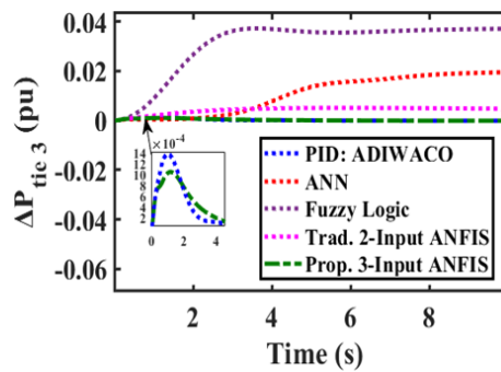
Figure 22. Scenario 1 \Delta P_{(tie\ 3)}
