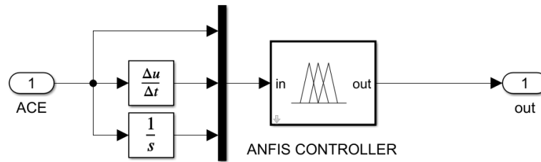
Figure 16. Controller subsystem within the simulation model
