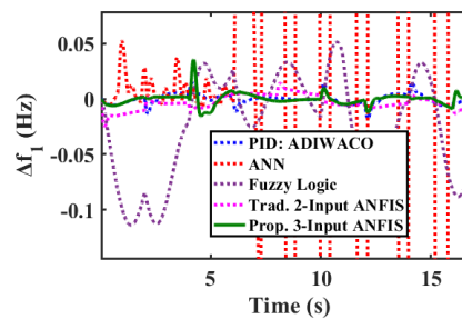
Figure 31. Scenario 3 Area 1 frequency response
