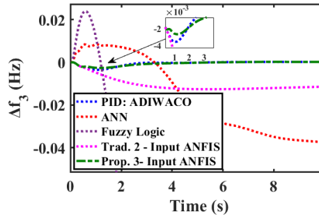
Figure 19. Scenario 1 Area 3 frequency response
