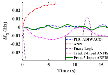
Figure 33. Scenario 3 Area 3 frequency response
