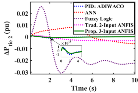
Figure 21. Scenario 1 \Delta P_{(tie\ 2)}
