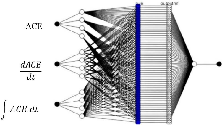
Figure 5. Proposed ANFIS structure showing all 5 layers
