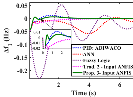
Figure 17. Scenario 1 Area 1 frequency response
