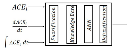
Figure 4. Proposed ANFIS block diagram
