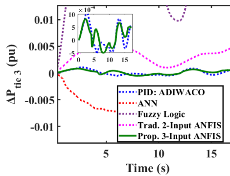
Figure 36. Scenario 3 \Delta P_{(tie\ 3)}
