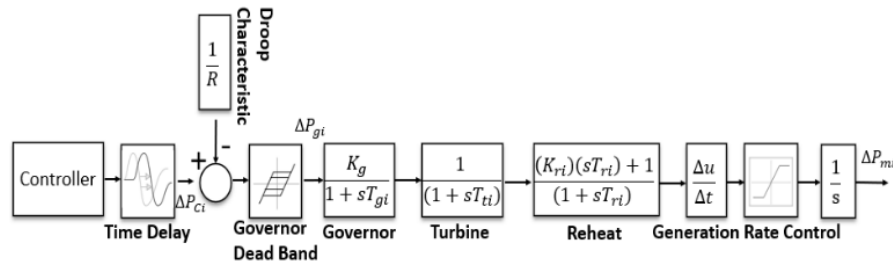
Figure 30. Block diagram representation of constraints
