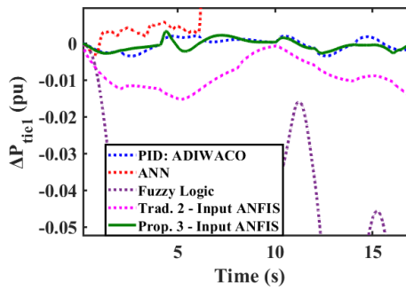
Figure 34. Scenario 3 \Delta P_{(tie\ 1)}
