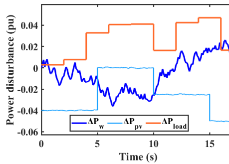
Figure 23. The applied power disturbances
