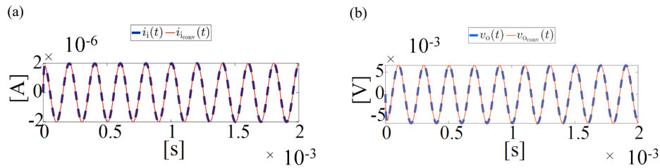
Figure 9. Simulation results, under transients, show the comparison between the input current and the output voltage derived from the model in (10), i.e., (i_i(t), v_o(t)) and those obtained from the inverse conversion of the model in (16) to the model in (10), i.e., (i_{i\text{conv}}(t), v_{o\text{conv}}(t)) . (a) Comparison between i_i(t) , and i_{i\text{conv}}(t) . (b) Comparison between v_o(t) , and v_{o\text{conv}}(t)
