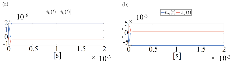
Figure 8. Simulation results, under transients, regarding the dynamic variables from (16). (a) d- and q-channel of i_i(t) . (b) d- and q-channel of v_o(t)
