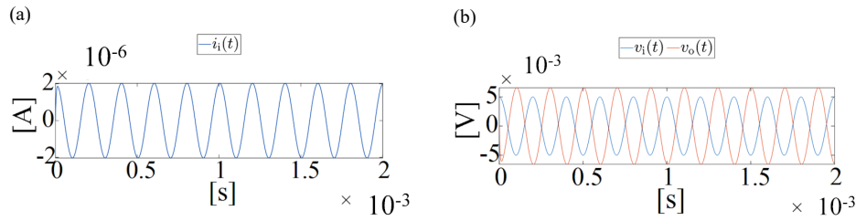
Figure 7. Simulation results, under transients, regarding the dynamic variables from (5). (a) Input current i_i(t) . (b) Input and output voltages v_i(t) and v_o(t)
