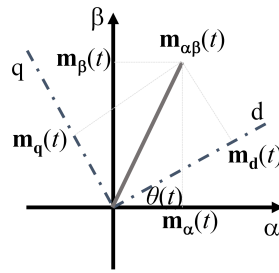
Figure 5. Geometric representation of an arbitrary vector \mathbf{m}_{\alpha\beta}(t) in reference frames \alpha\beta and dq . In addition, the vector components of the vector in its two reference frames are included
