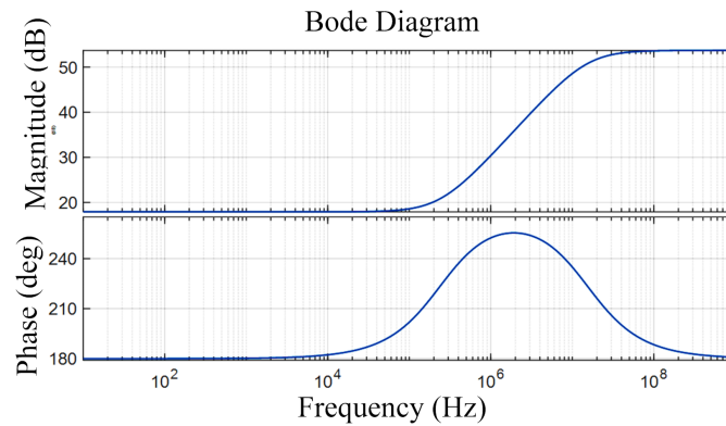
Figure 4. Bode diagram of \mathbf{A}_v(j \cdot \omega) . At low frequencies the \mathbf{A}_v(j \cdot \omega) \approx 18 dB and phase reach 180°. At high frequencies, the \mathbf{A}_v(j \cdot \omega) \approx 54 dB
