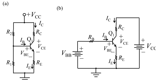
Figure 2. CEA operating in dc regime. (a) Topology in dc bias. The capacitors C_B and C_C act as open circuits. (b) Topology in dc bias with equivalent Thévenin input network
