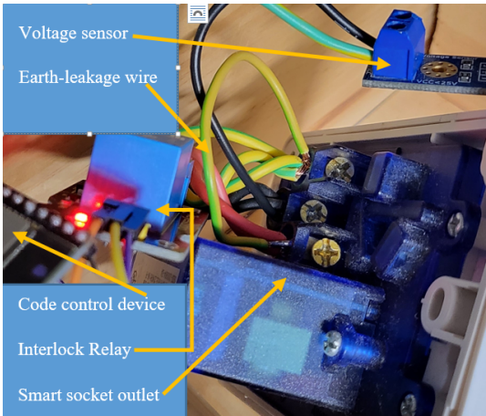
Figure 10. Smart socket out voltage interlocking method
