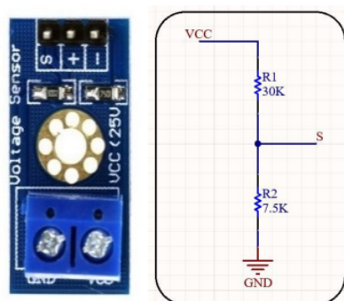
Figure 4. Modul F031-06—voltage sensor (0–25 V) [29]
