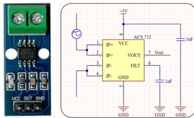
Figure 3. Modul ACS712—current sensor (5 A) [28]
