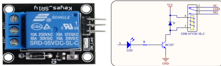
Figure 5. The SRD-05VDC-SL-C relay module [31]
