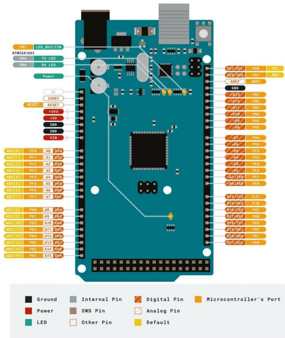
Figure 2. Pinout diagram of mega 2560 [26]
