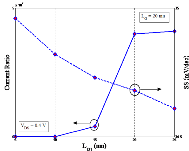
Figure 13. Current ratio diagram and sub-threshold swing versus the length of L_{D1} in V_{DS} = 0.4 V
