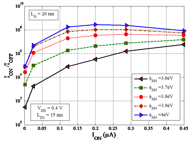
Figure 11. The ON/OFF current ratio versus ON current by changing the \phi_{M4} in the proposed structure at V_{DS} = 0.4 V
