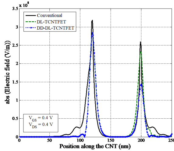
Figure 7. Electric field versus position along the CNT at V_{DS} = 0.4 V and V_{GS} = 0.4 V
