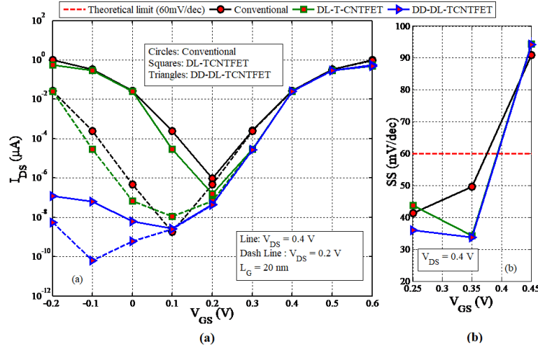
Figure 3. (a) I_{DS} - V_{GS} transfer characteristics diagram in V_{DS} = 0.2, 0.4 V (b) sub-threshold swing versus gate-source voltage in V_{DS} = 0.4 V
