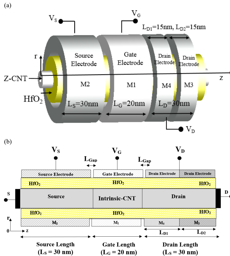
Figure 1. (a) Three-dimensional structure of the proposed design (DD-DL-TCNTFET). (b) Cross-sectional view of the DD-DL-TCNTFET, illustrating the arrangement of components, including the zigzag carbon nanotube, gate dielectric, and the dual work-function drain electrodes
