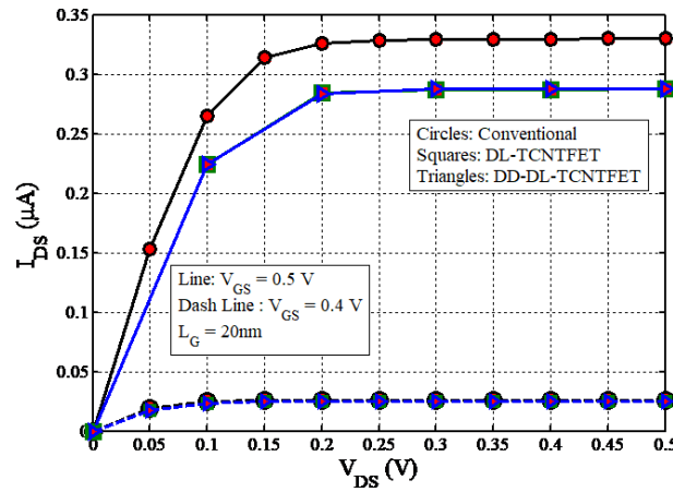
Figure 4. Drain current versus of the drain-source voltage for T-CNTFET, DL-TCNTFET and DD-DL-TCNTFET structures in V_{GS} = 0.4, 0.5 V
