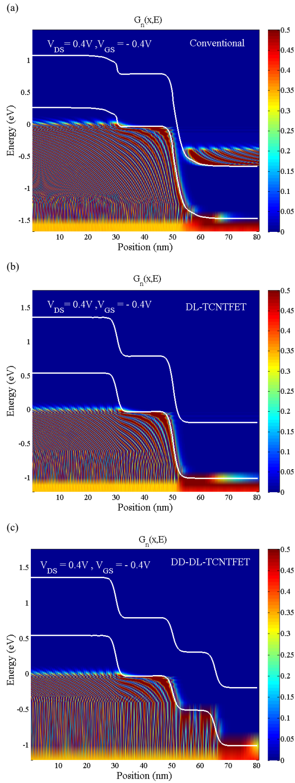
Figure 6. Energy band diagrams versus position along the CNT channel for the structures (a) conventional T-CNTFET (b) DL-TCNTFET and (c) DD-DL-TCNTFET, illustrating the tunneling width between the channel's valence band and the drain's conduction band at V_{DS} = 0.4V and V_{GS} = -0.4V
