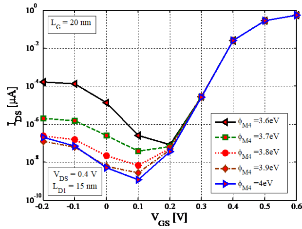
Figure 10. Transfer diagram by changing the \phi_{M4} in the proposed structure at V_{DS} = 0.4 V
