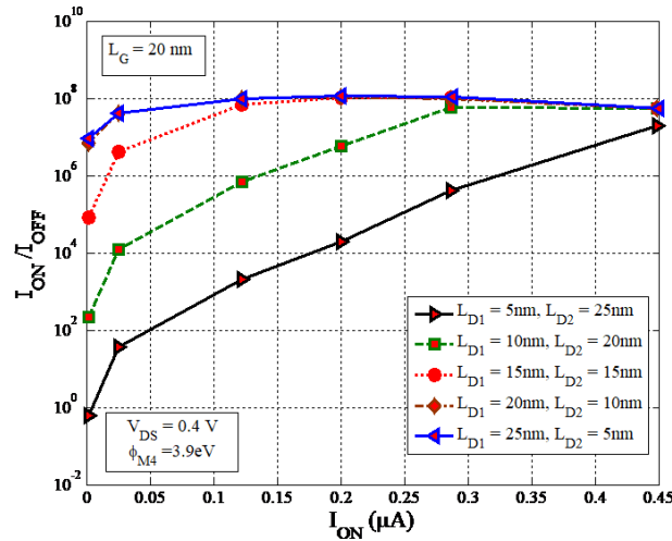
Figure 9. The ON/OFF current ratio versus ON current by changing the length of L_{D1} in the proposed structure at V_{DS} = 0.4 V
