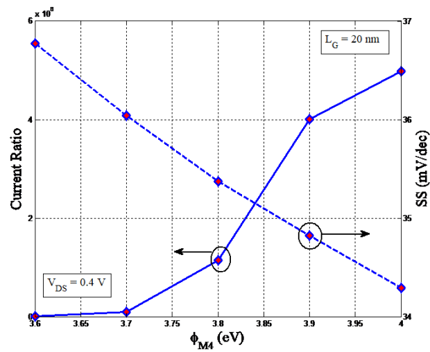
Figure 12. Current ratio diagram and sub-threshold swing versus \phi_{M4} in V_{DS} = 0.4 V
