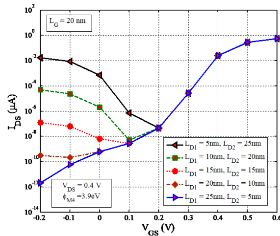
Figure 8. Transfer diagram by changing the length of L_{D1} in the proposed structure at V_{DS} = 0.4 V
