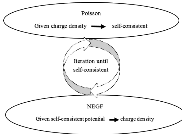
Figure 2. Overview of simulation algorithm and iteration process in NEGF analysis
