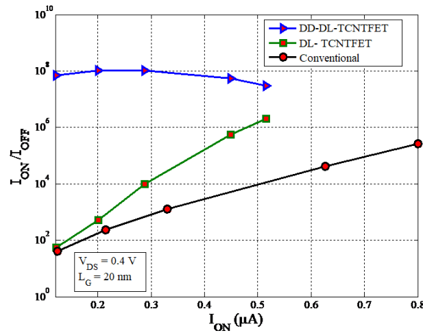
Figure 5. The ON/OFF current ratio curve versus ON current for the DD-DL-TCNTFET, DL-TCNTFET and conventional structures in V_{DS} = 0.4 V
