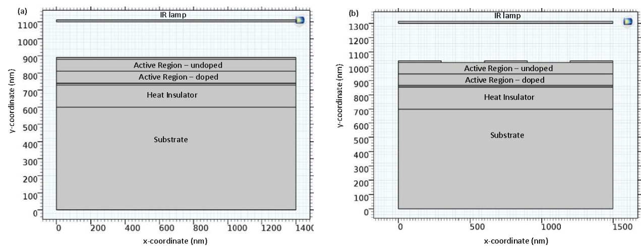
Figure 1. Geometrical structure of the ZnO pyroelectric sensor—(a) fully covered electrode model with active region thickness of 140 nm (b) partially covered electrode model with active region thickness of 160 nm developed using COMSOL with an IR lamp as heat source on top
