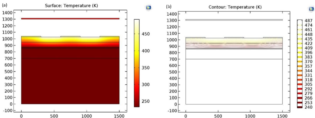
Figure 7. (a) Temperature as measured across the active region of the partially covered top electrode sensor model (b) heat contours for the variation in temperature across the active region
