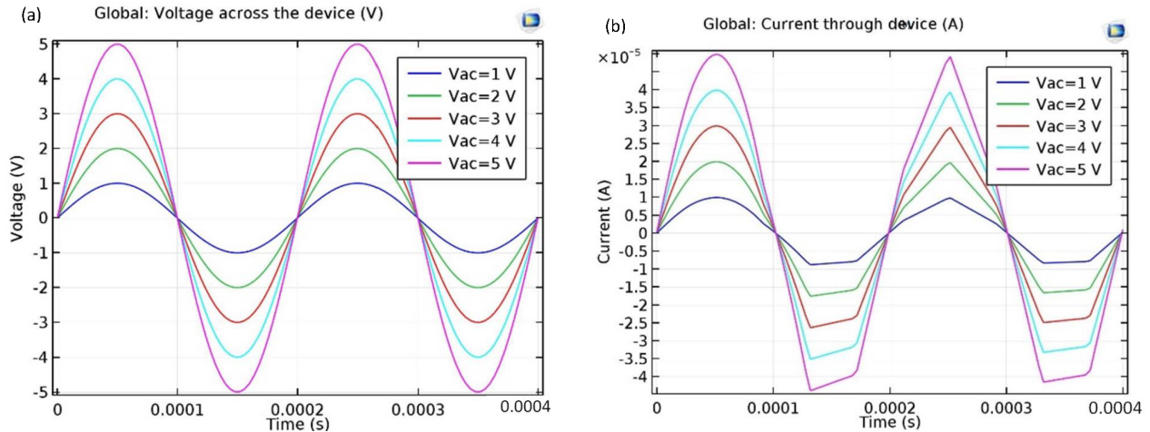
Figure 2. Voltage and Current as measured across the active region sandwiched between the electrodes
