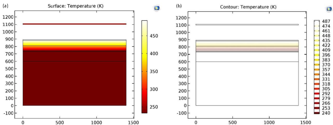
Figure 5. (a) Temperature as measured across the active region of the fully covered top electrode sensor model (b) the heat contours for the variation in temperature across the active region
