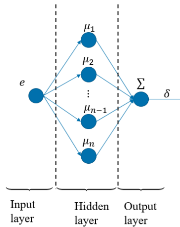
Figure 3. Neural network structure using in this paper
