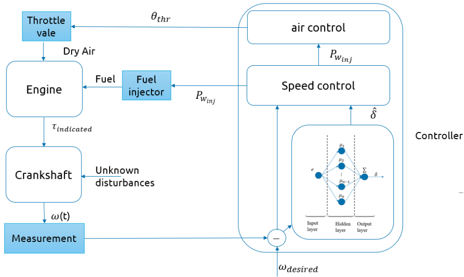
Figure 2. Control structure for controlling the ICE
