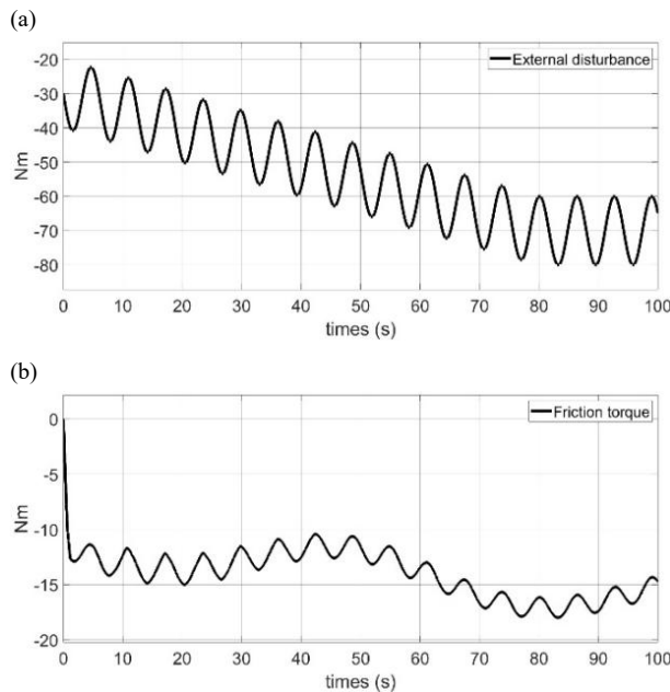
Figure 6. The friction torque (a) and external disturbance torque (b) affected to the system (10) during the simulation
