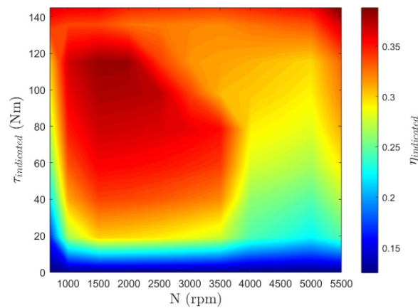
Figure 1. Indicated torque efficiency
