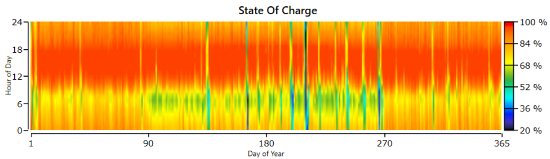
Figure 8. Battery state of charge
