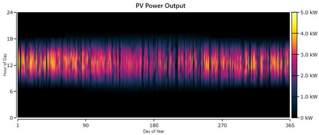
Figure 7. PV power output
