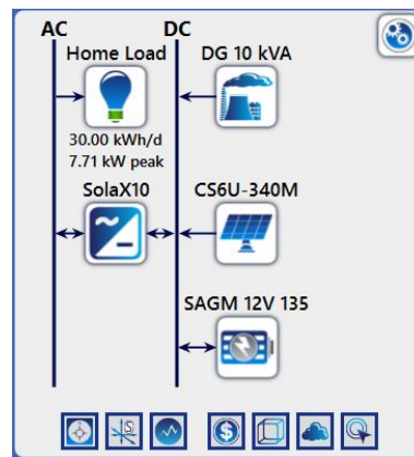
Figure 6. System model for each house
