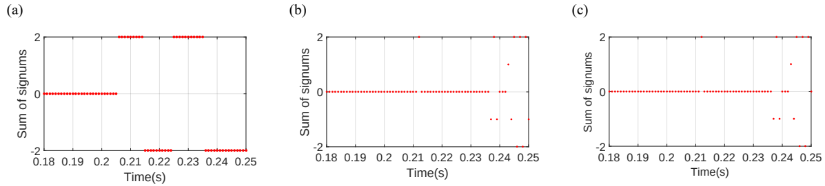
Figure 5. Sum of signums of (a) phase A (b) phase B (c) phase C
