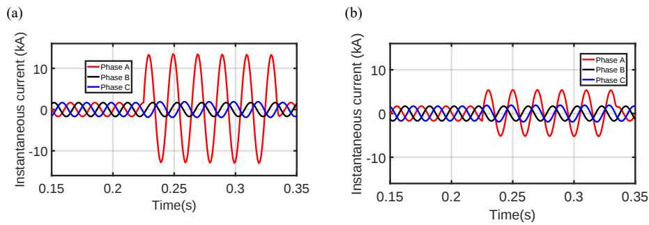
Figure 3. Instantaneous current waveform for phase A, phase B and phase C (a) end 1 (b) end 2
