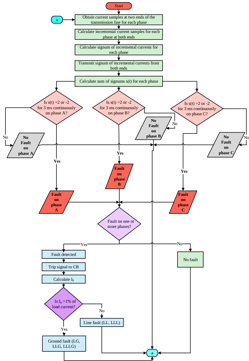
Figure 6. Flowchart for fault detection and classification for line between generator bus and load bus
