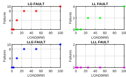
Figure 8. Number of failures reported for L_{GL} using instantaneous power concept [23–25]
