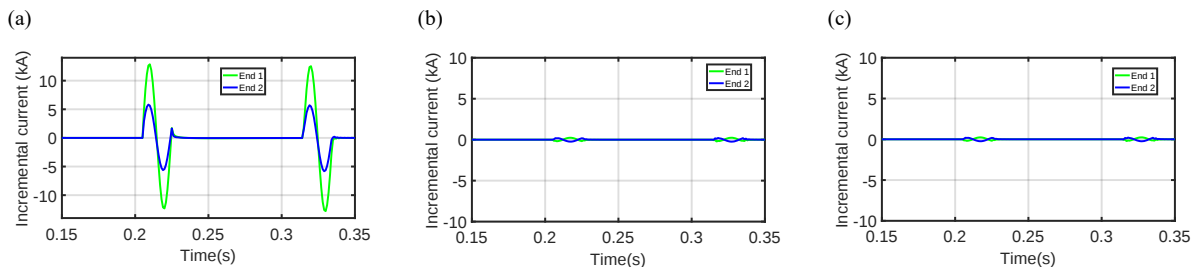
Figure 4. Incremental current of (a) phase A (b) phase B (c) phase C
