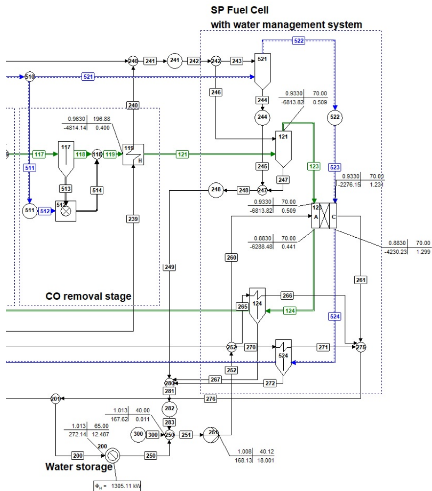
Figure 5. Simulated model of the PEMFC with water management
