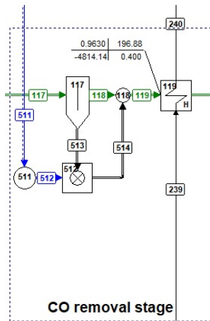
Figure 4. Simulated model of the carbon monoxide removal process
