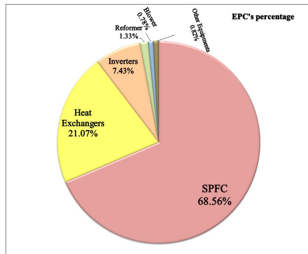
Figure 8. Distribution of equipment purchase costs for the proposed cogeneration system
