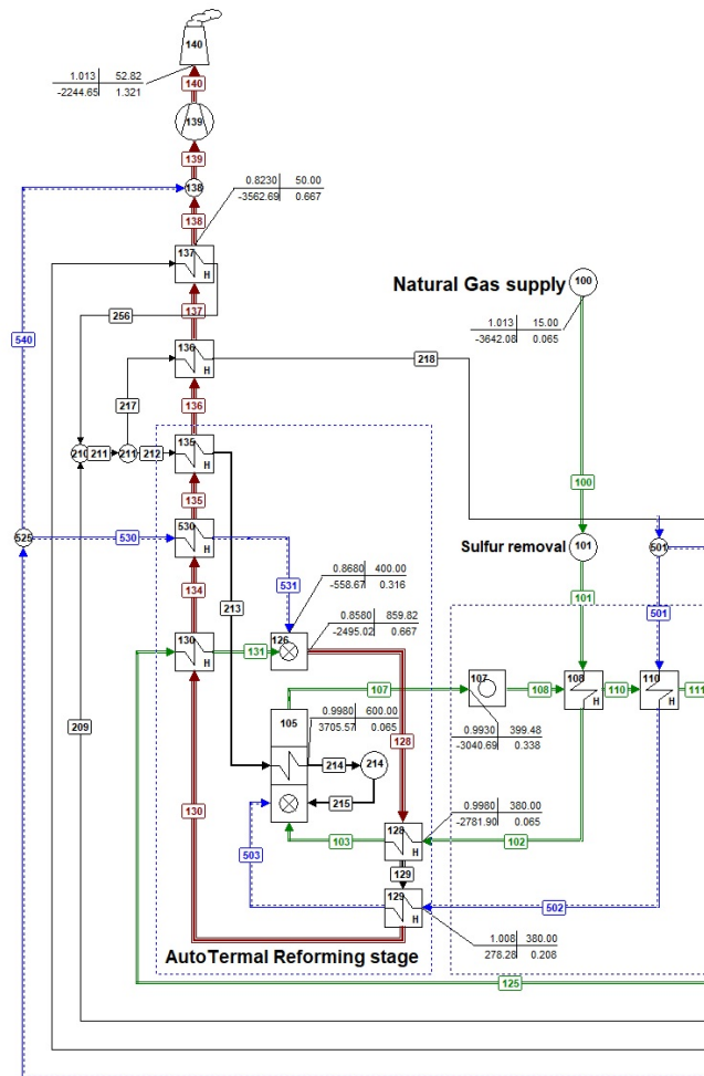
Figure 2. Simulated model of the ATR system for natural gas
