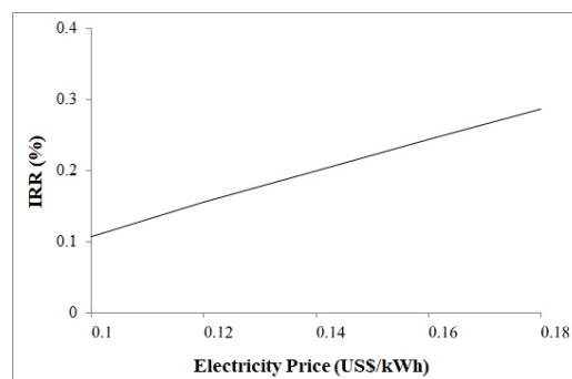
Figure 7. IRR variations for the case studies based on different electricity purchase prices
