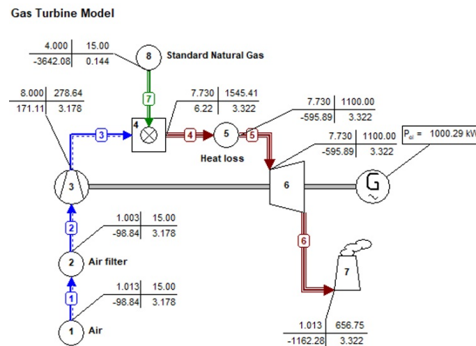
Figure 9. A modelled gas turbine system for comparing fuel consumption and emissions production
