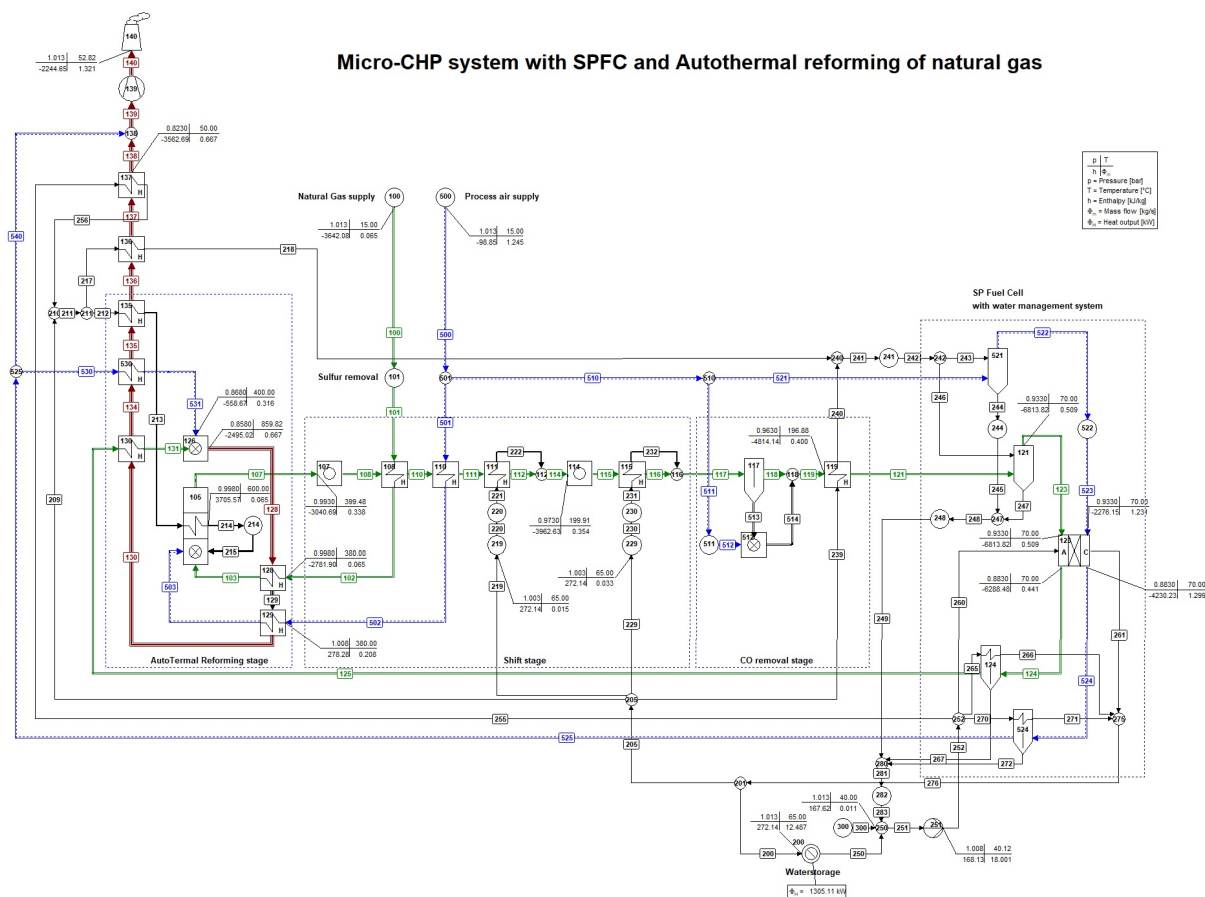
Figure 1. Integrated model simulation of the combined heat and power system utilizing a PEMFC and ATR of natural gas
