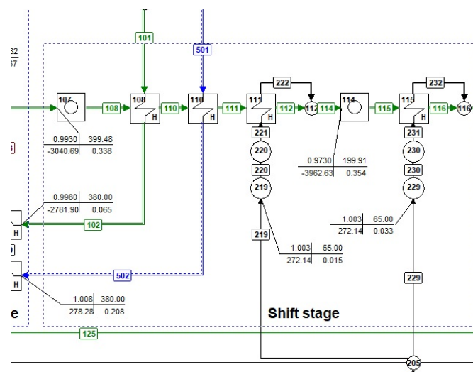
Figure 3. Simulated model of the shift process
