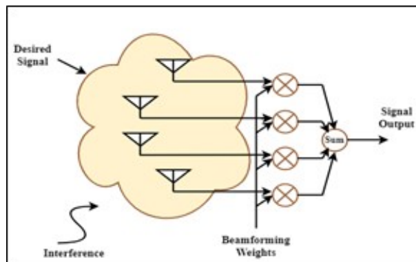
Figure 4. Adaptive array
