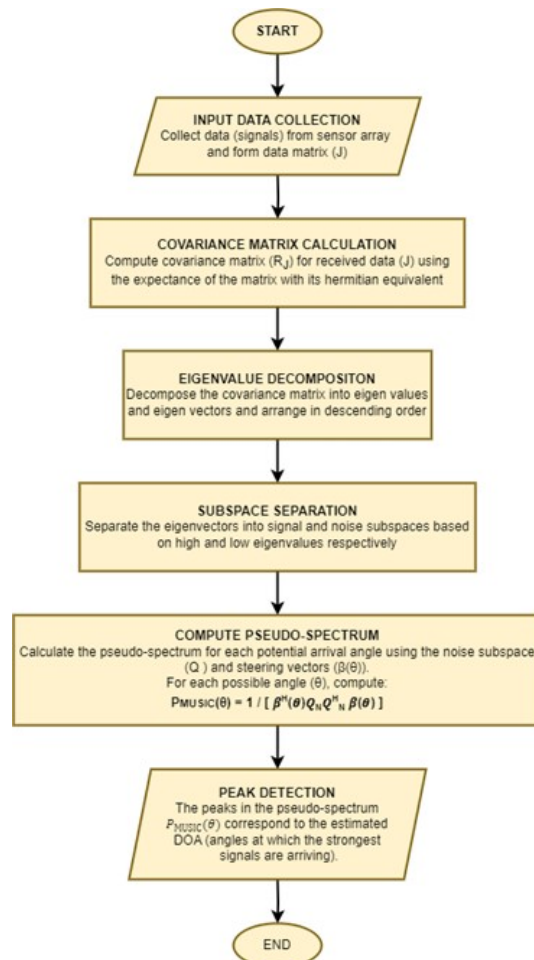
Figure 6. Schematic representation of the MUSIC algorithm
