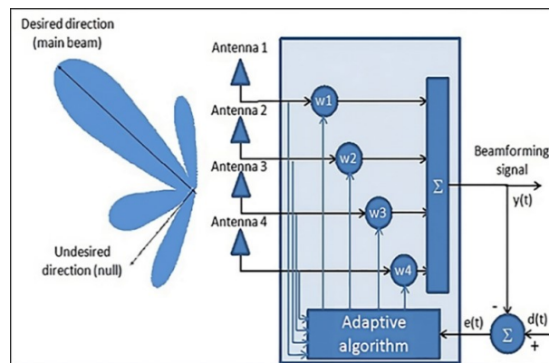
Figure 8. Adaptive beamformer
