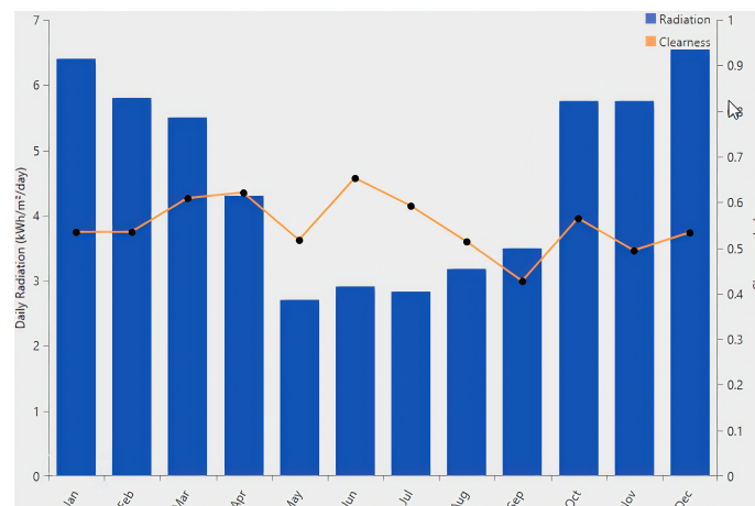
Figure 12. Monthly solar irradiance as inputted for simulation
