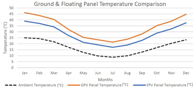
Figure 7. Ground and floating PV panel temperature comparison
