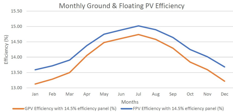
Figure 8. Monthly ground and floating PV panel efficiency given a panel with 14.5% rated efficiency
