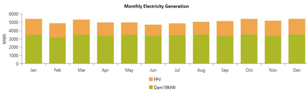
Figure 20. Power output of a HPP & FPV hybrid power station
