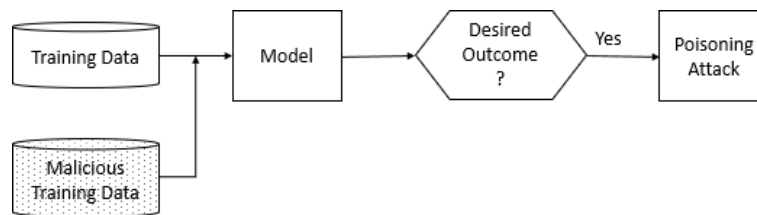
Figure 5. Poisoning attack
