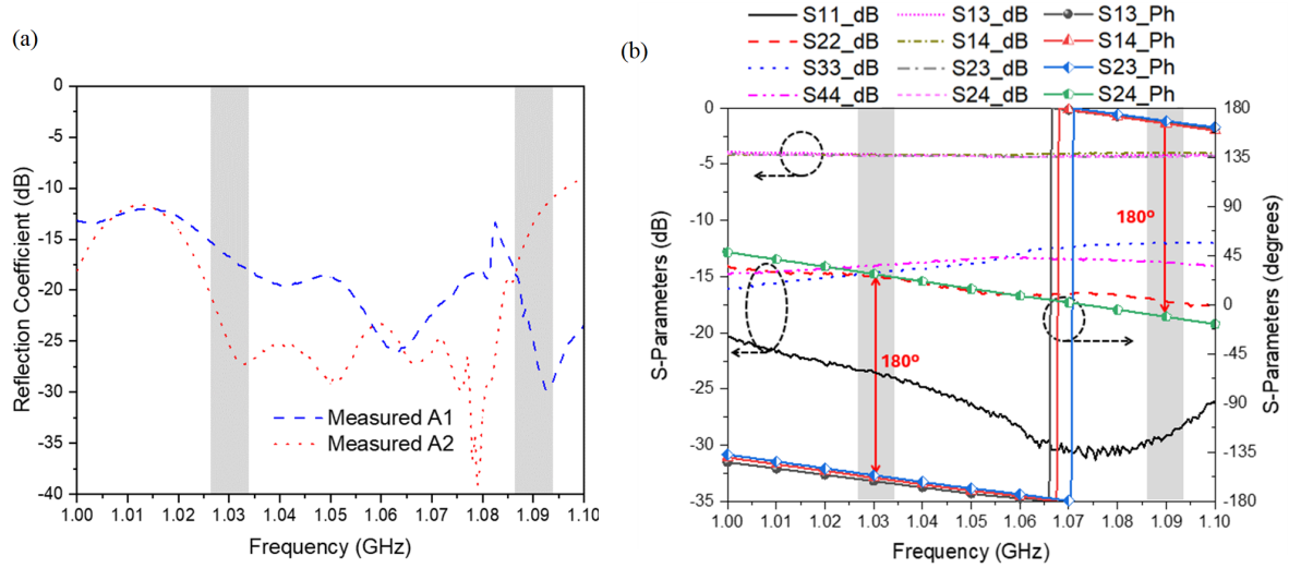
Figure 18. The measured S-parameters of (a) Arrays A1 and A2 (b) control network
