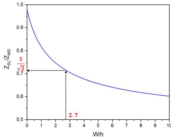
Figure 1. The relation between Z_{SL}/Z_{MS} and w/h
