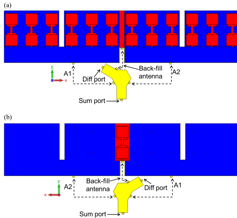
Figure 16. The assembled proposed SSR antenna array (a) front view (b) rear view
