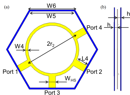
Figure 10. The proposed rat-race (a) front view (b) side view
