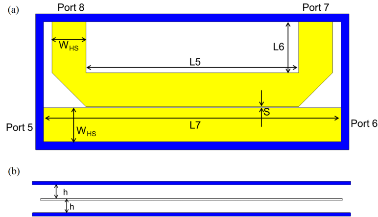
Figure 13. The proposed directional coupler (a) front view (b) side view
