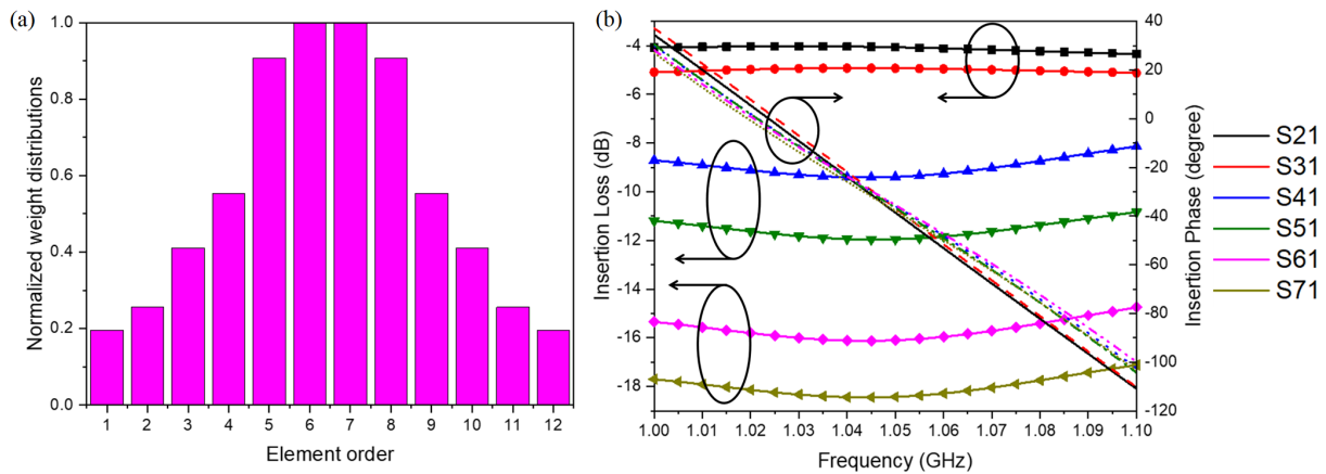
Figure 9. The feeding network (a) weight distributions (b) insertion losses and phases
