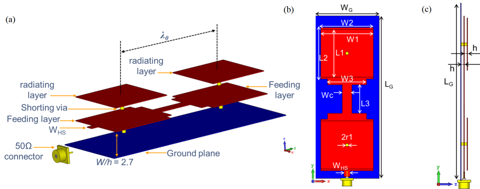
Figure 4. The proposed antenna column (a) exploded geometry (b) front view (c) side view
