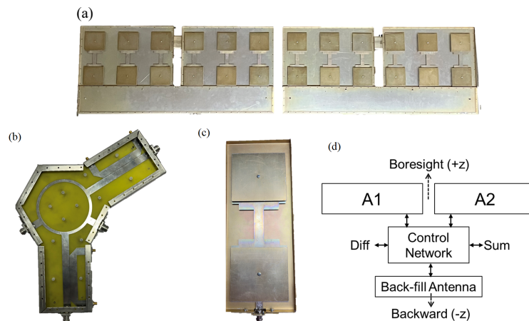
Figure 17. Prototype (a) A1 and A2 (b) the control network (c) the back-fill antenna (d) the assembled block diagram
