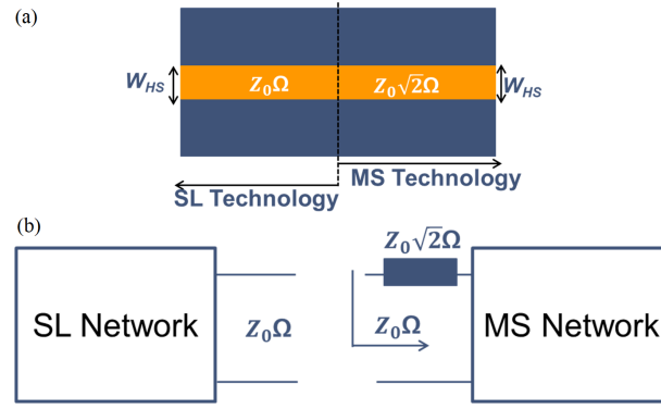
Figure 3. The proposed HS methodology (a) layout (b) matching technique
