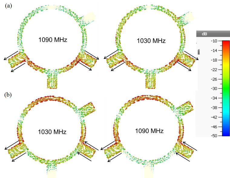
Figure 12. The current distributions across the proposed rat race when it is excited at (a) port 3 and (b) port 4
