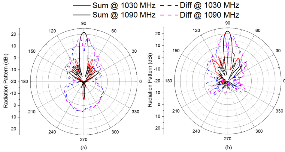
Figure 19. The radiation patterns (a) simulated (b) measured
